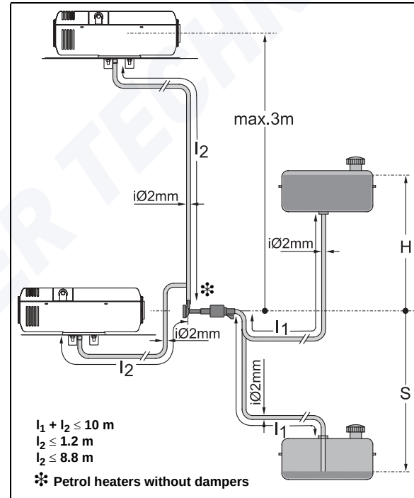
Fig. 9: Fuel supply
