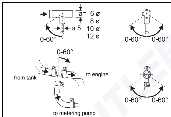
Fig. 10: Webasto fuel extractor
