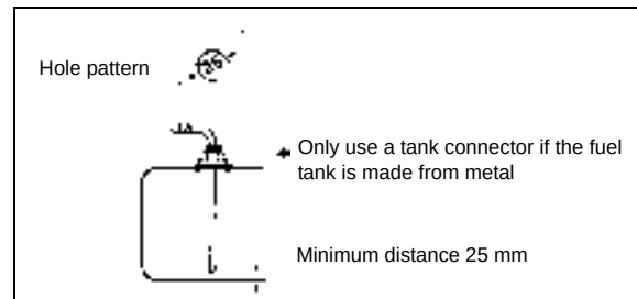
Fig. 11: Webasto tank connector
