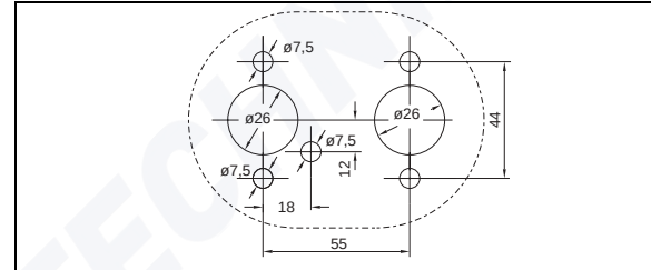
Fig. 3: Hole pattern
