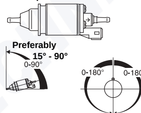
Fig. 15: Metering pump DP 2
