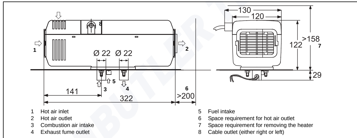
Fig. 1: Dimensions of the heater
