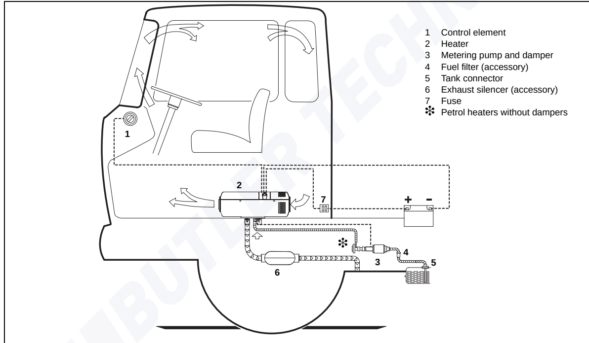
Fig. 7: Installation example for air heater
