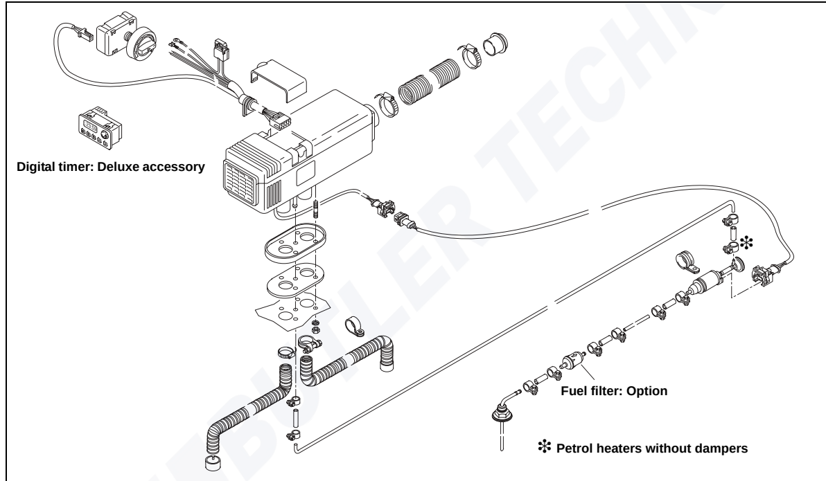
Fig. 6: Installation diagram for air heater
