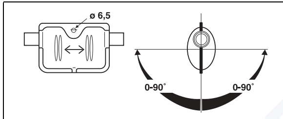
Fig. 18: Exhaust silencer Flow direction (arbitrary)
