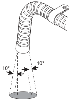
Fig. 22: Exhaust pipe opening Installation position
