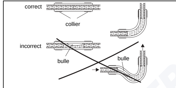
Fig. 14 Raccordement tube-tuyau
