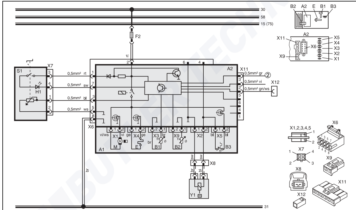
Fig. 30: Automatic circuit diagram for the Air Top 2000, 12V/24V with control element, for legend see pages 70 and 71
