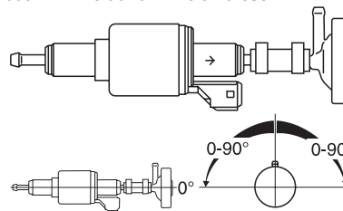
Fig. 16: Metering pump DP 30
