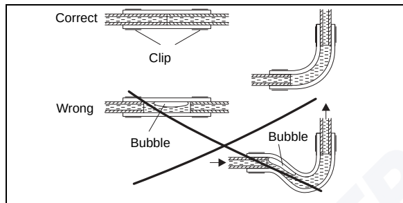
Fig. 14: Pipe / hose connection
