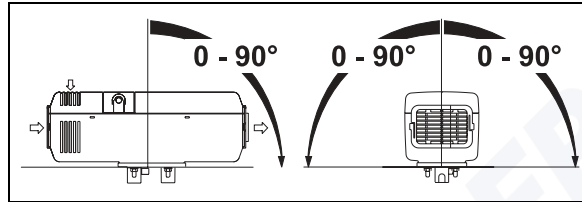
Fig. 2: Recommended installation positions for diesel heaters
