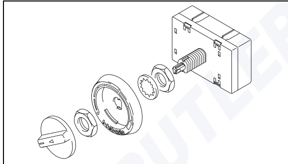
Fig. 26: Control element
