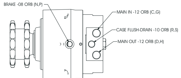
DRIVE MOTOR PORT REFERENCE
