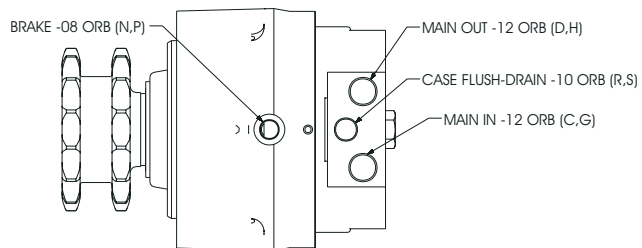
DRIVE MOTOR PORT REFERENCE
