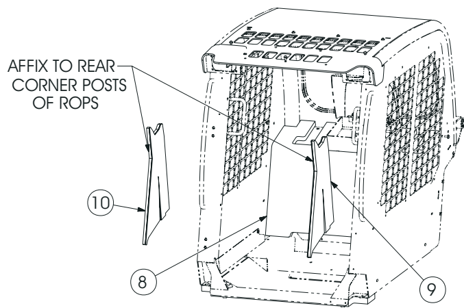
ROPS FRONT VIEW
