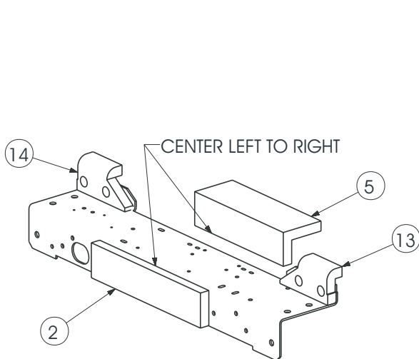
BOLT-IN CROSSMEMBER
