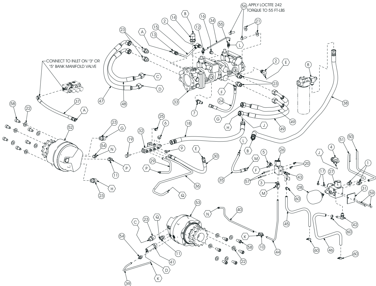
DRIVE MOTOR PORT REFERENCE
