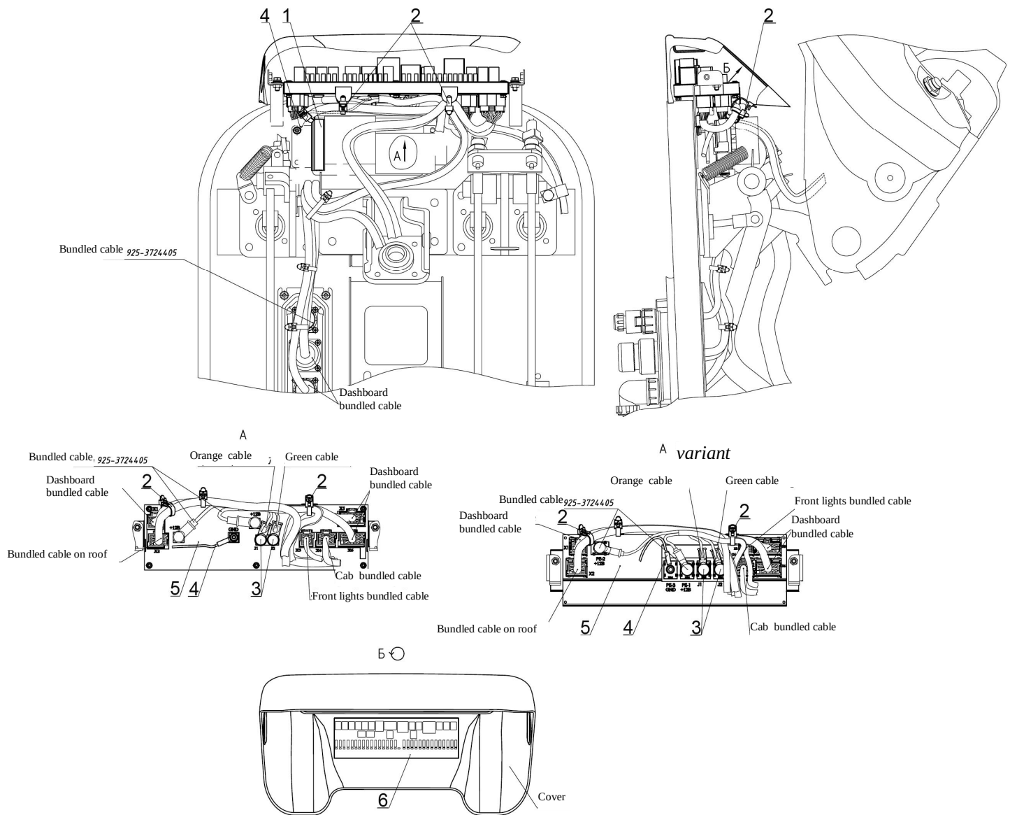
Fig. 37.11 Switching unit
