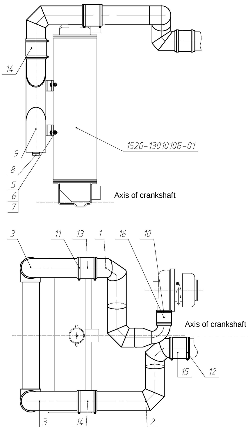
Fig. 13.2 Cooler assembly
