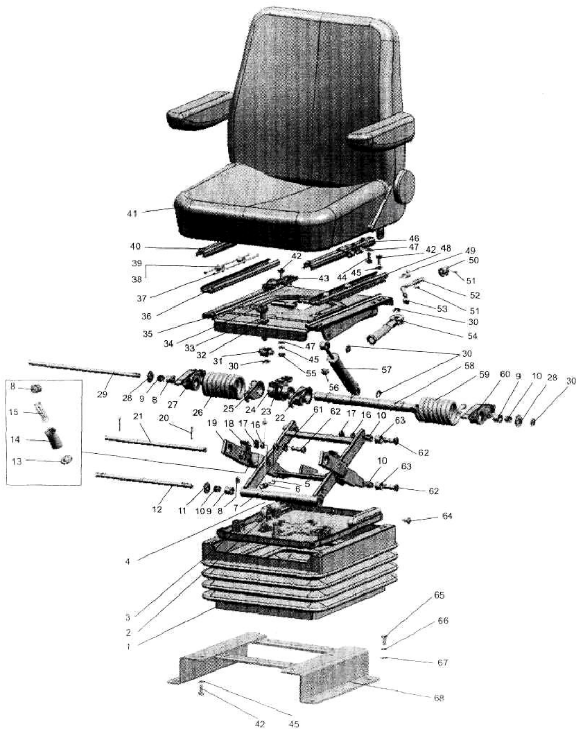
Fig. 68.1 Operator's seat
