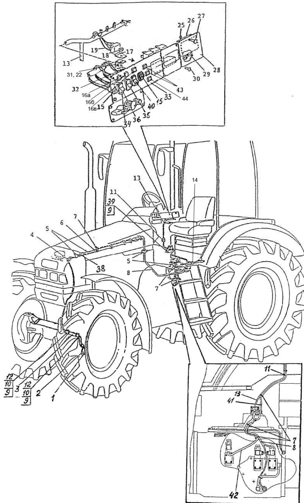
Fig. 87.2 DL, FDA and FPTO control (1523-8700210-D)
