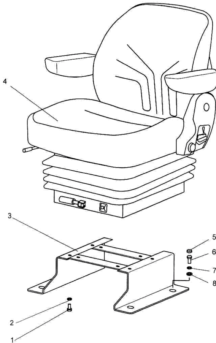
Fig. 68.2 Operator's seat
