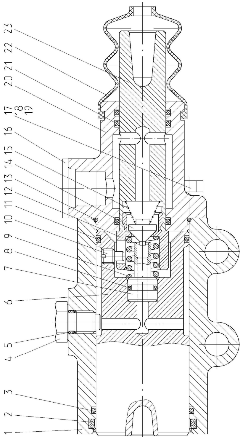
Fig. 16.8 Hydraulic booster
