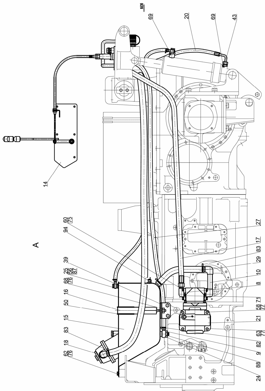
Fig. 46.12 Hydraulic units and fittings
