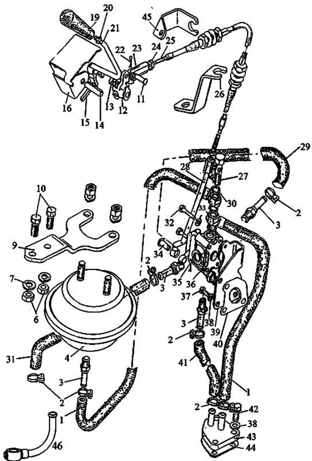
Fig. 42.2 Rear PTO hydraulic drive control
