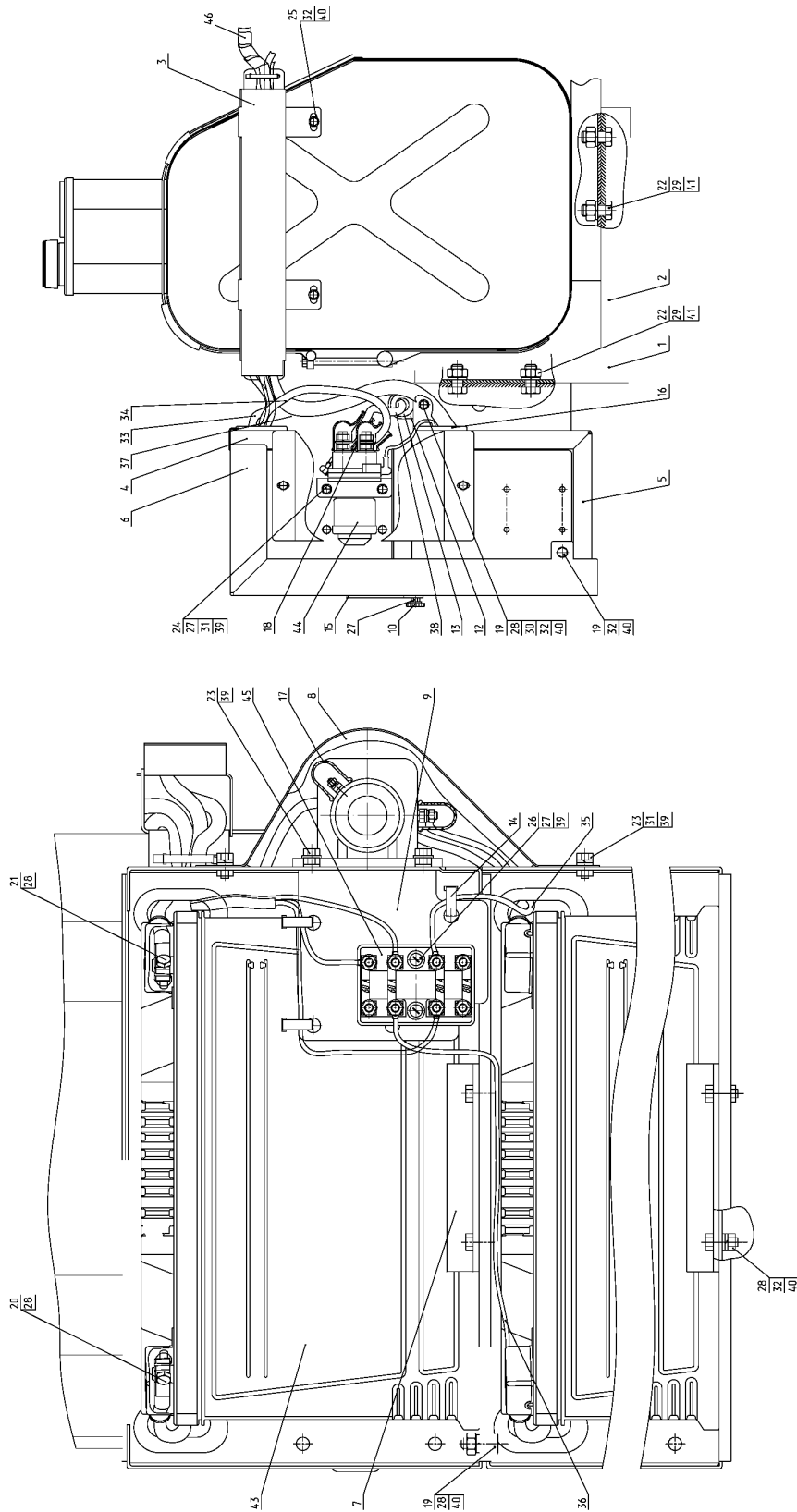
Fig. 37.10 Storage battery assembly
