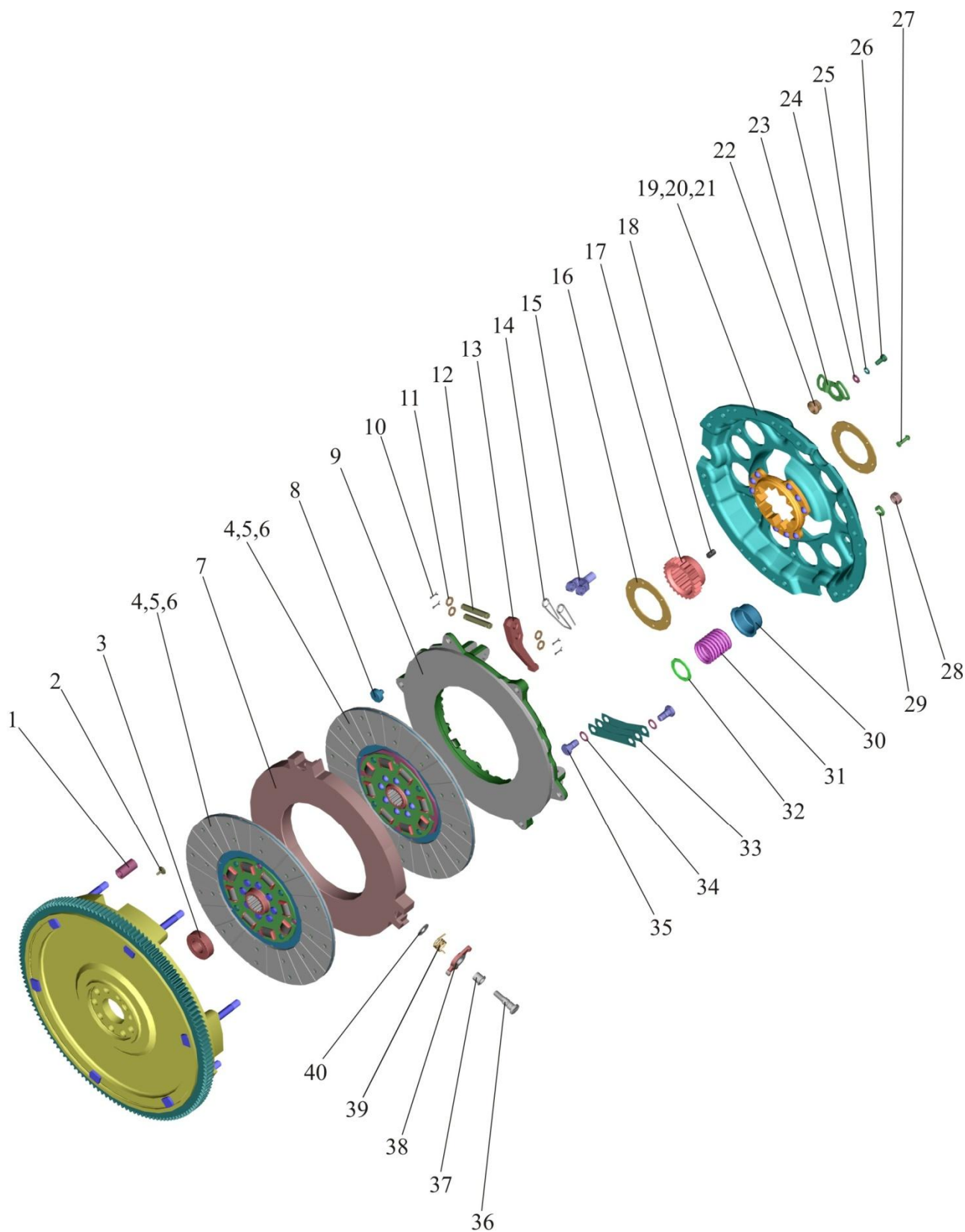
Fig. 16. 1 Clutch assembly
