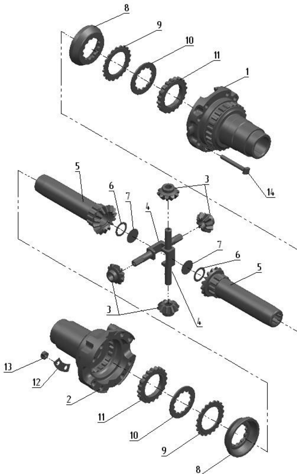
Fig. 23.3 Differential
