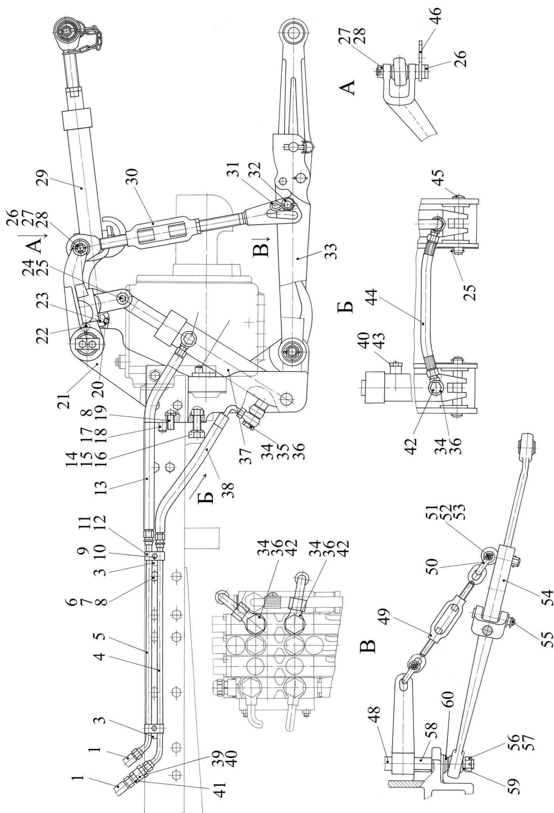
Ris 46.6 Front lift linkage
