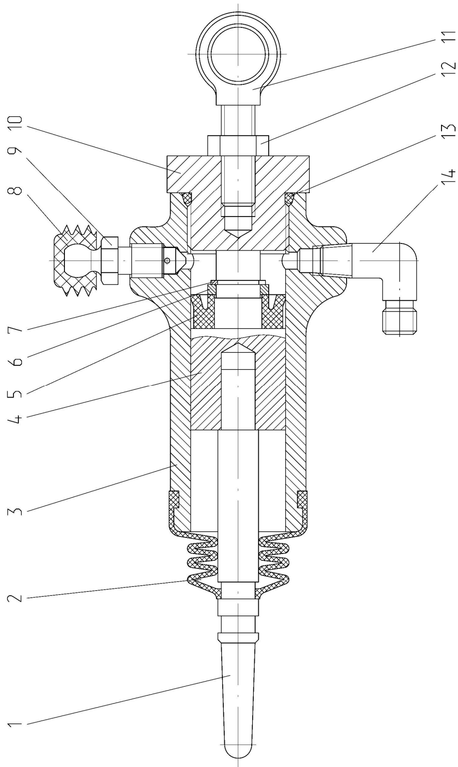
Fig. 16.9 Working cylinder
