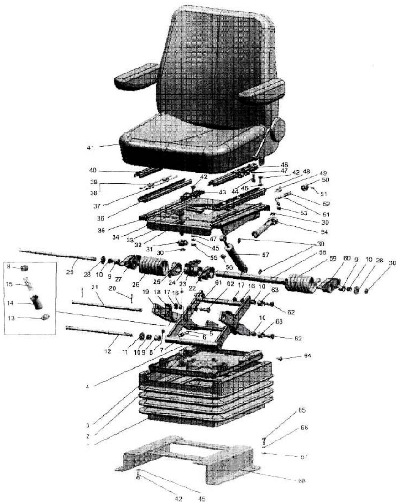
Fig. 68.1 Operator's seat
