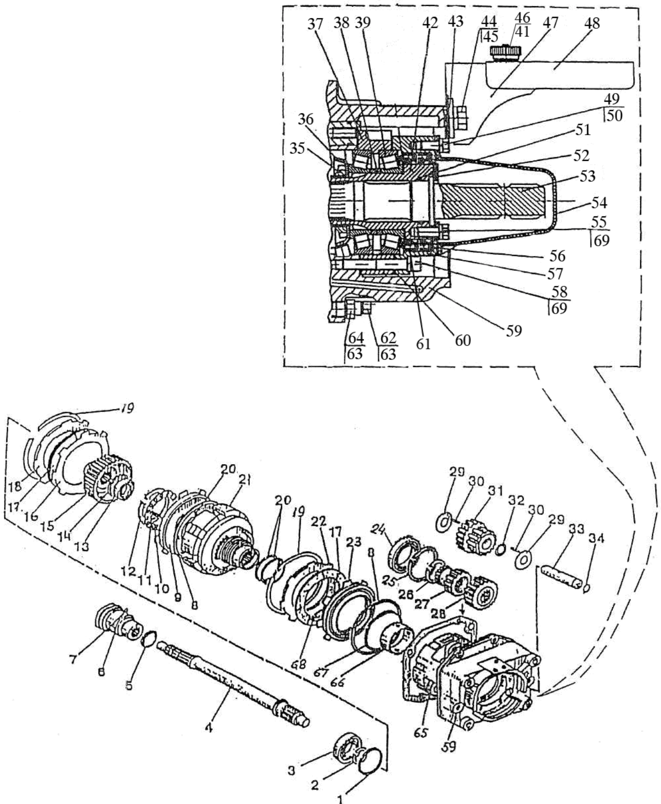
Fig. 42.1 Rear power take-off shaft
