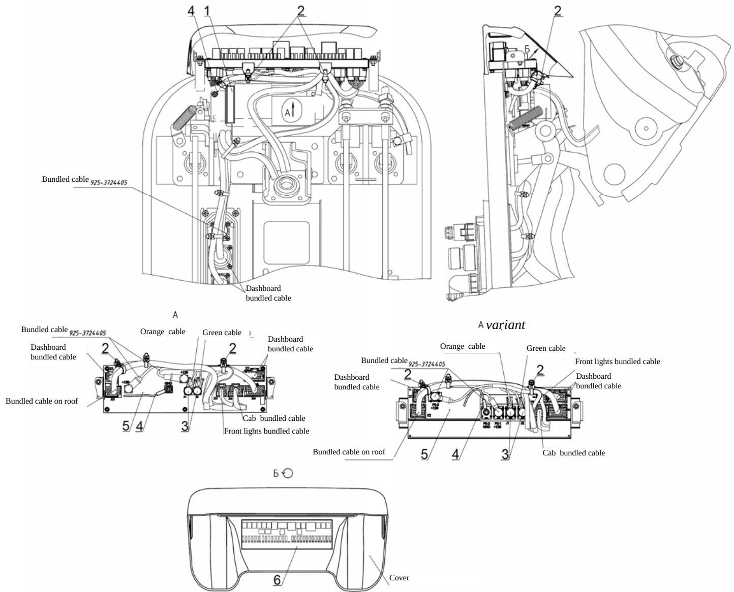
Fig. 37.10 Switching unit
