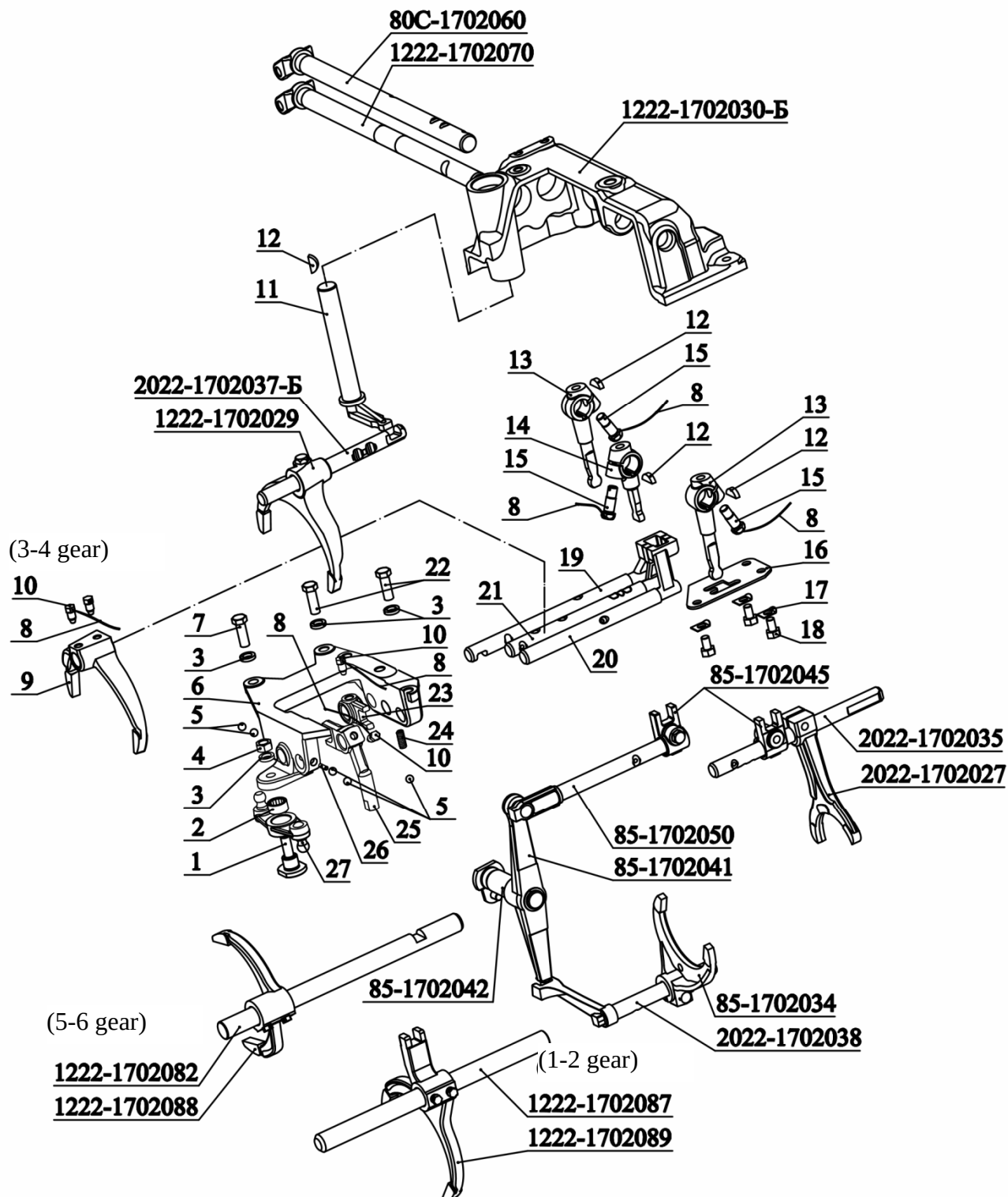
Fig. 17.9 Gearbox control mechanism
