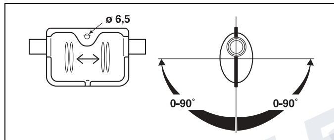
Fig. 18: Exhaust silencer
