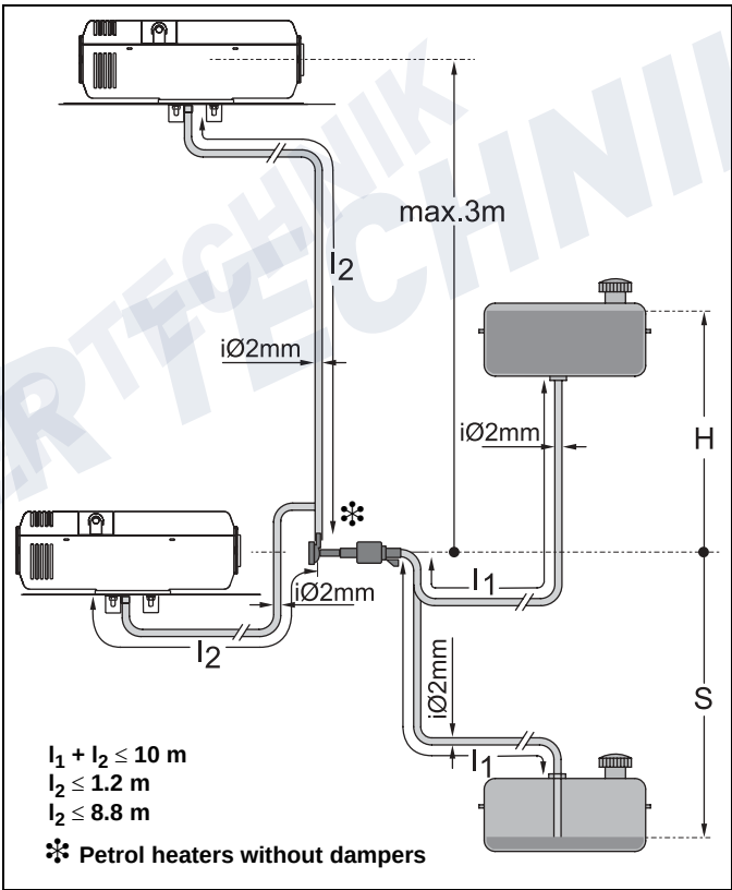
Fig. 9: Fuel supply
