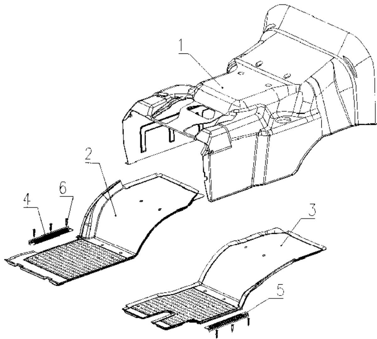
C12-7 ENGINE HOOD, FLOOR LINING FOR STANDARD CAB/标准驾驶室发动机罩、地板 Fig.C12-8
