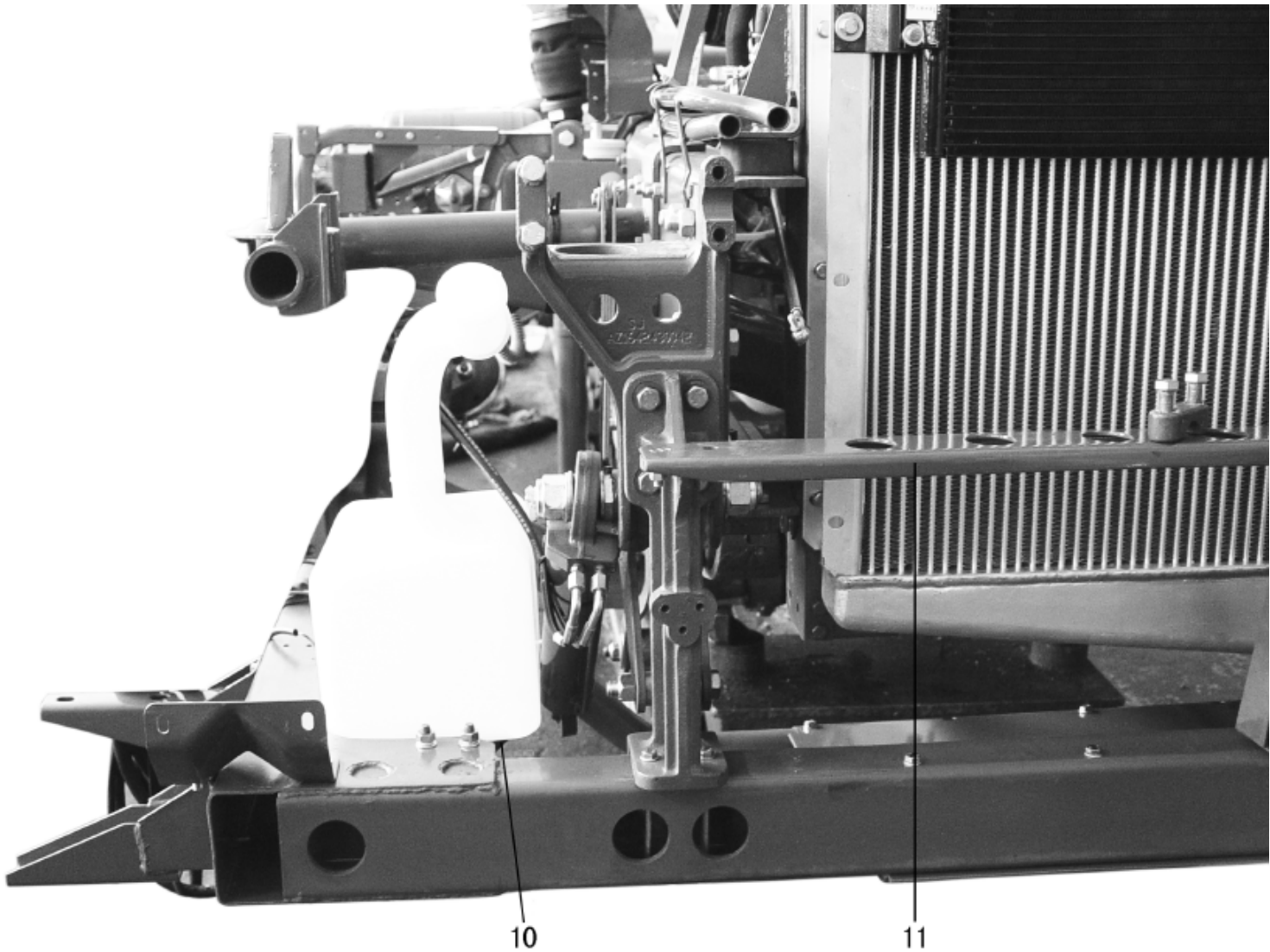
C7-11 BRACKET FOR BUMPER, TOWING HOOK FRONT/保险杠支架，前牵引装置
