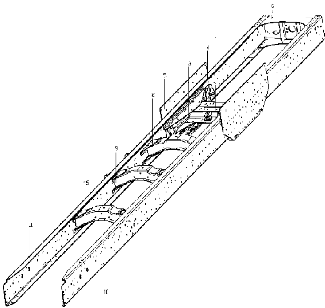
C7-4 CHASSIS FRAME FOR 6×4 TIPPER TRUCK/6×4自卸车车架 Fig. C7-4
