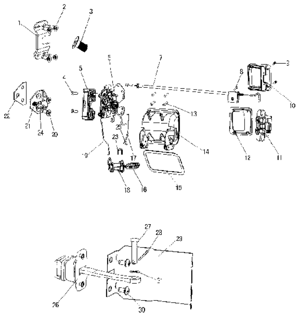
C12-18 D00R LOCK/门锁 Fig. C12-20
