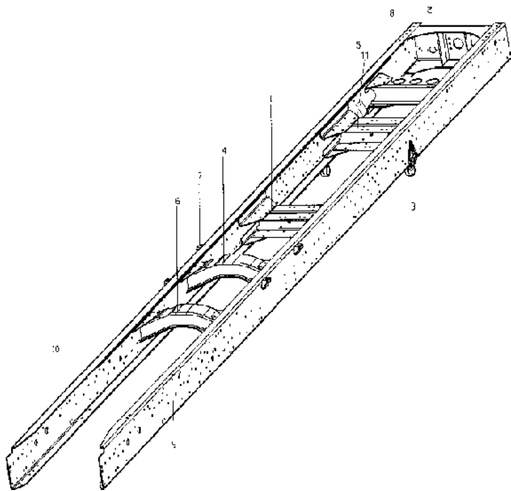
C7-3 CHASSIS FRAME FOR 4×2 CARGO TRUCK/4×2载货车车架 Fig. C7-3
