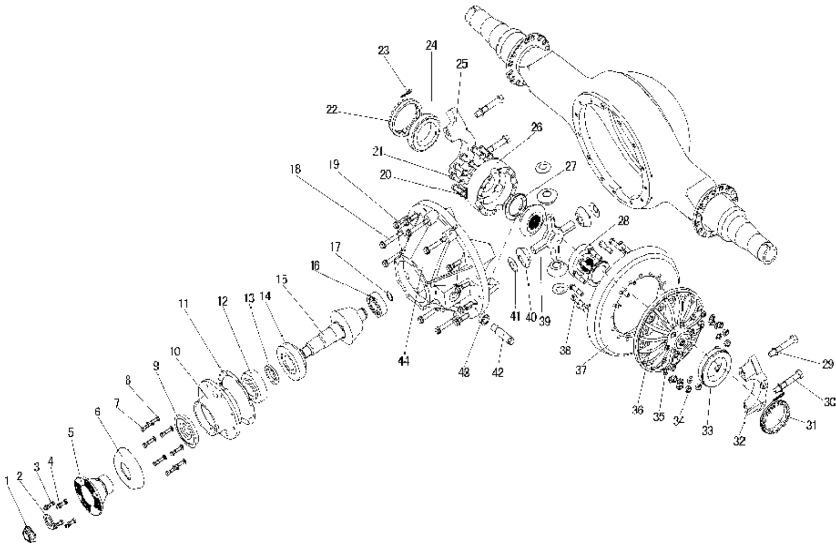
REAR AXLE DRIVE/后桥驱动装置
