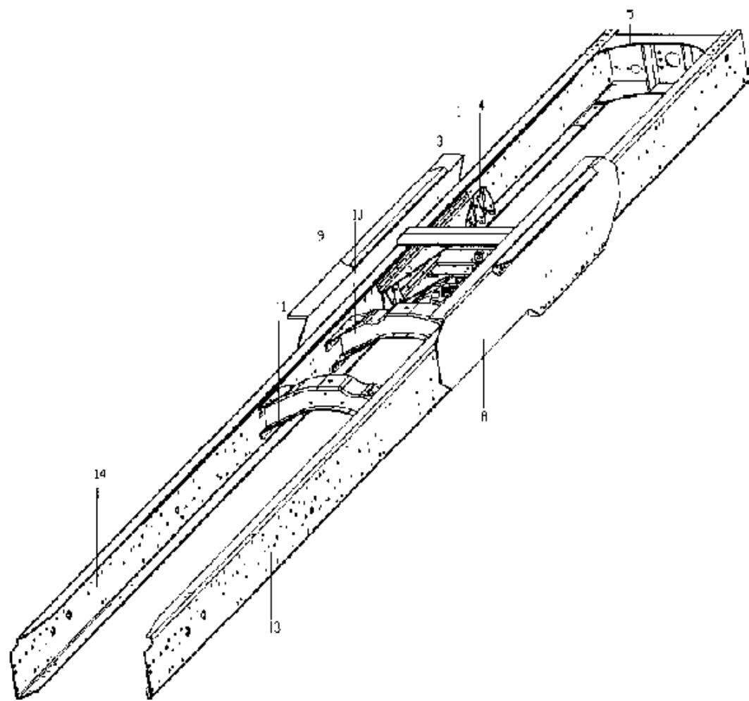
C7-5 CHASSIS FRAME FOR 6×4 TRACTOR TRUCK/6×4牵引车车架 Fig.C7-5
