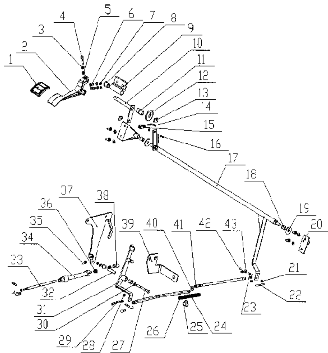
C1-1 OPERATION DEVICE/加速踏板操纵装置
