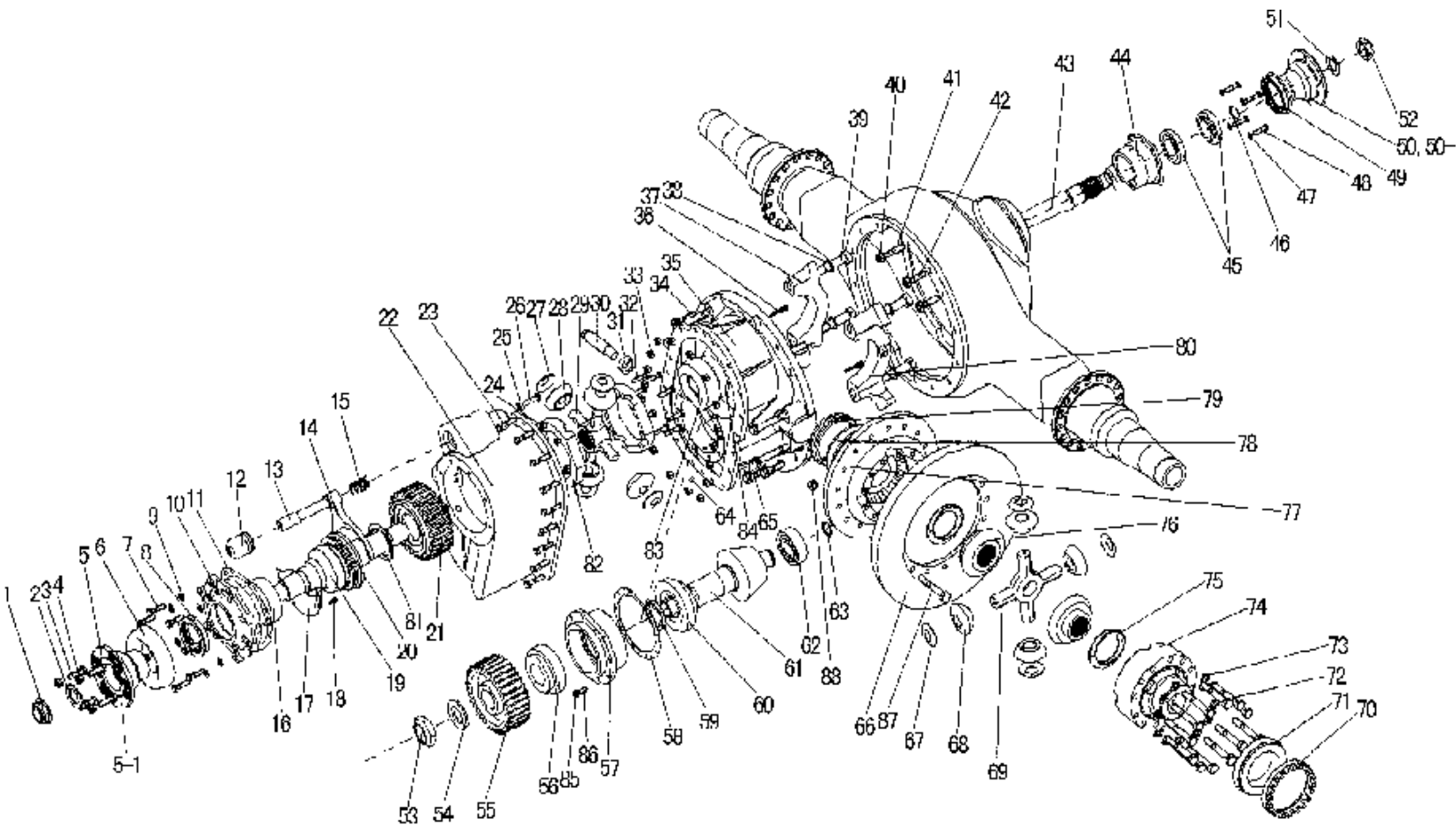
C6-5 FIRST REAR AXLE DRIVE/中桥驱动装置 Fig.C6-5
