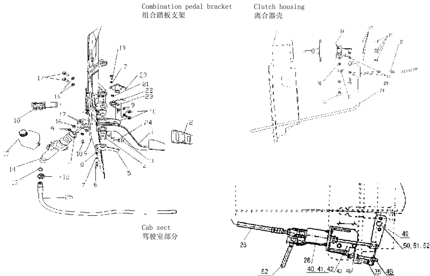
C2-1 CLUTCH OPERATION SYSTEM/离合器操纵系统 Fig.C2-1
