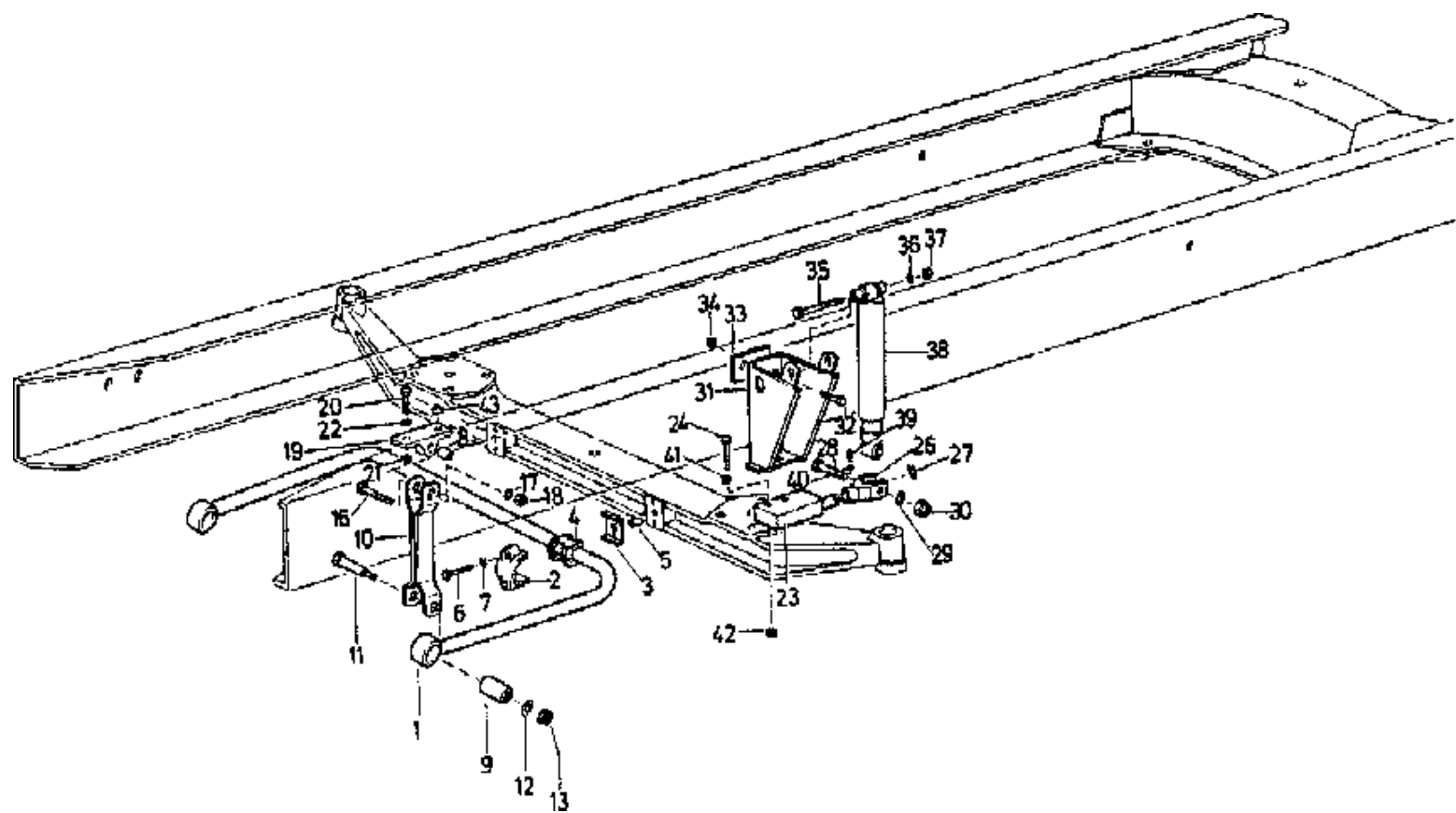
C8-5 4×2, 6×4 STABLIZER, SHOCK ABSORBER FRONT/4×2, 6×4前稳定杆与减振器 Fig.C8-6
