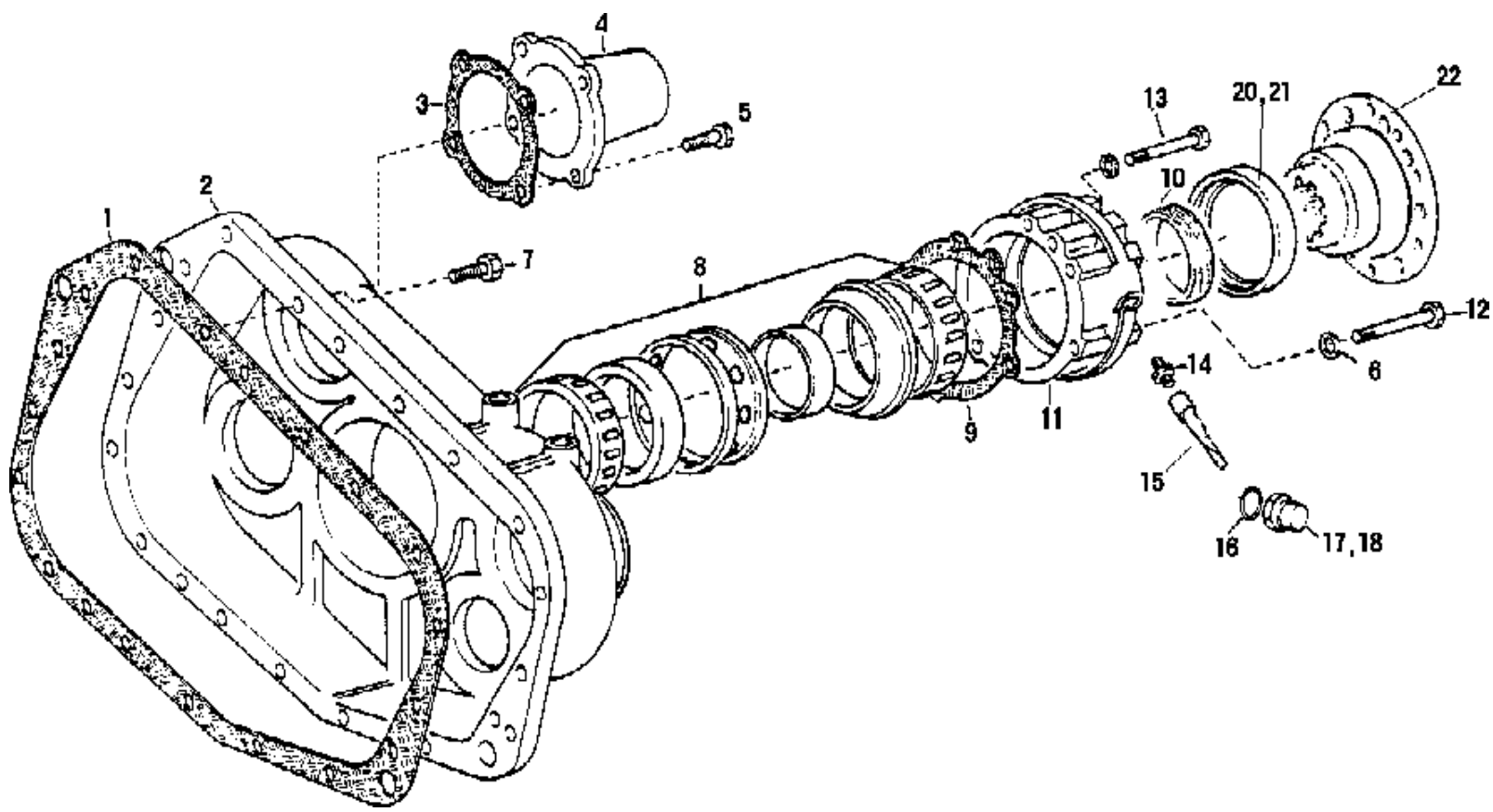
9JS150T REAR COVER/后盖总成
