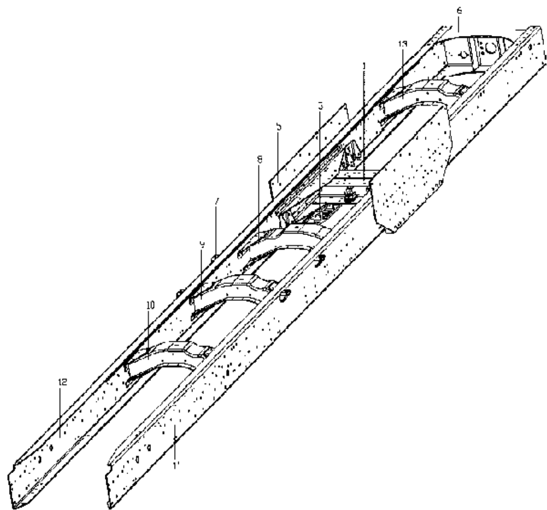
C7-8 CHASSIS FRAME FOR 8×4 TIPPER TRUCK/8×4自卸车车架
