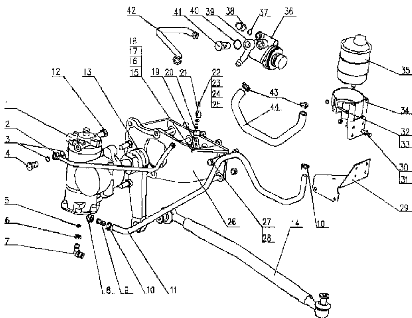
C9-2 4×2, 6×4HYDRAULIC STEERING SYSTEM 4×2, 6×4液压力转向系统 Fig. C9-2
