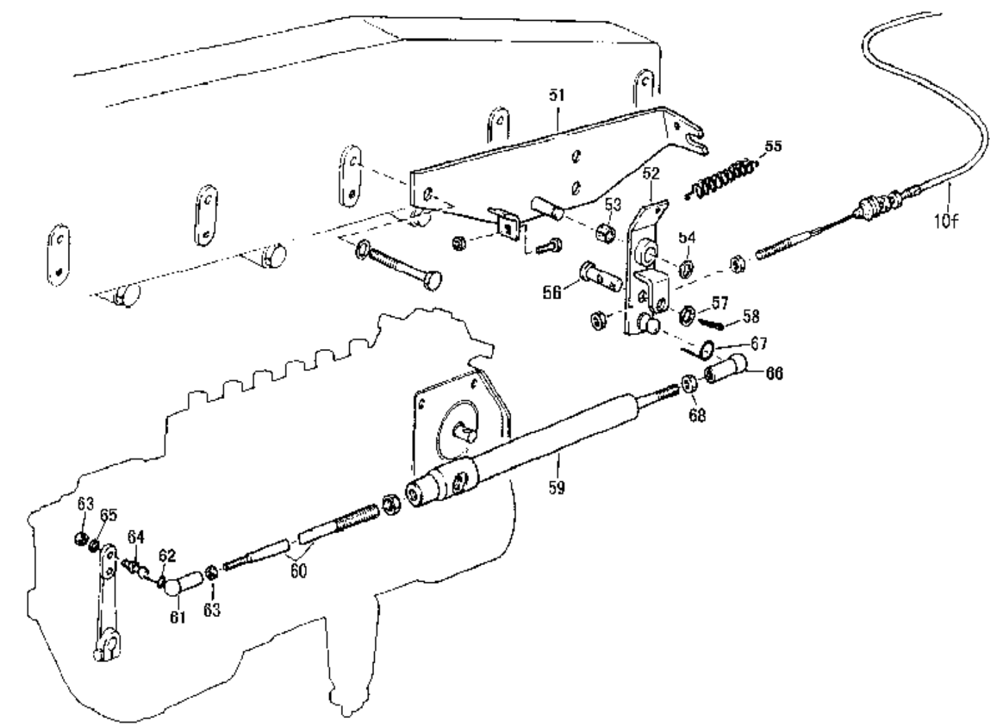
C1-1 OPERATION DEVICE/加速踏板操纵装置
