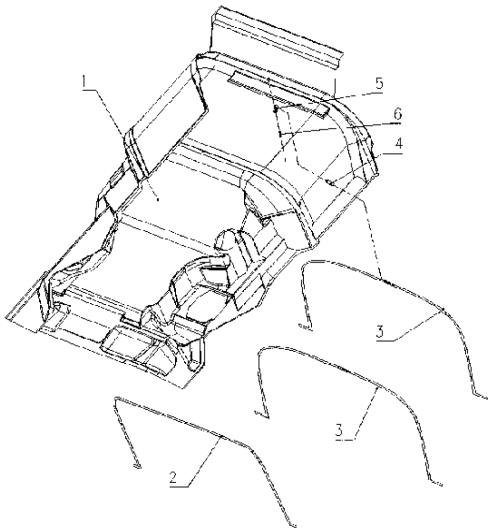
C12-8 SOUNDPROOF ON BOTTOM OF CAB/驾驶室底部隔音材料 Fig.C12-9
