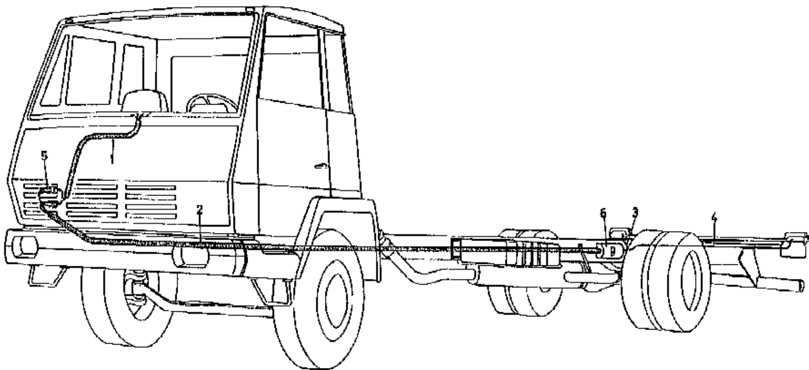
C11-6 ELECTRICAL LINES/电线线束 Fig.C11-6
