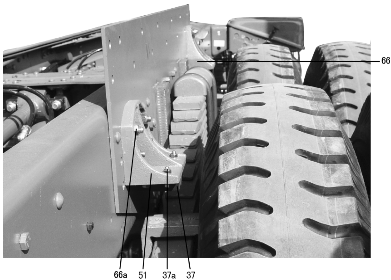
C8-4 6×4, 8×4 SWIVEL SPRING AND SUSPENSION/6×4, 8×4平衡悬架
