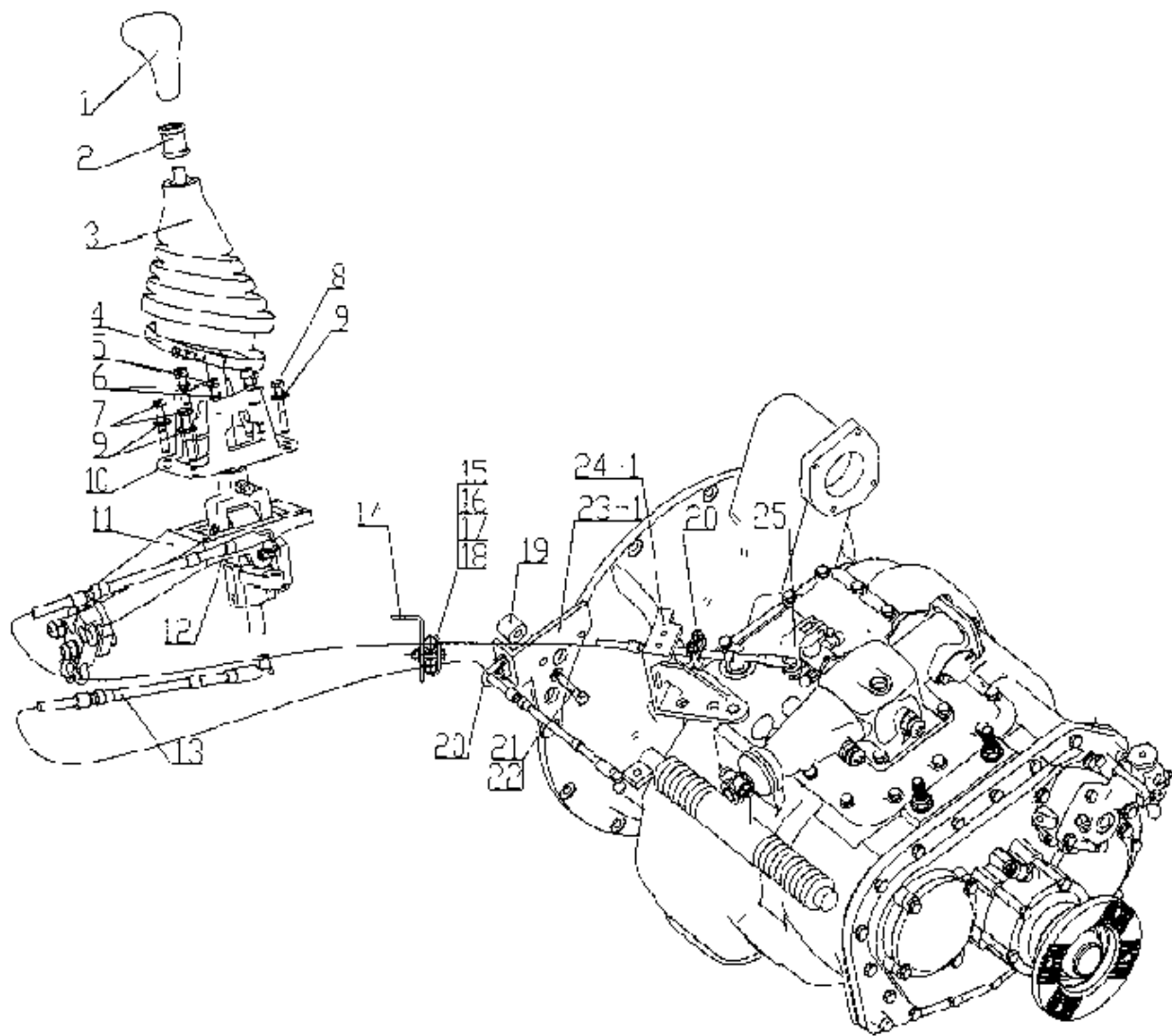
C3-1 GEARBOX GEAR CHANGE SYSTEM/变速器换档操纵装置
