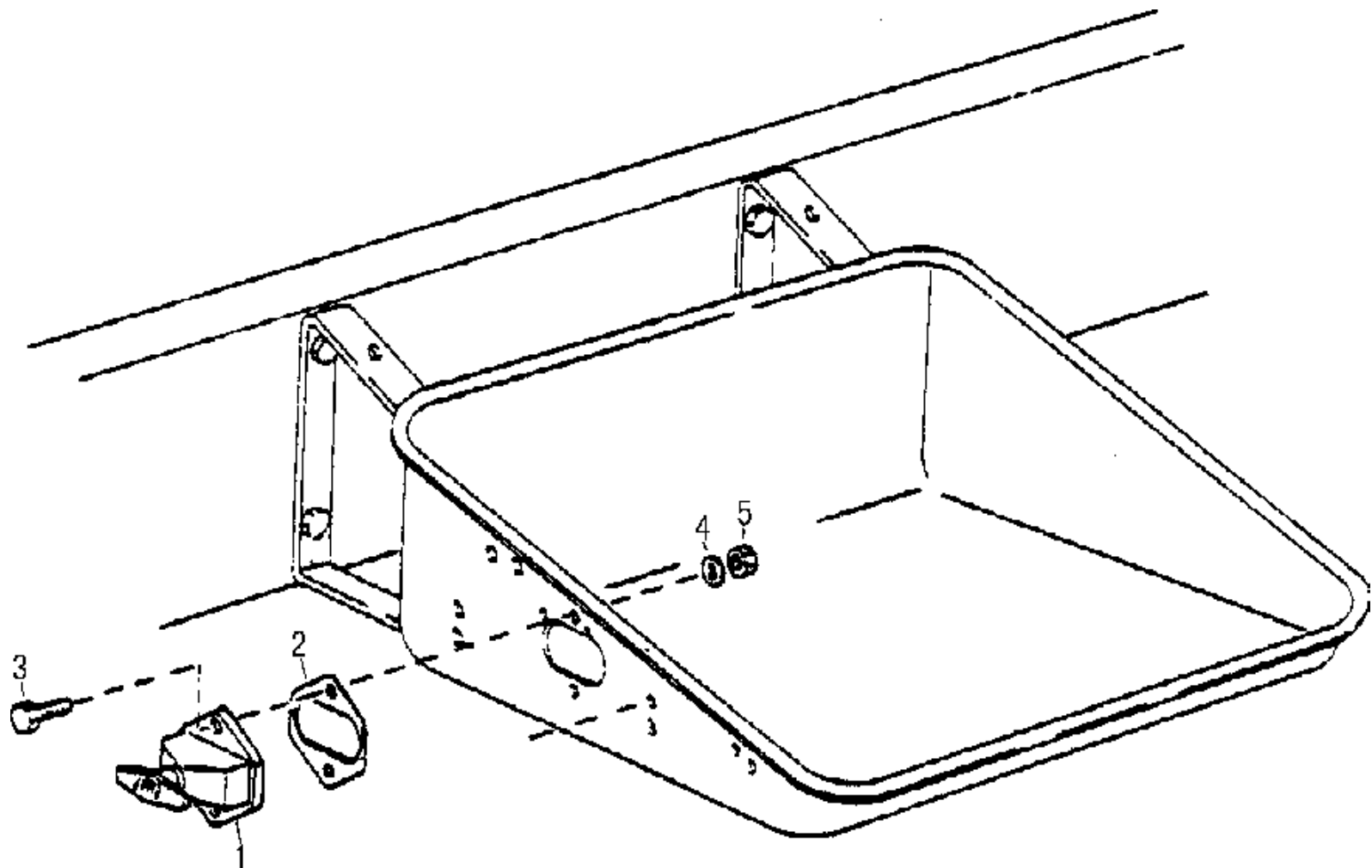
C11-8 BATTERY, MAIN SWITCH/蓄电池，电源总开关 Fig.C11-8
