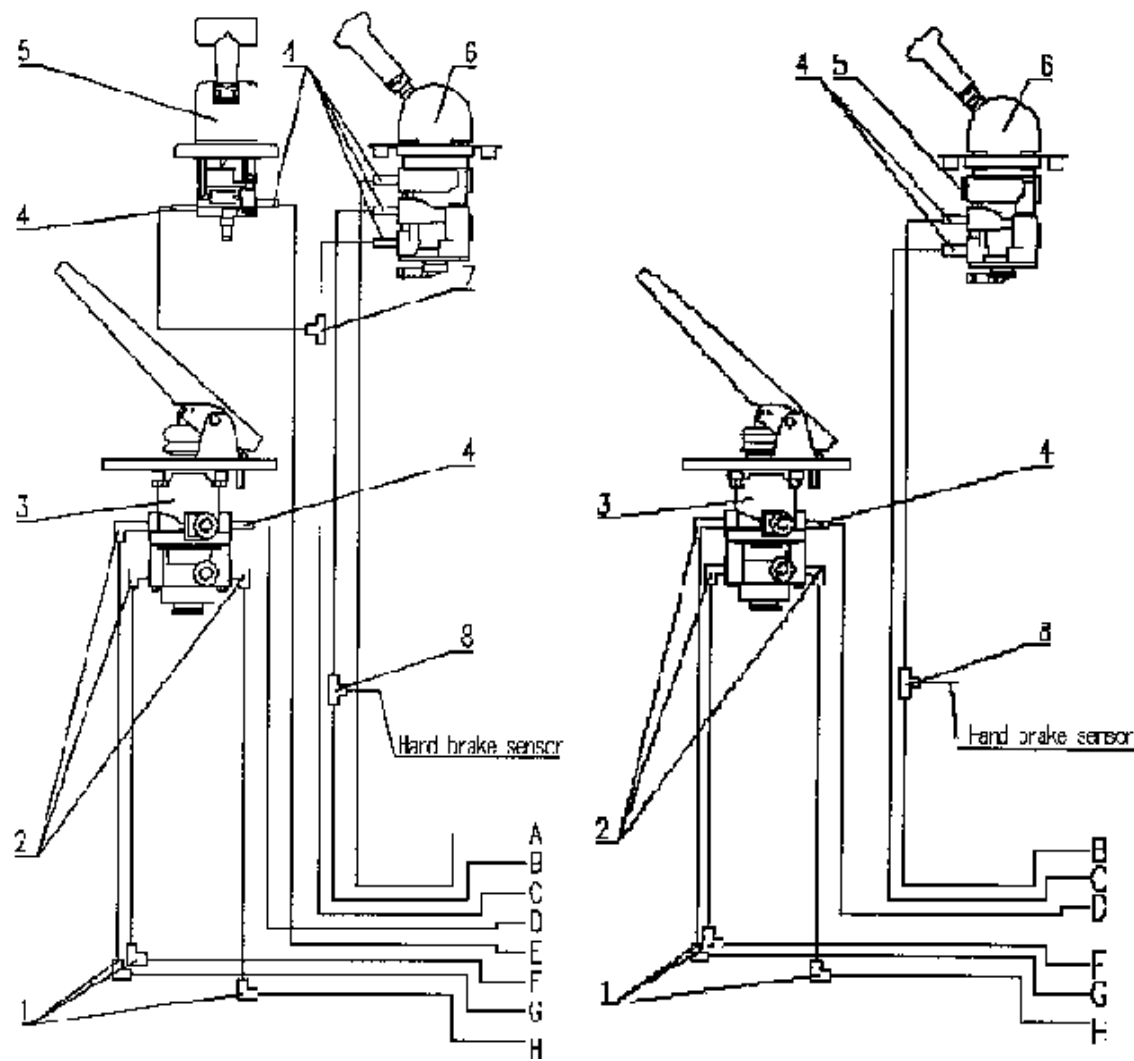
C10-1 BRAKE MECHANISM IN CAB/驾驶室制动操纵机构 Fig.C10-1
