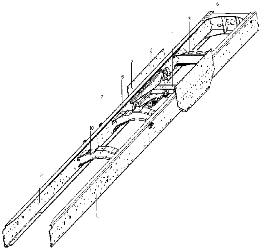
C7-6 CHASSIS FRAME FOR 6×4 CARGO TRUCK/6×4载货车车架 Fig.C7-6
