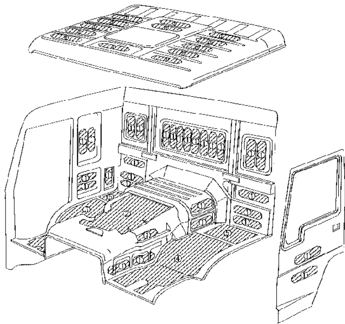
C12-4 SOUND PROOF FOR LONG, HIGH-ROOF CAB/中长，高顶驾驶室隔音材料 Fig.C12-5
