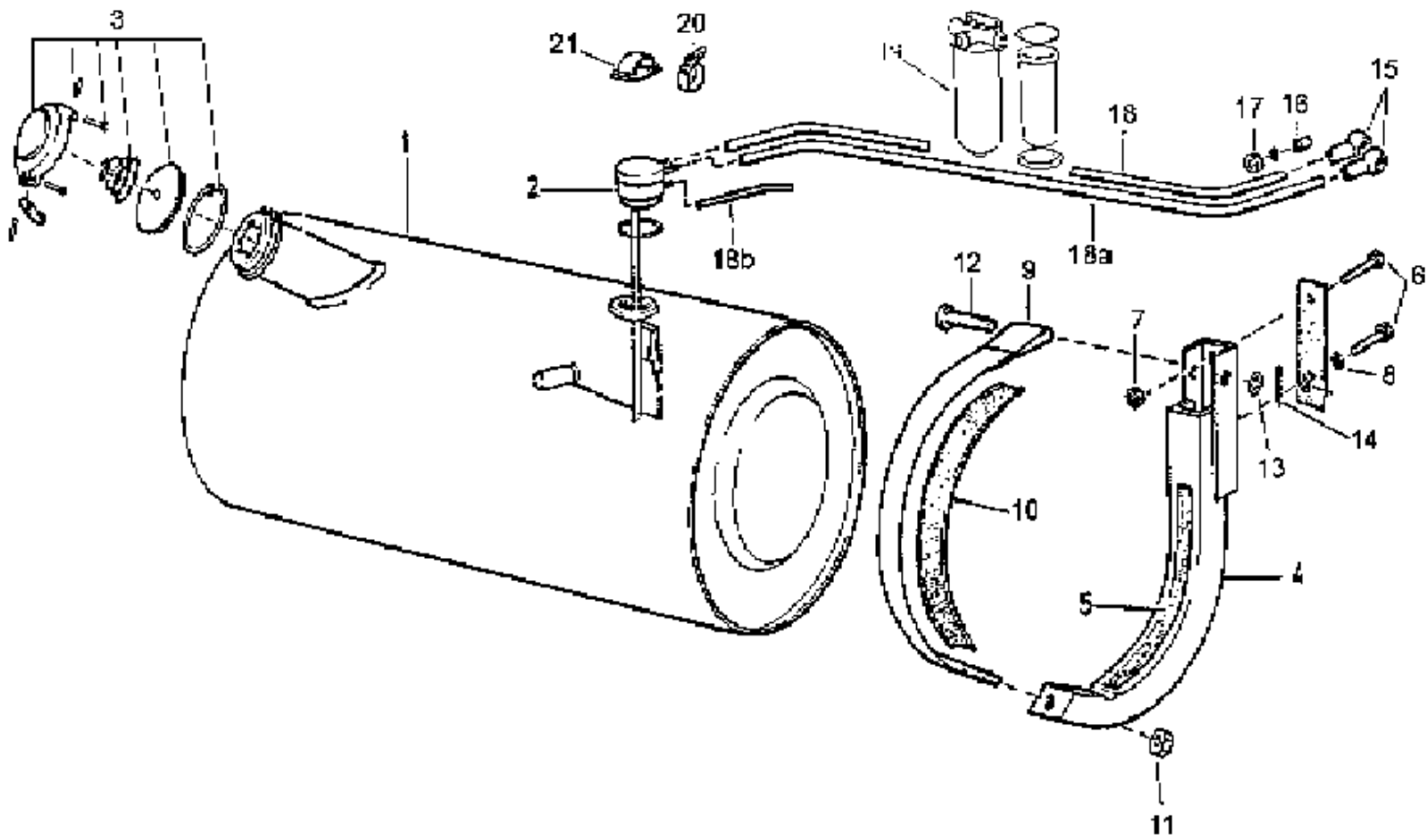
C1-3 200L FUEL AL-TANK/200L铝制燃油箱及管路
