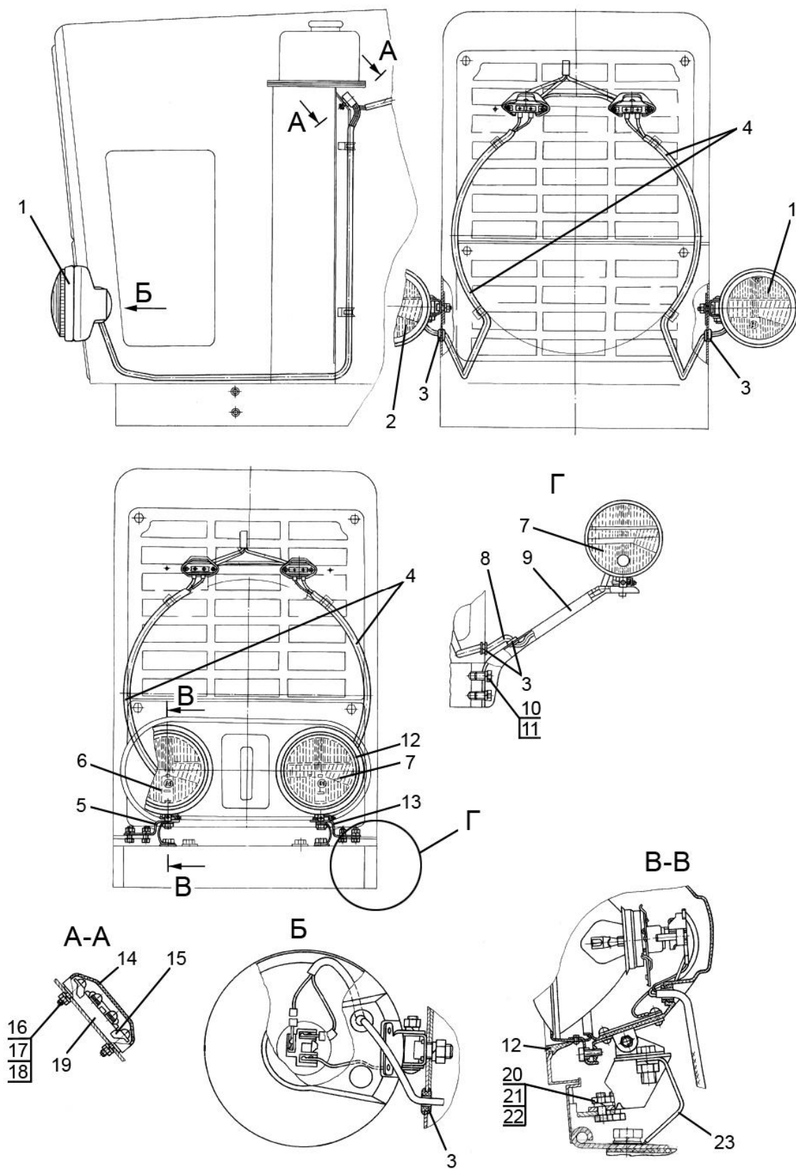
Fig. 37.7 Head lamps installation
