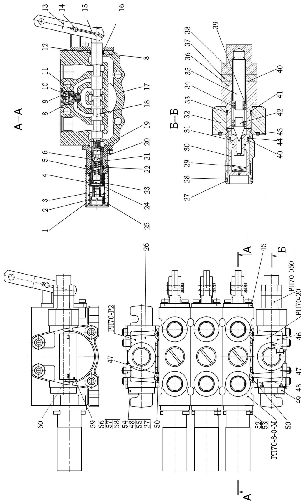
Fig. 46.11. Hydraulic distributor valve ПП70
