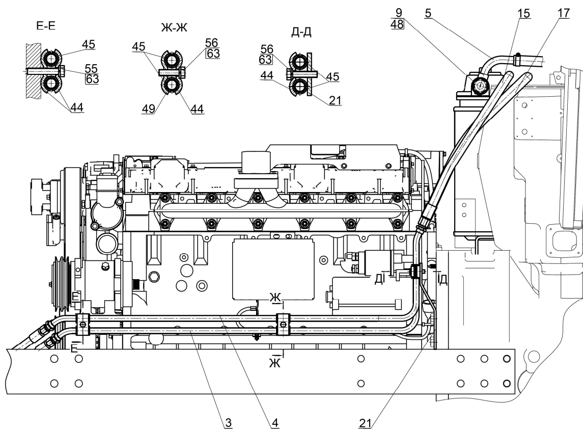
Fig. 34.2a Hydrostatic steering control
