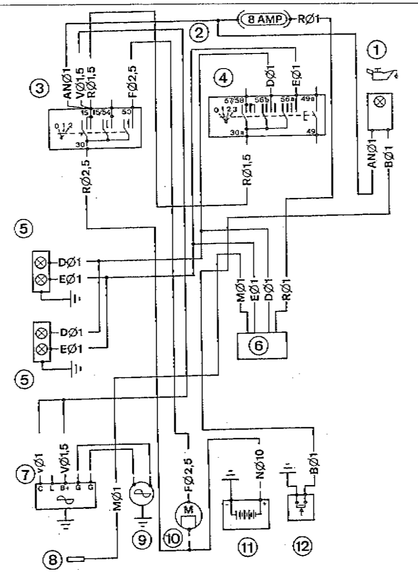
Fig.21 - Electrical system with 3LD-510 engine
