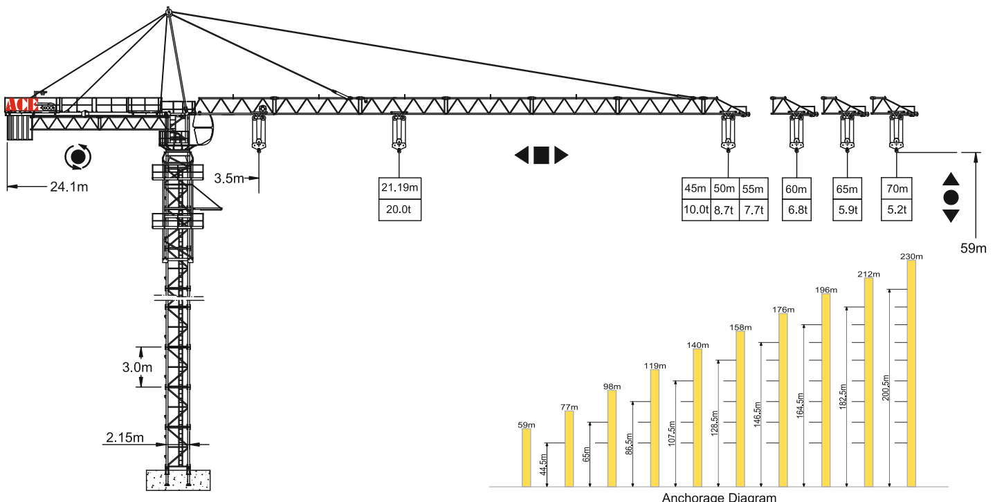
Anchorage Diagram
