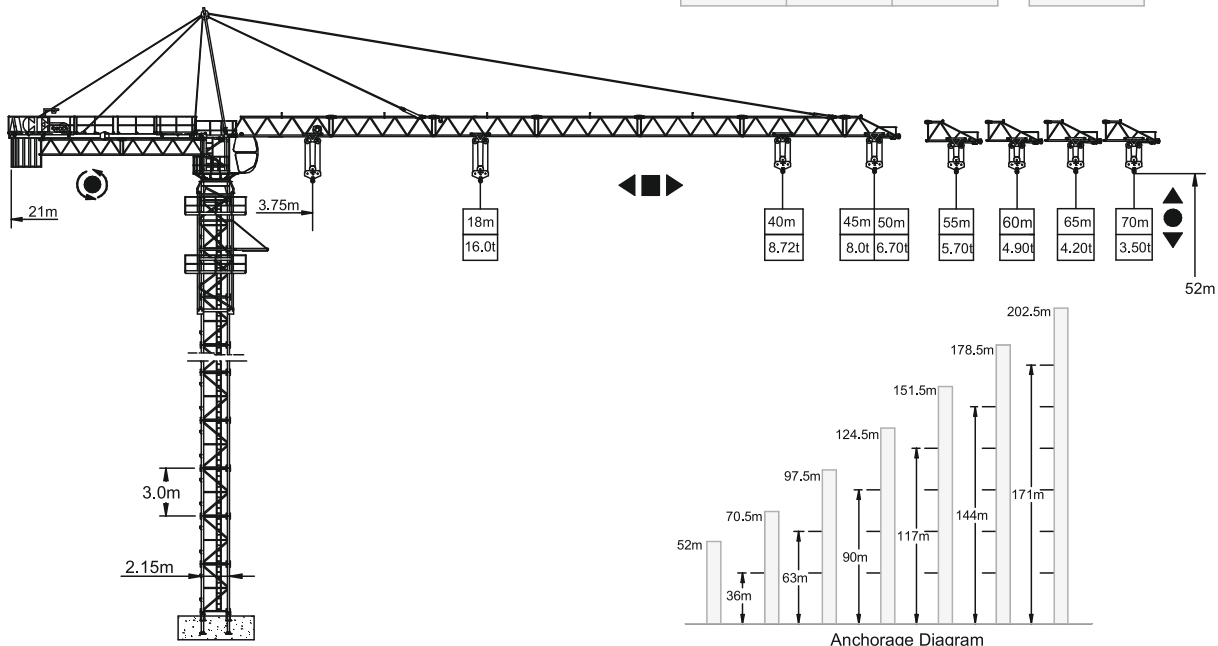
Anchorage Diagram
