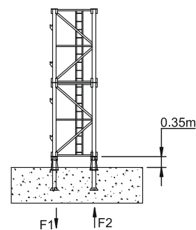
Outrigger Stationary
