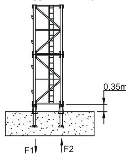
Outrigger Stationary
