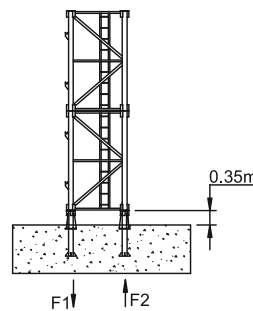
Outrigger Stationary
