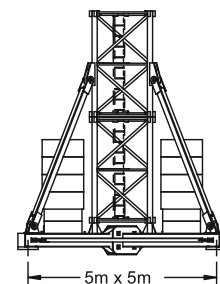
Chassis Stationary/Rail Mounted
