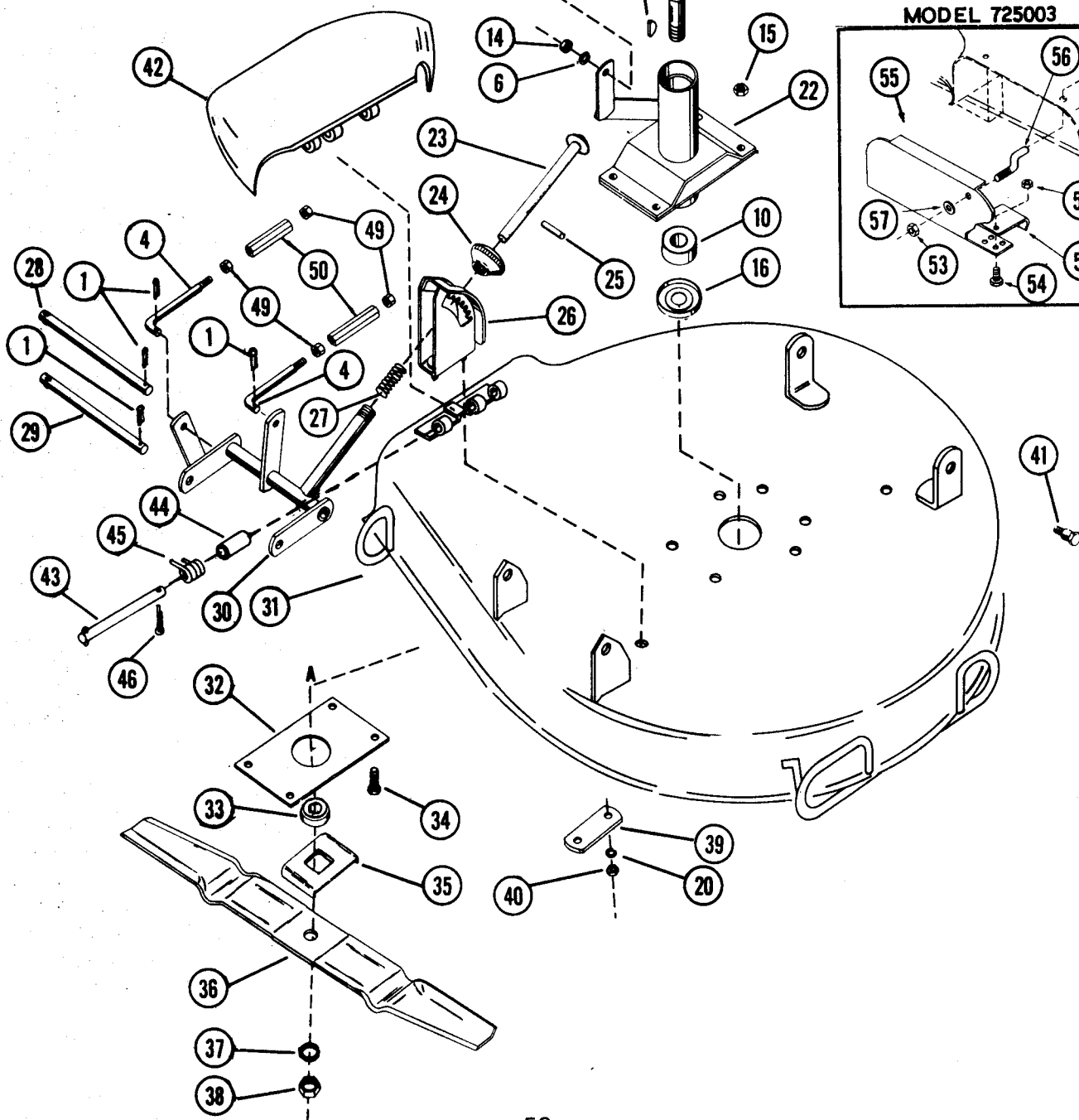
LEAF MULCHER KIT MODEL 725003
