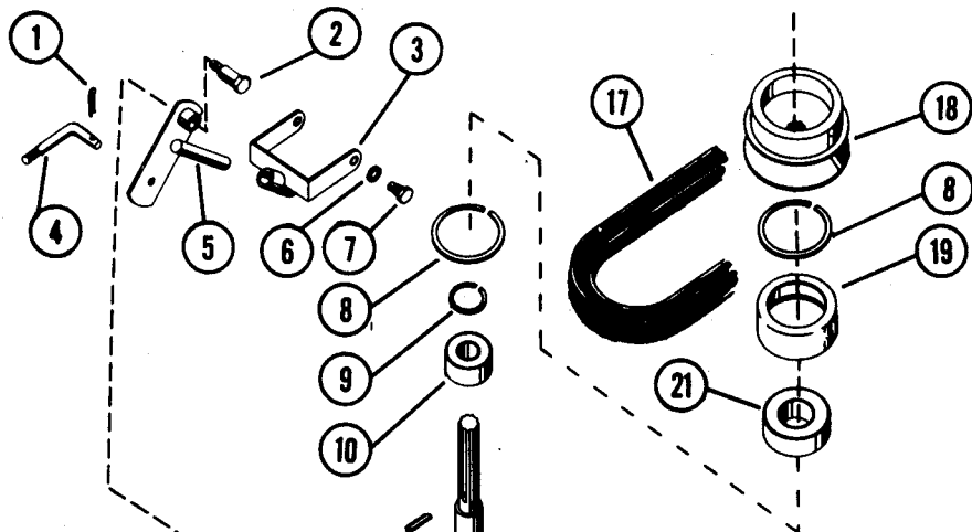
LEAF MULCHER KIT MODEL 725003
