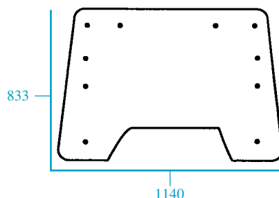
23/4004-4 (D9031, 82000488) Parabrisas abatible - 10 agujeros Windscreen (Opening) - 10 holes
