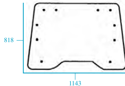
23/4004-5 (D9030, 82004391) Parabrisas abatible - 10 agujeros - claro Windscreen (Opening) - 10 holes - clear
