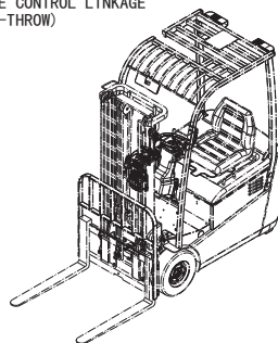
多路阀操纵总成(二片) VALVE CONTROL LINKAGE (TWO-THROW)
