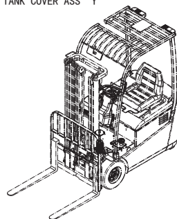
液压油箱附件总成 OIL TANK COVER ASS'Y
