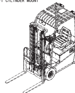
起升油缸安装图 LIFT CYLINDER MOUNT
