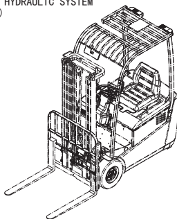
倾斜油缸 TILT CYLINDER
