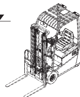
起升油缸安装图/LIFT CYLINDER MOUNT
