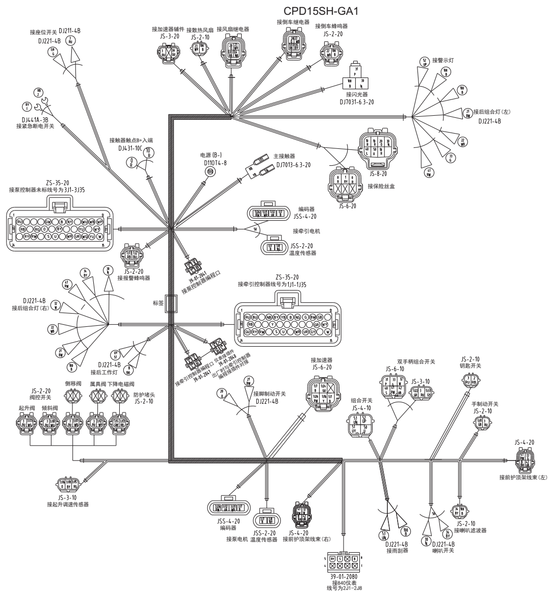
车身线束(选用)/WIRE HARNESS, BODY (OPTION)
