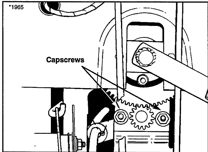
Figure 31. Steering Gear Adjustment
