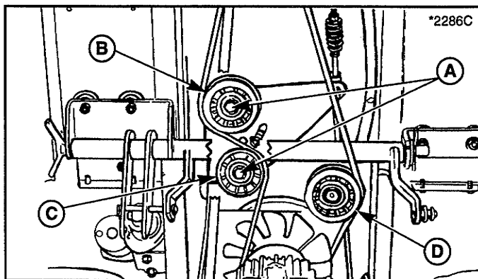
Figure 34. Drive Belt Idler Pulley
