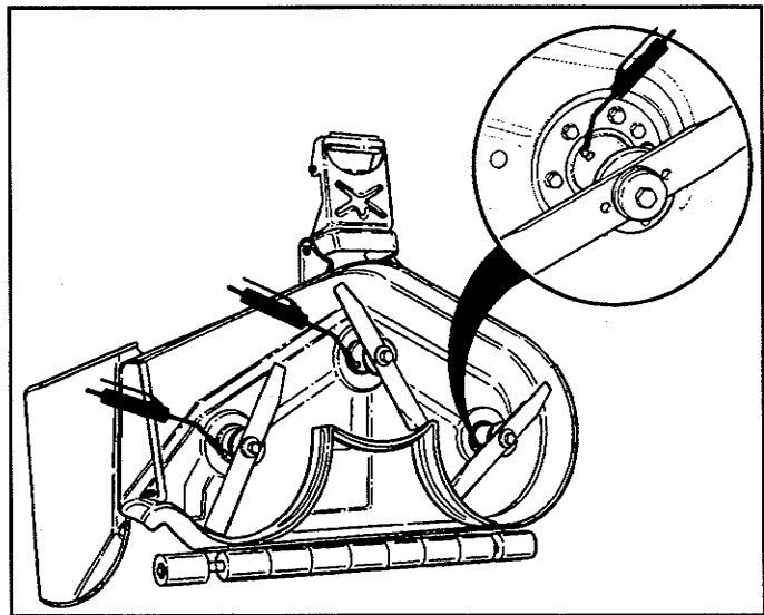
Figure 21. Arbor Lubrication Points
