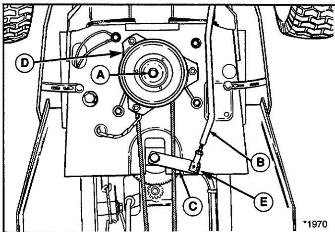
Figure 35. Drive Belt PTO Pulley
