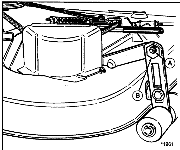
Figure 32. Leveling The Mower Side-to-Side A. Outside Nut B. Eccentric Nut
