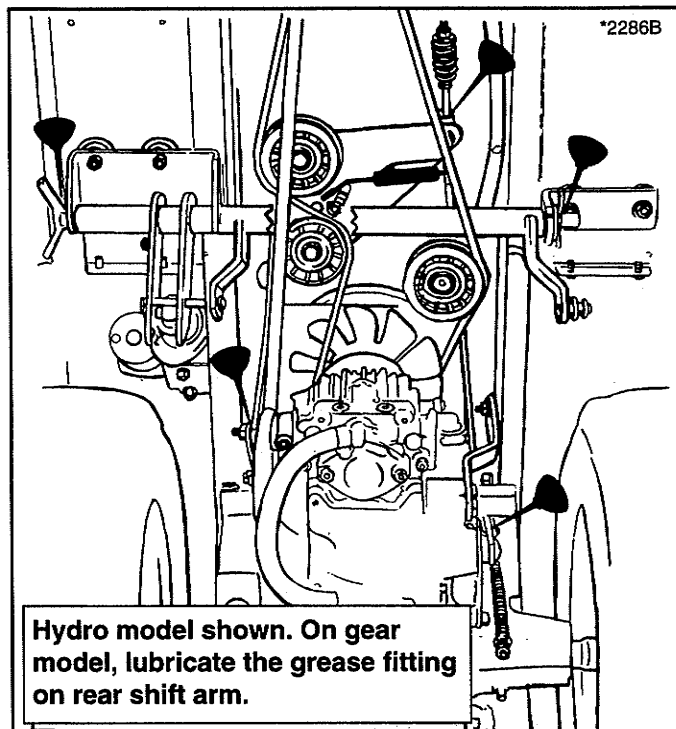
Figure 17. Tractor Lubrication Points - Rear Half
