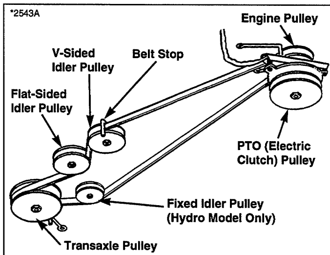
Figure 36. Tractor Drive Belt Routing
