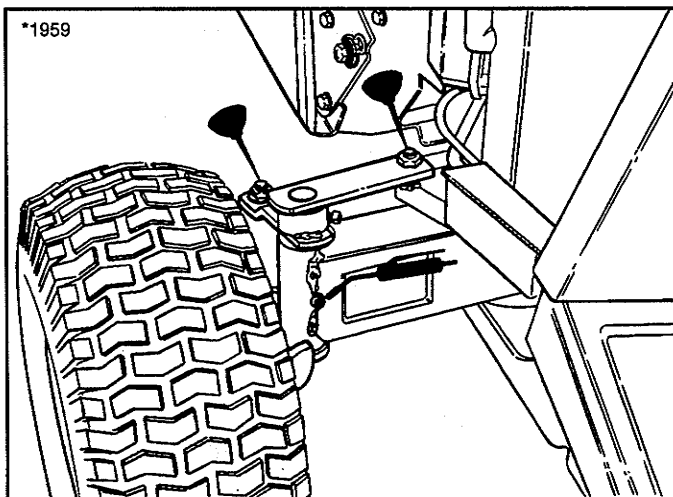
Figure 18. Front Axle Lubrication Points
