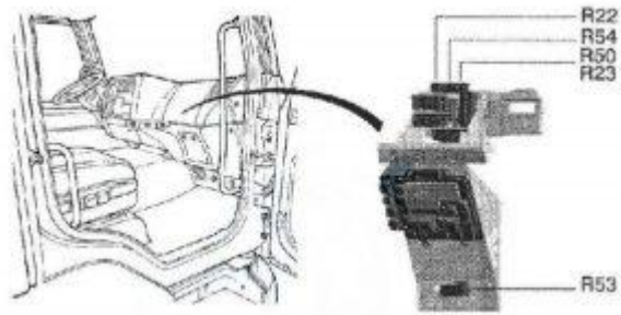
Renault Midlum – fuse box diagram – relay
