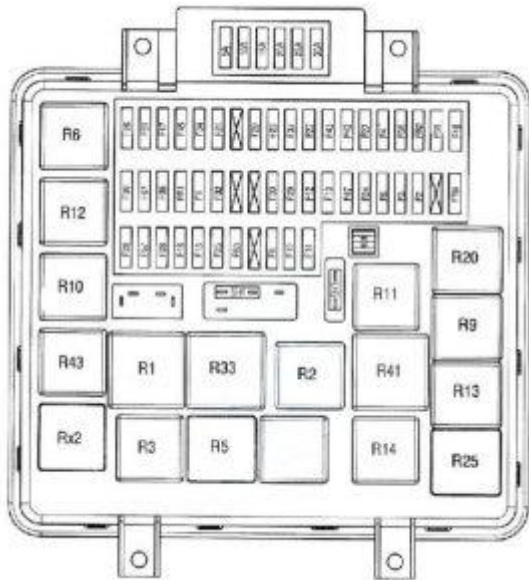
Renault Midlum – fuse box diagram
