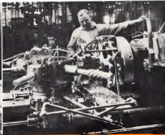
Another machine that reduces manufacturing costs and improves tractor performance. Oliver "Cletrac" sprockets, cut on this machine, are alike as peas in a pod.
