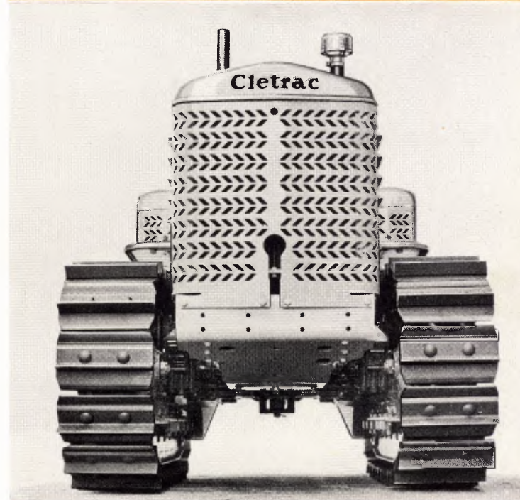
STANDARD MODEL Oliver "Cletrac" is known the world over for economy, dependability and the ability to "take it", regardless of operating conditions. Made in two widths, the standard model (AG and AD) has 42-inch track centers and the hillside model (AGH and ADH) has 50-inch track centers.
