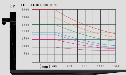
Load Chart
