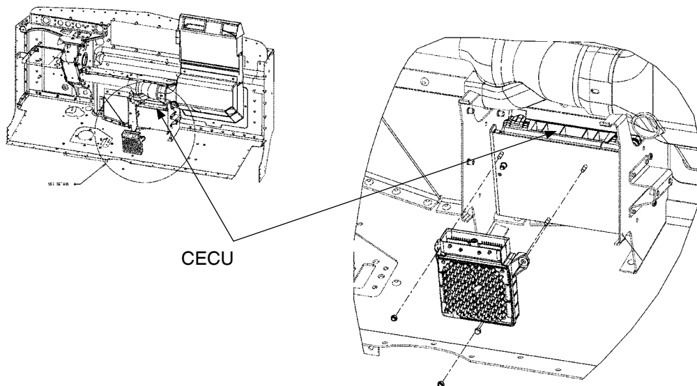
FIGURE 8-5. CECU Location.
