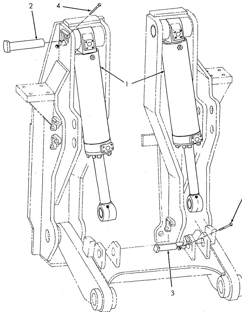
RIPPER CYLINDER MOUNTING
