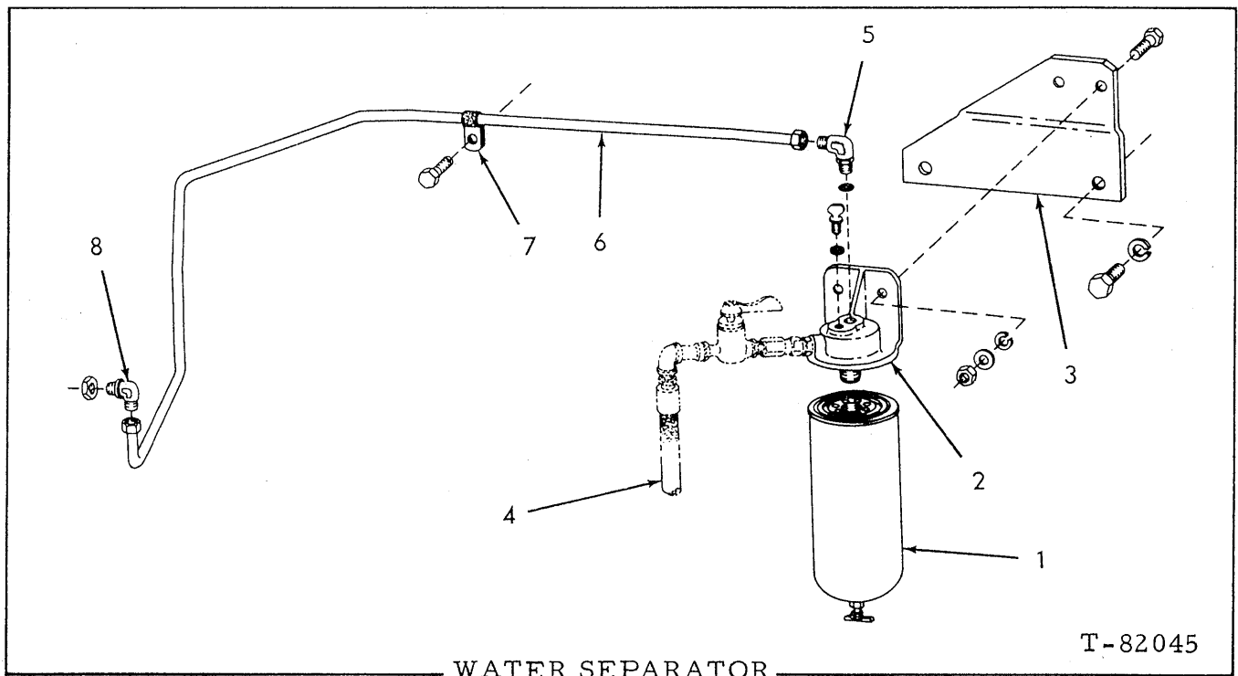
WATER SEPARATOR
