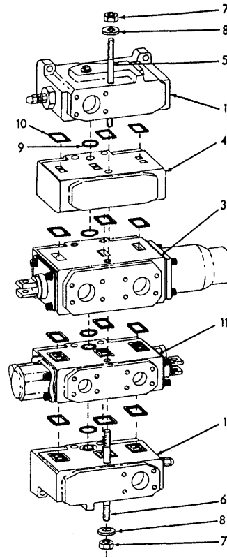
VALVE ASSY. 70665122
