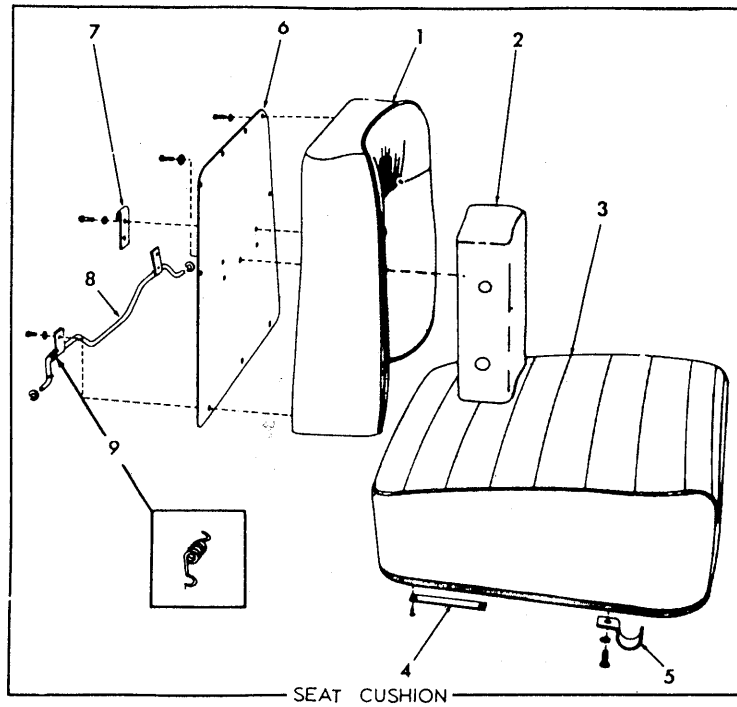
SEAT ASSEMBLY
