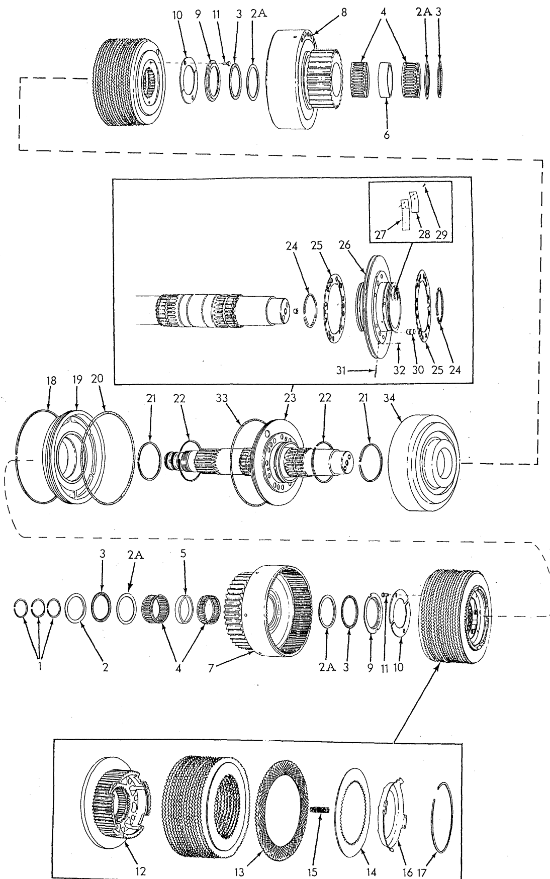
CLUTCH AND SHAFT ASSEMBLY
