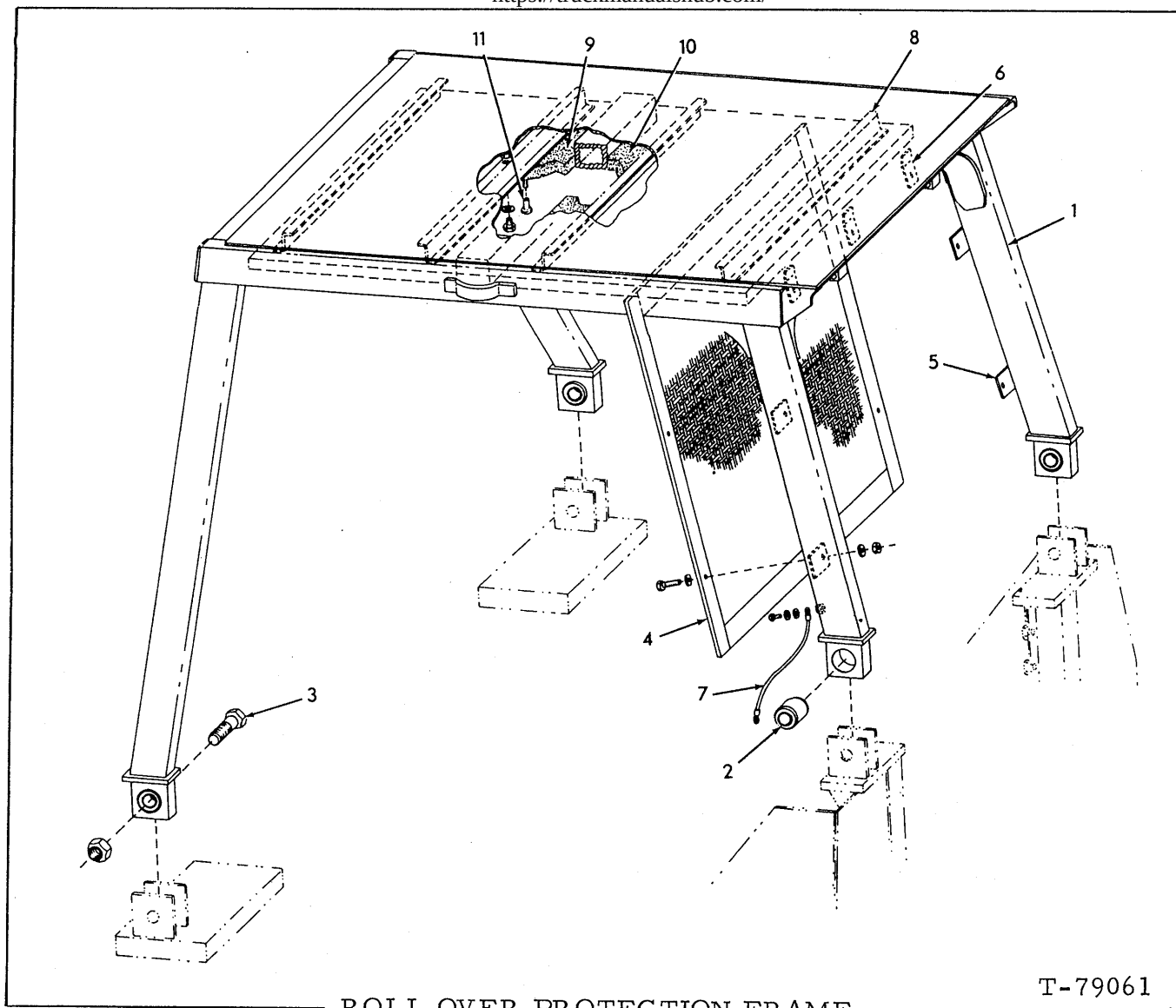
ROLL OVER PROTECTION FRAME
