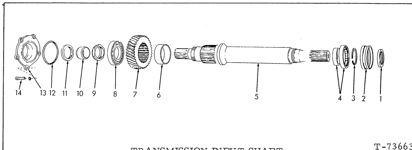
TRANSMISSION INPUT SHAFT
