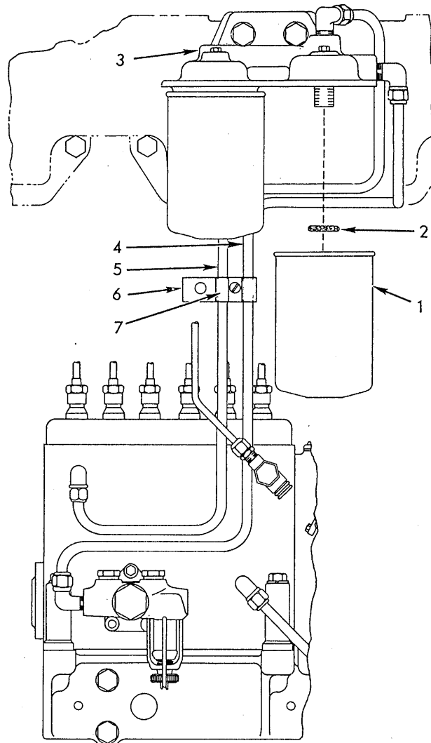
FUEL FILTER
