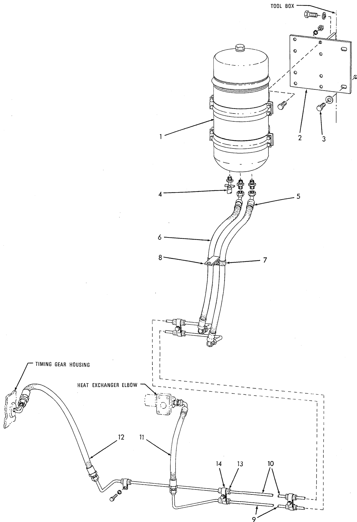
OIL FILTER LINES (By-pass Type)
