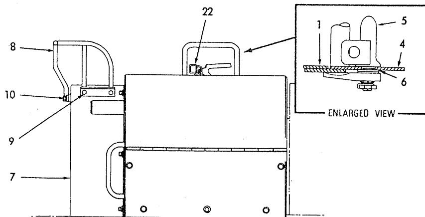
BATTERY AND TOOL BOXES
