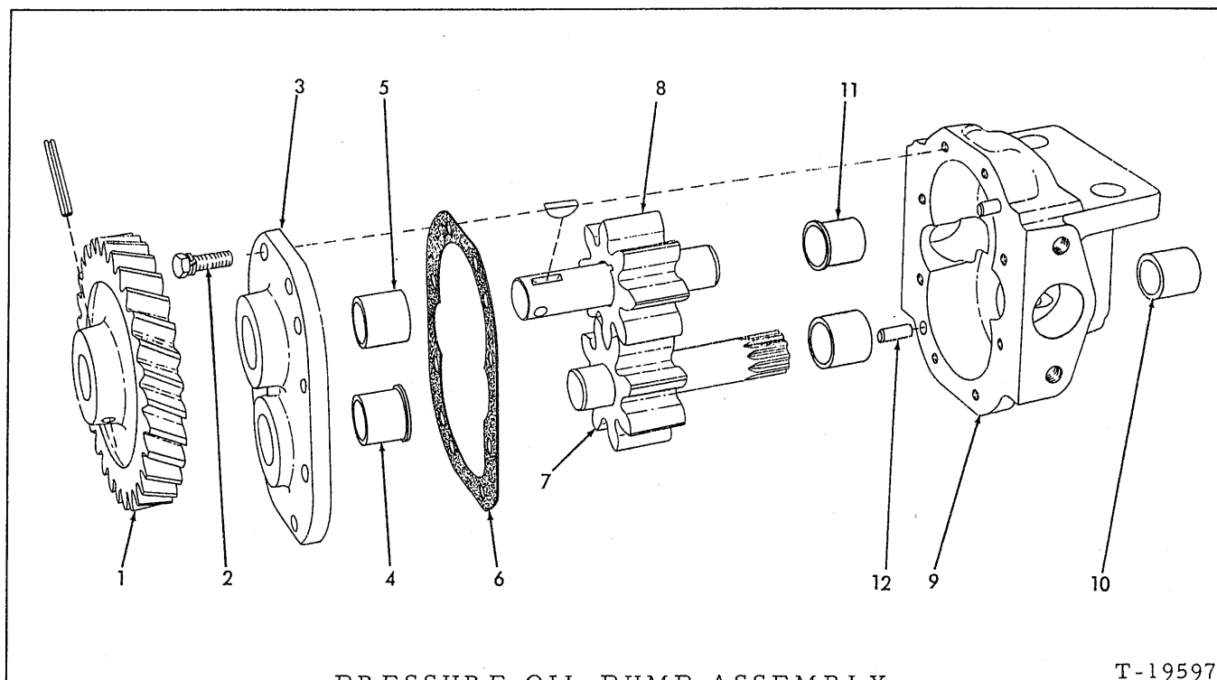
PRESSURE OIL PUMP ASSEMBLY
