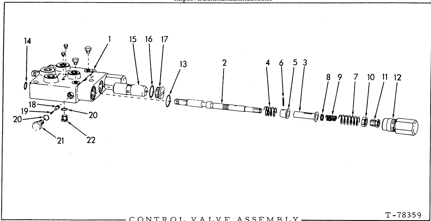
CONTROL VALVE ASSEMBLY
