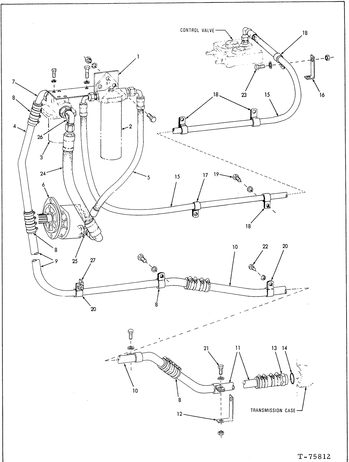
HYDRAULIC STEERING CONTROL
