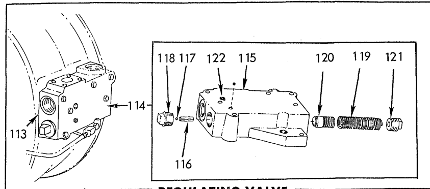
REGULATING VALVE
