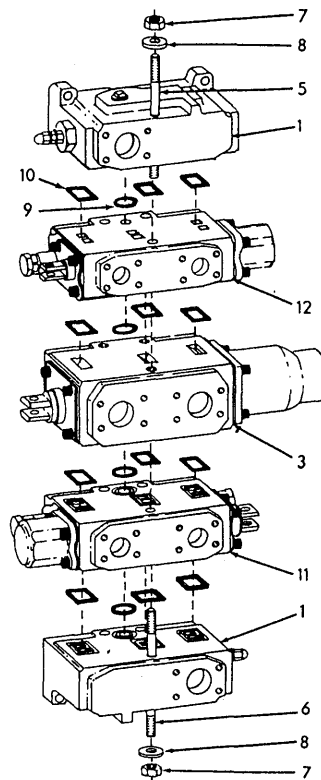
VALVE ASSY. 70662085, 70686070, 73110105
