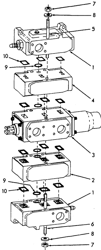
VALVE ASSY. 70660647, 70686090, 73110106
