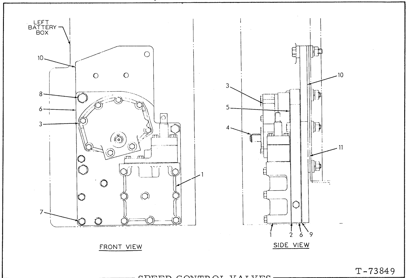
SPEED CONTROL VALVES
