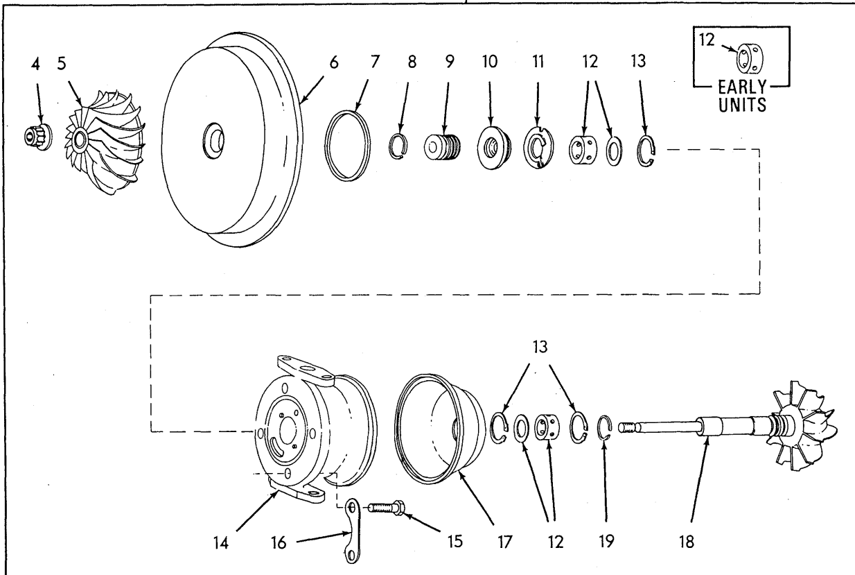
TURBOCHARGER ASSEMBLY
