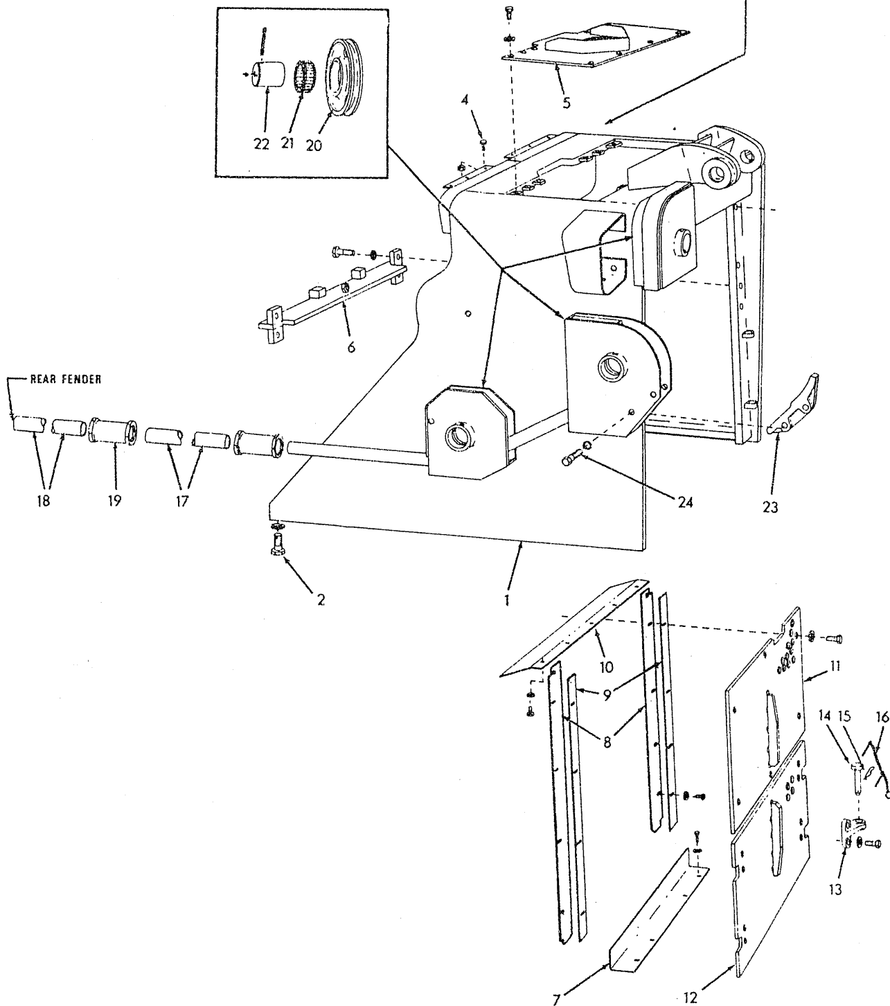
RADIATOR GUARD
