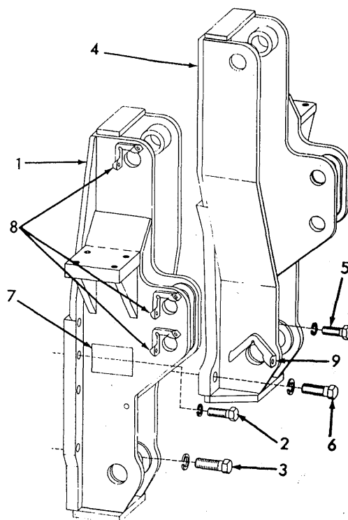
RIPPER MOUNTING FRAME
