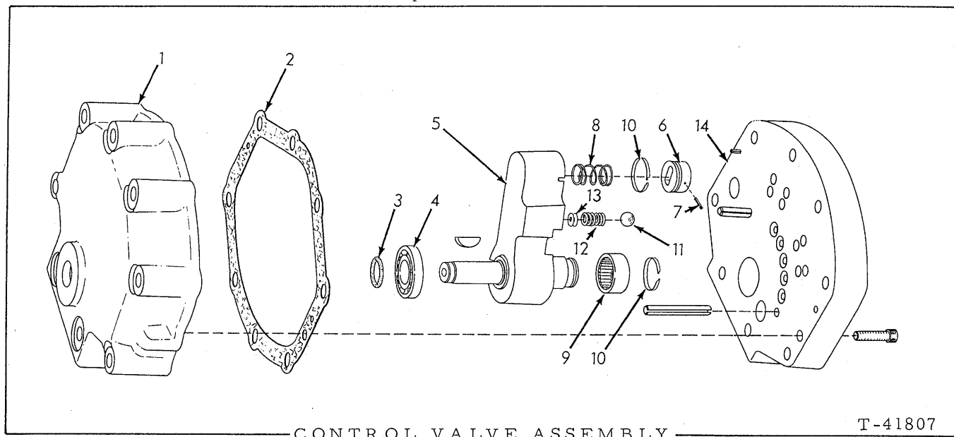
CONTROL VALVE ASSEMBLY
