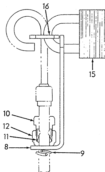
ENGINE OIL DIPSTICK
