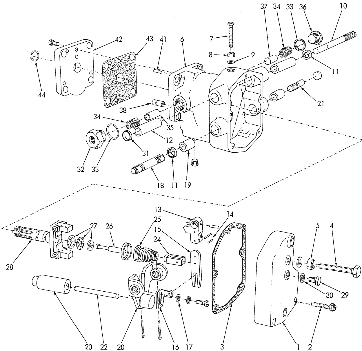
GOVERNOR ASSEMBLY
