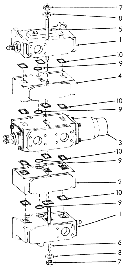
CONTROL VALVE
