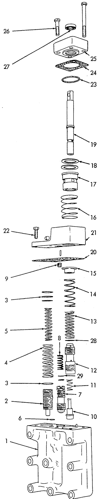
MODULATING VALVE ASSEMBLY
