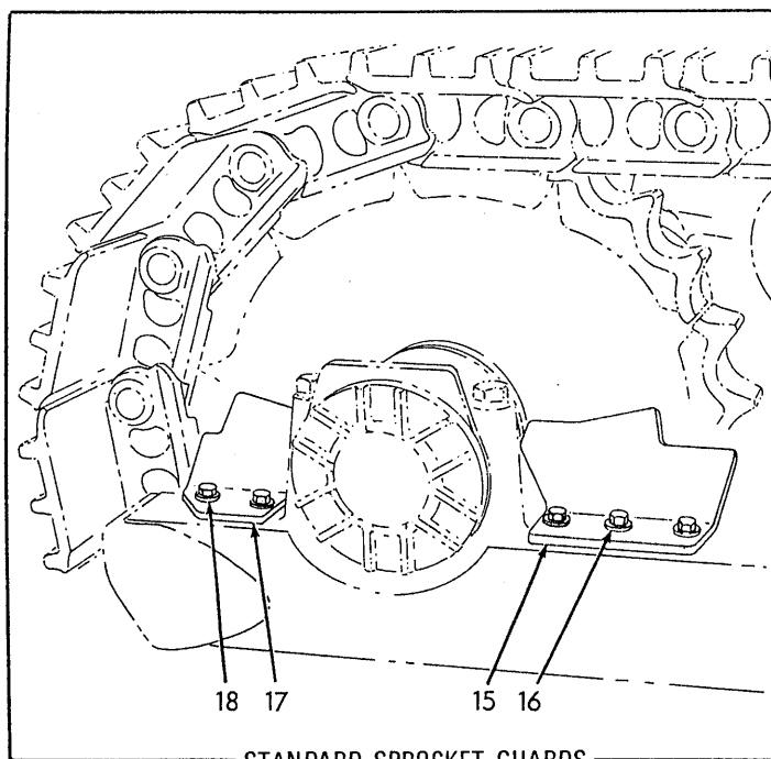
STANDARD SPROCKET GUARDS
