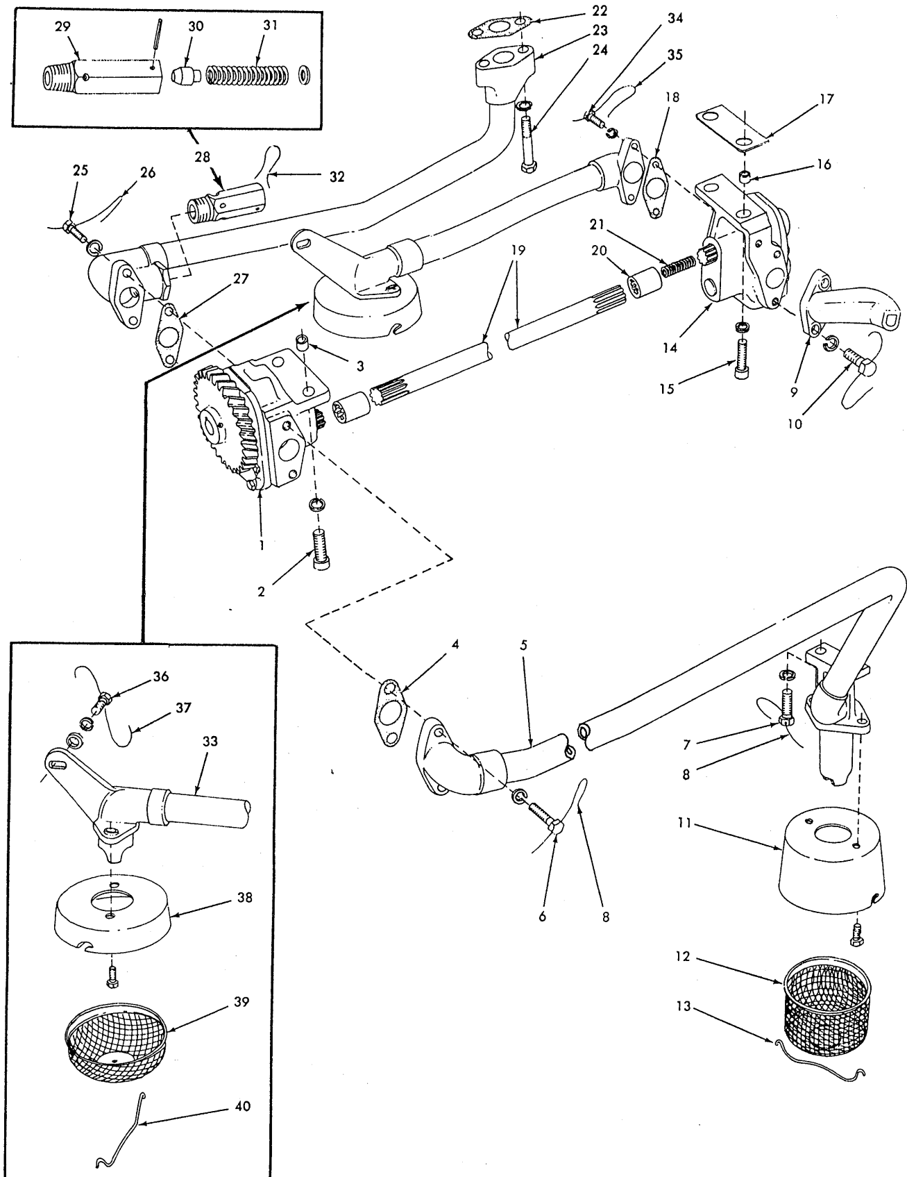
OIL PUMPS
