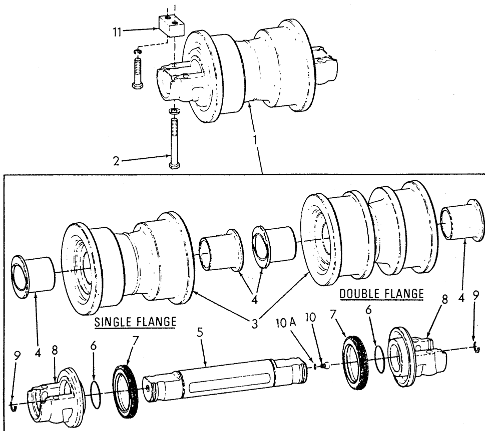
TRACK ROLLERS
