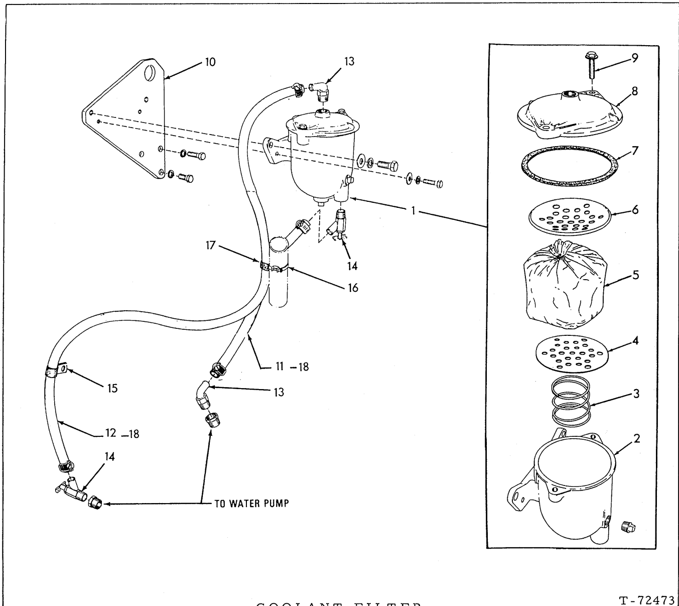
COOLANT FILTER
