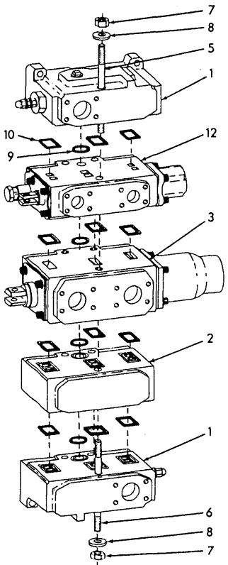
VALVE ASSY. 70665121
