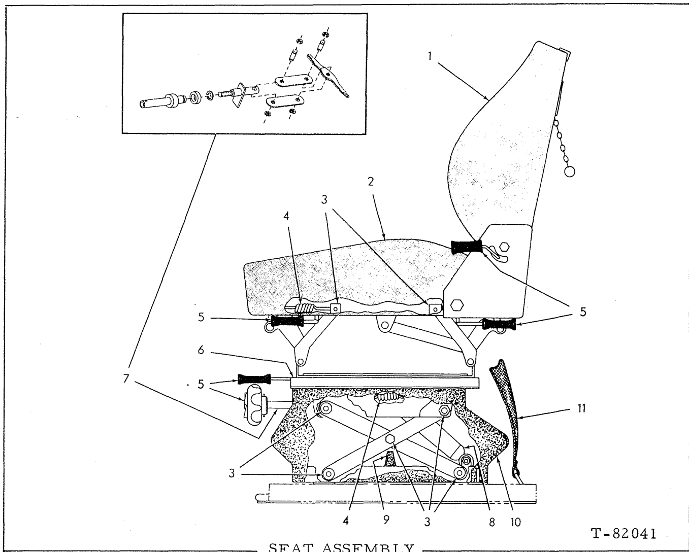
SEAT ASSEMBLY
