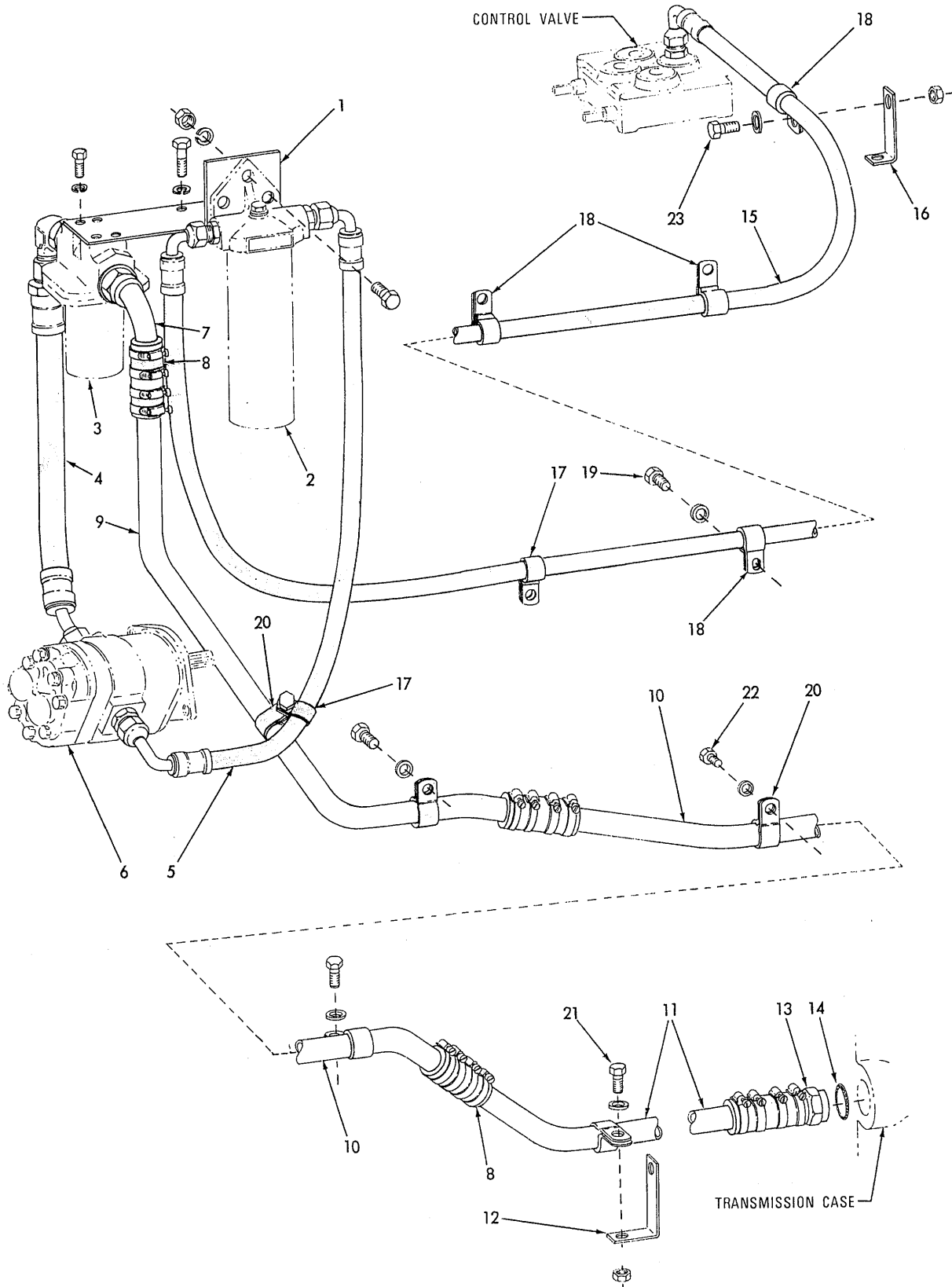
HYDRAULIC STEERING CONTROL
