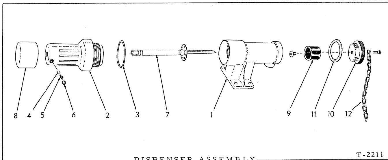
DISPENSER ASSEMBLY
