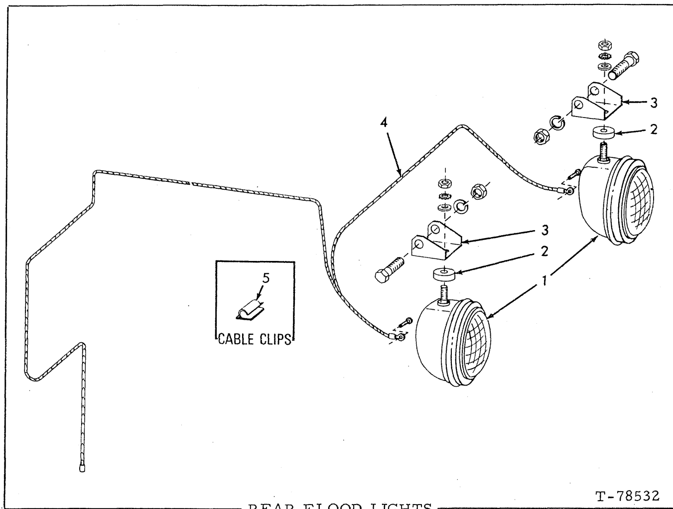
REAR FLOOD LIGHTS
