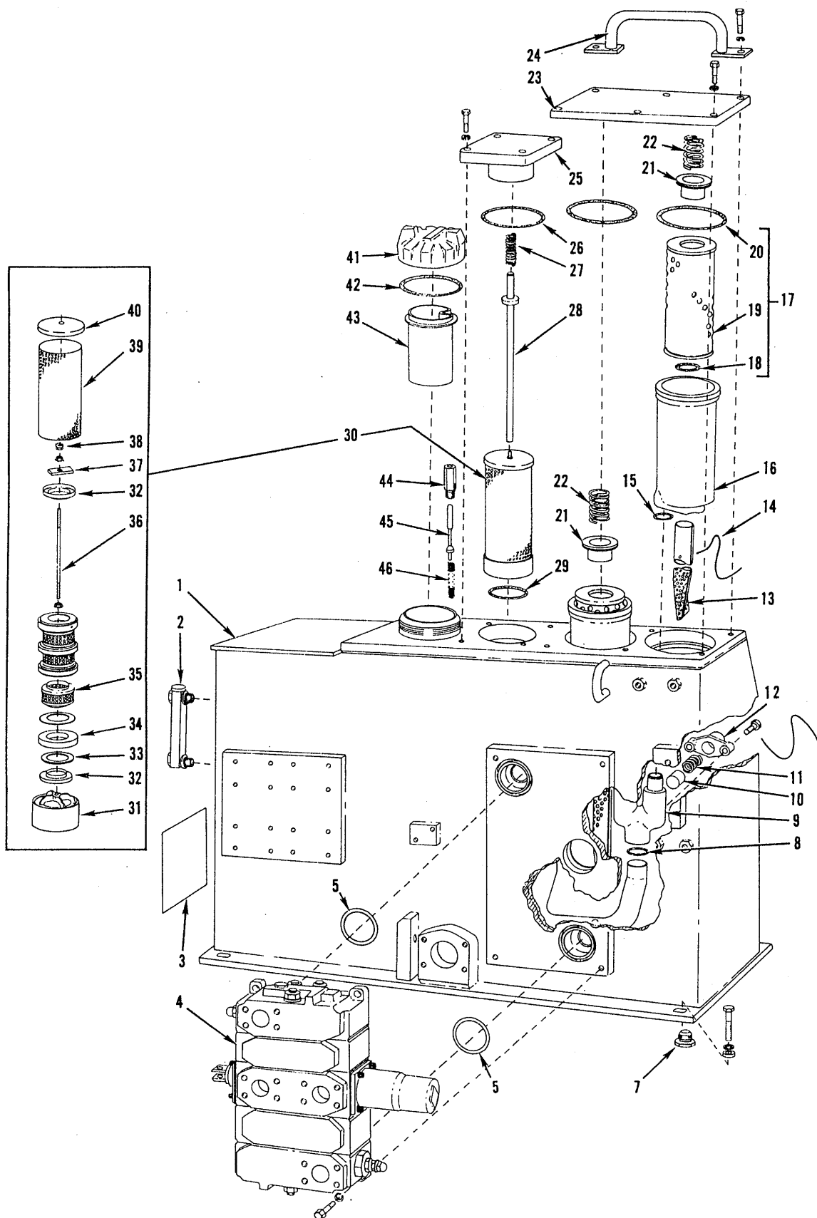
HYDRAULIC TANK AND CONTROL VALVE
