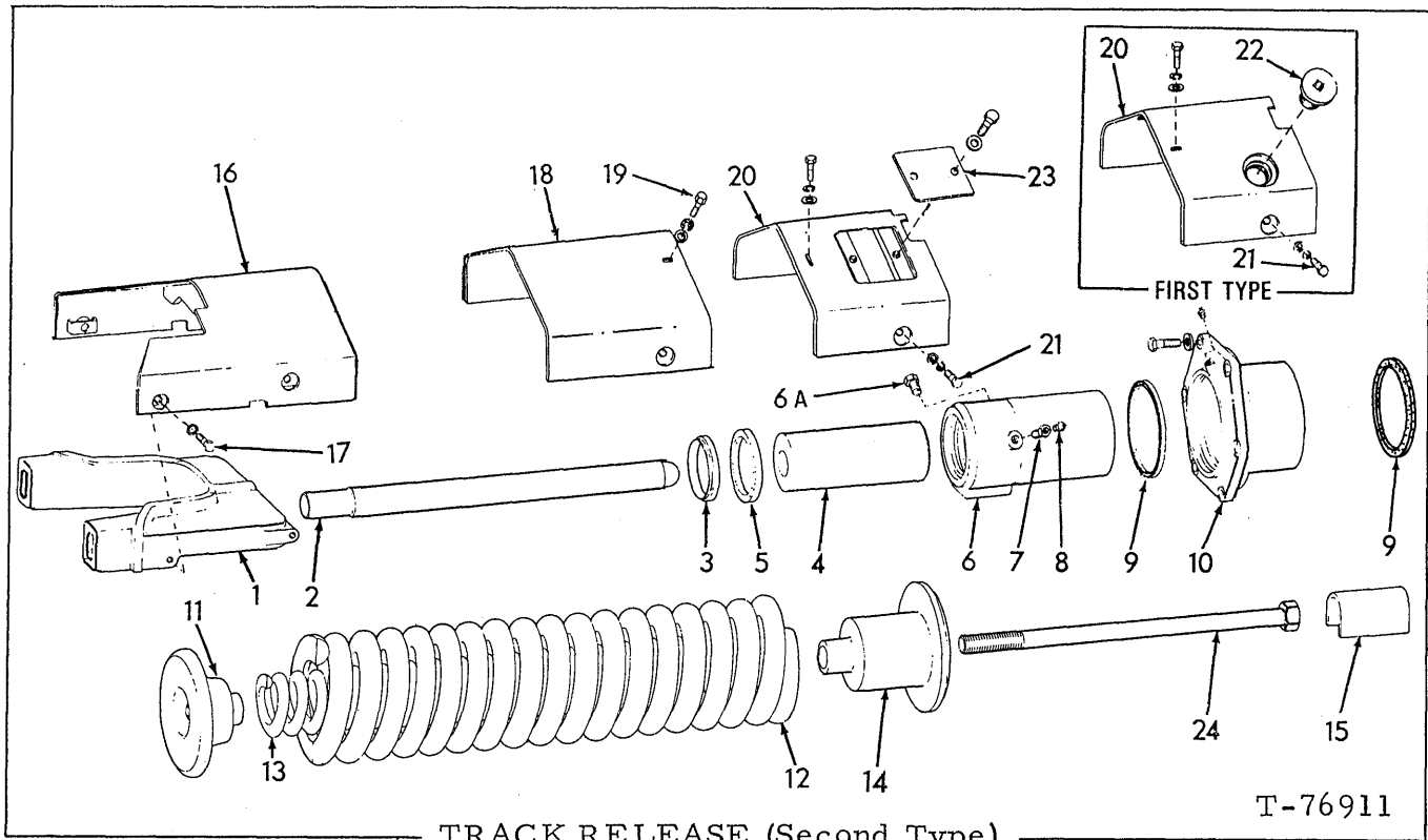
TRACK RELEASE (Second Type)
