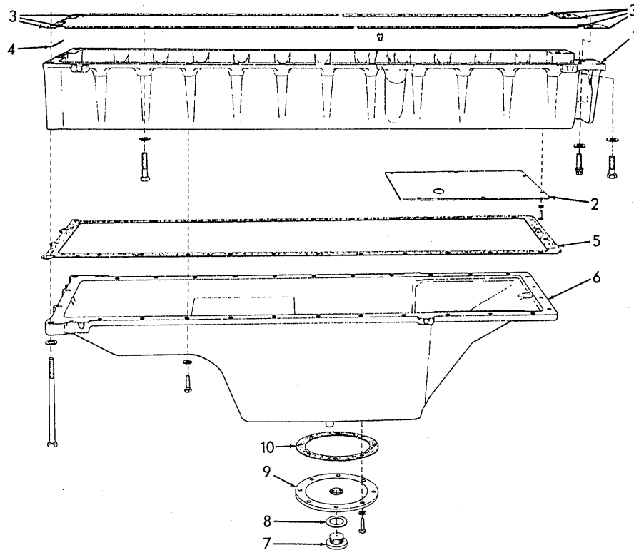
OIL PAN
