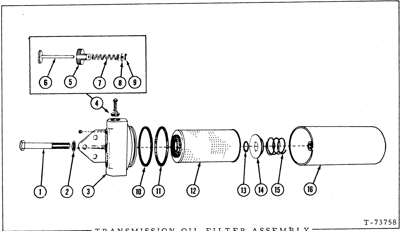
TRANSMISSION OIL FILTER ASSEMBLY
