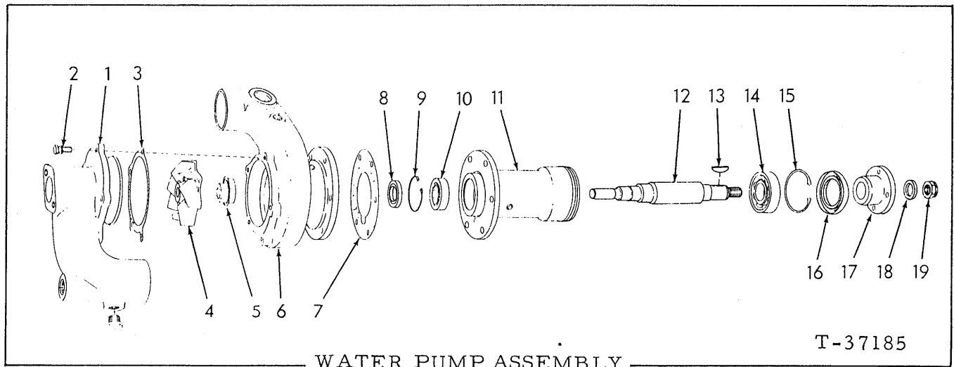
WATER PUMP ASSEMBLY
