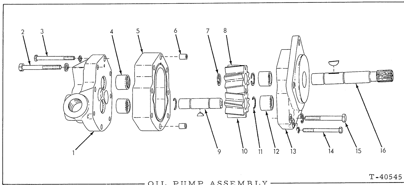
OIL PUMP ASSEMBLY
