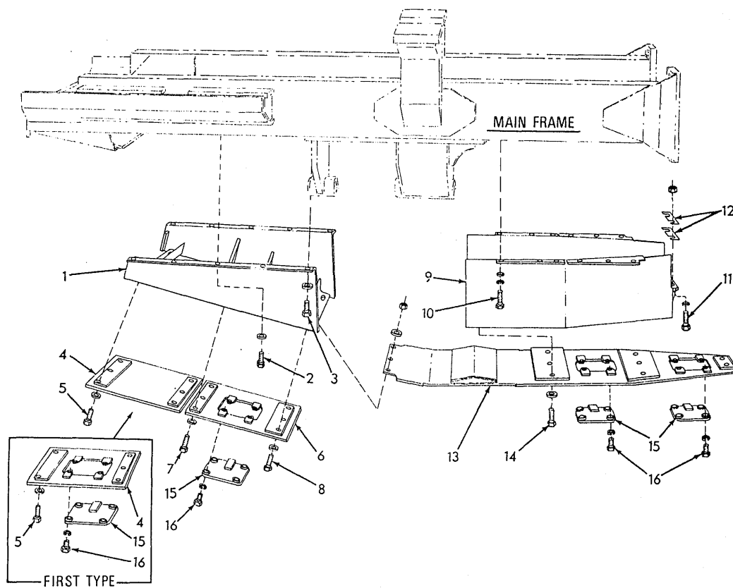
BOTTOM GUARDS
