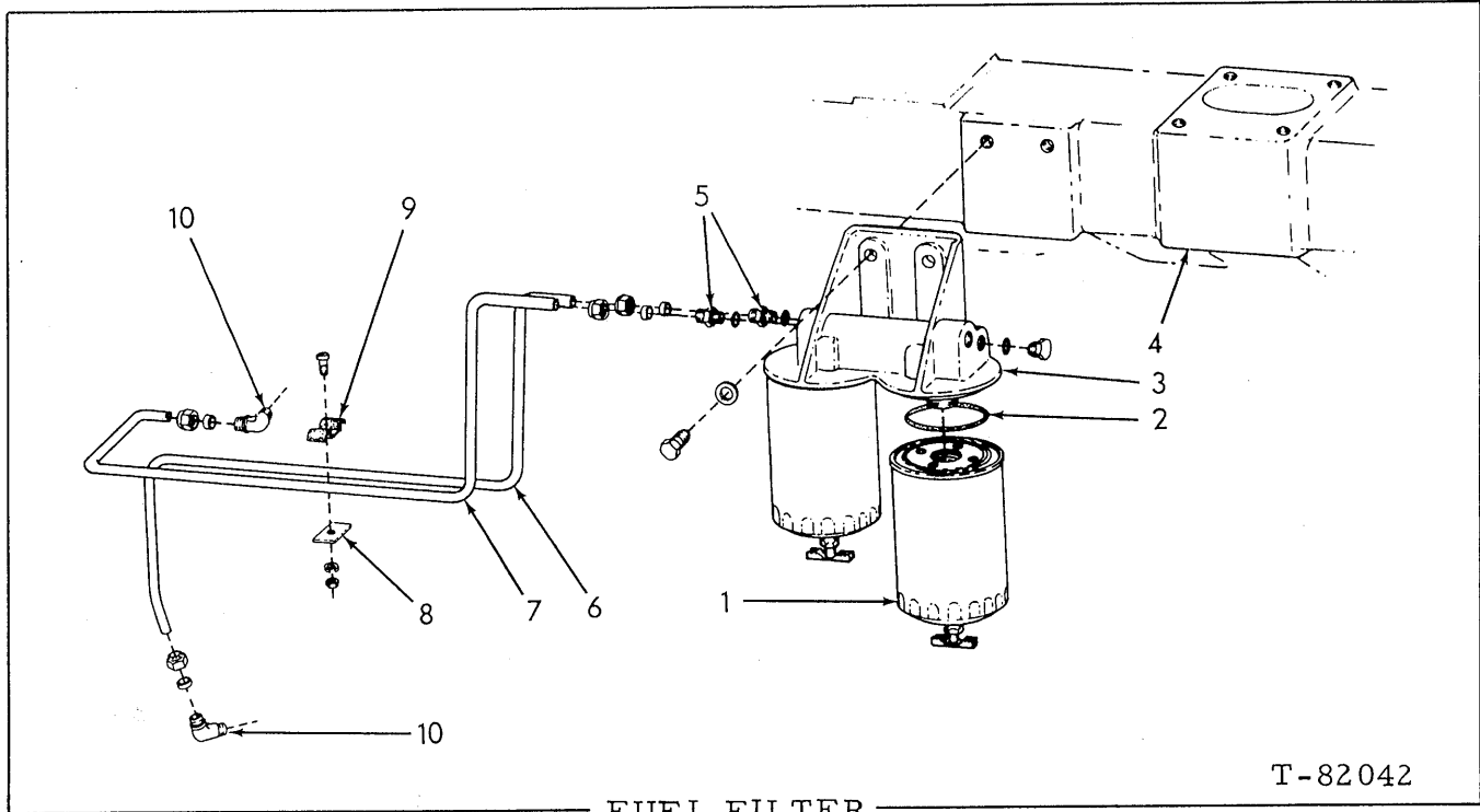
FUEL FILTER
