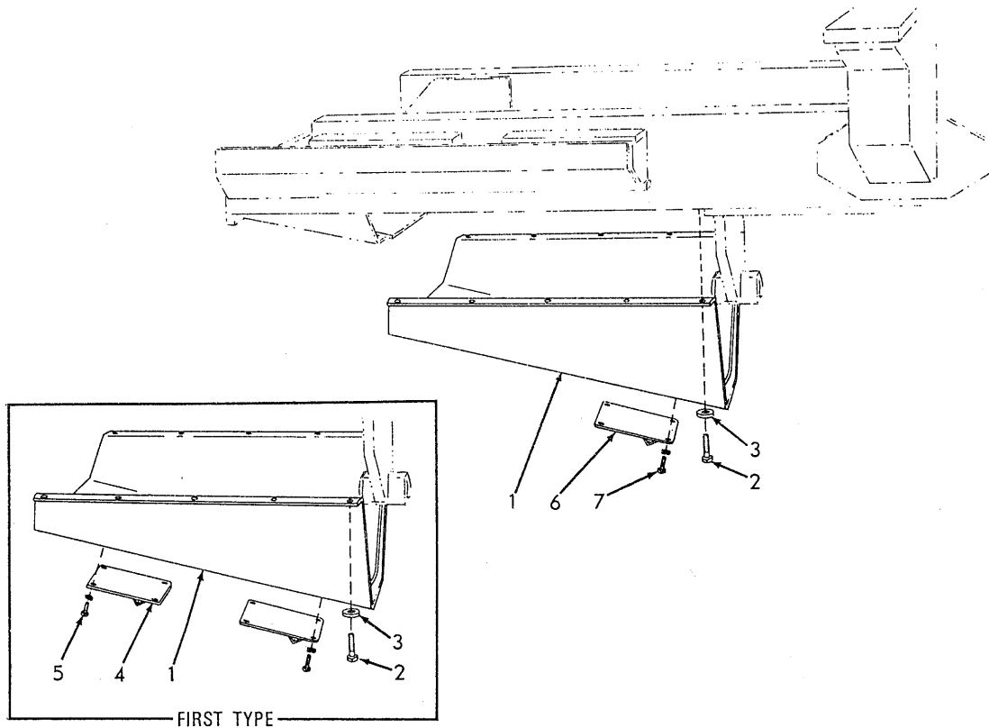
CRANKCASE GUARD
