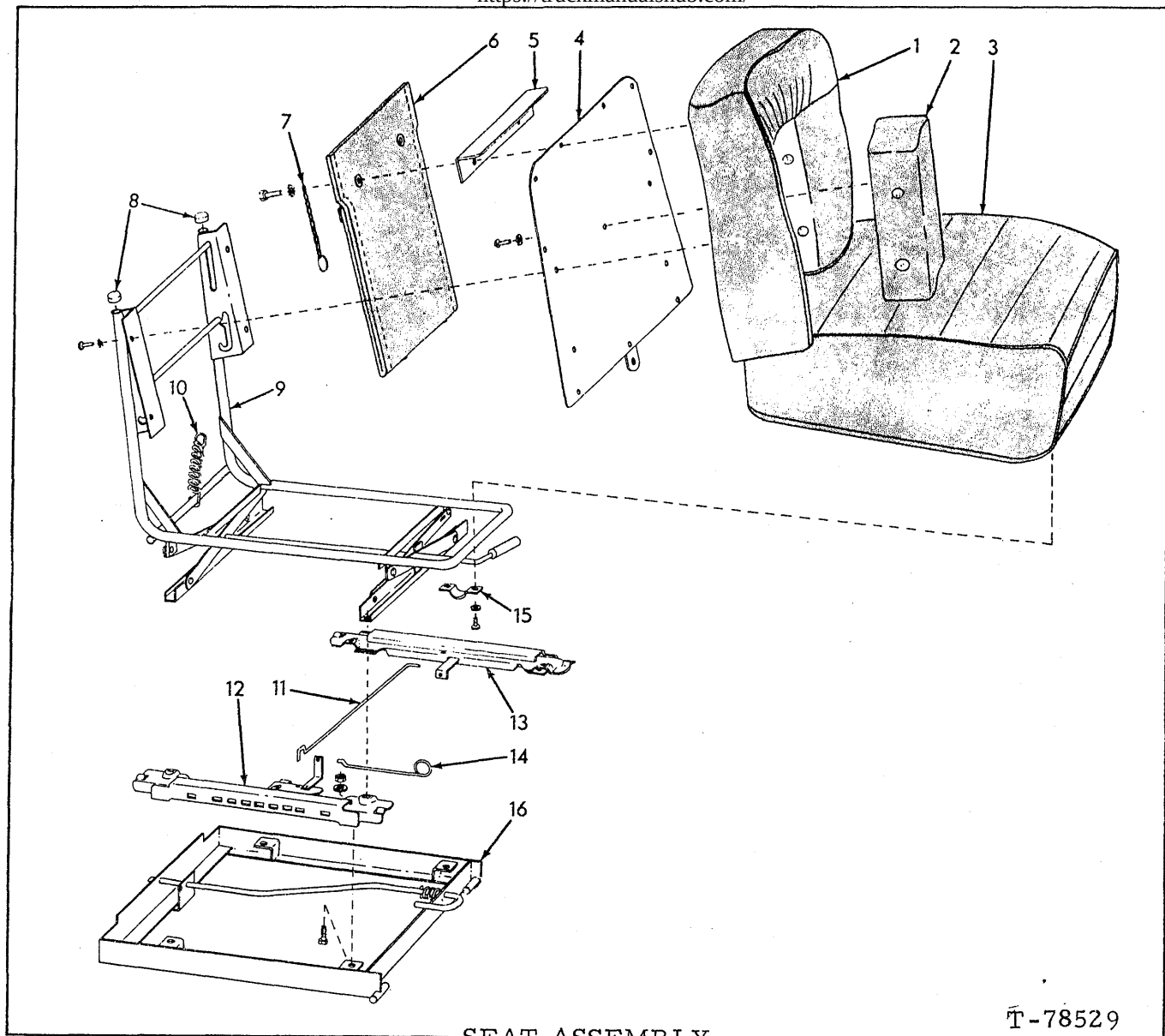
SEAT ASSEMBLY
