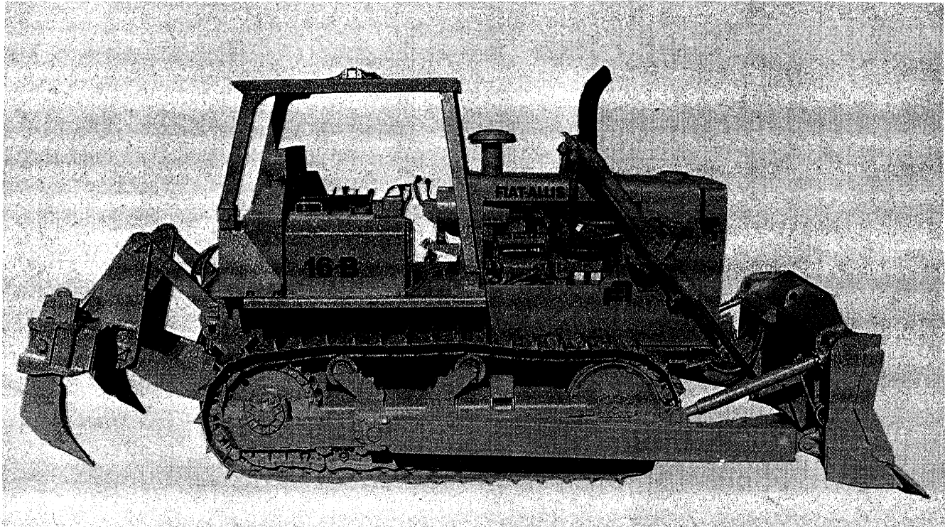
16-B (POWER SHIFT) CRAWLER TRACTOR (W/16HS DOZER AND 16R RIPPER)
