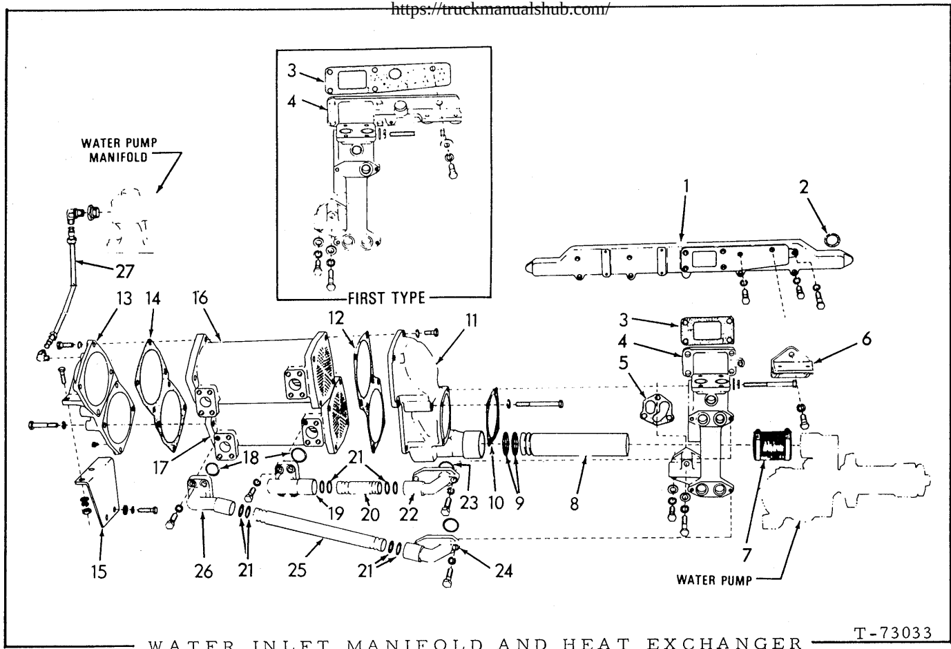
WATER INLET MANIFOLD AND HEAT EXCHANGER
