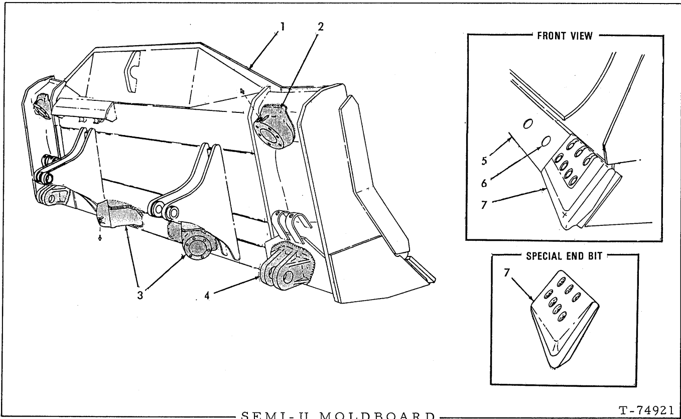
SEMI-U MOLDBOARD
