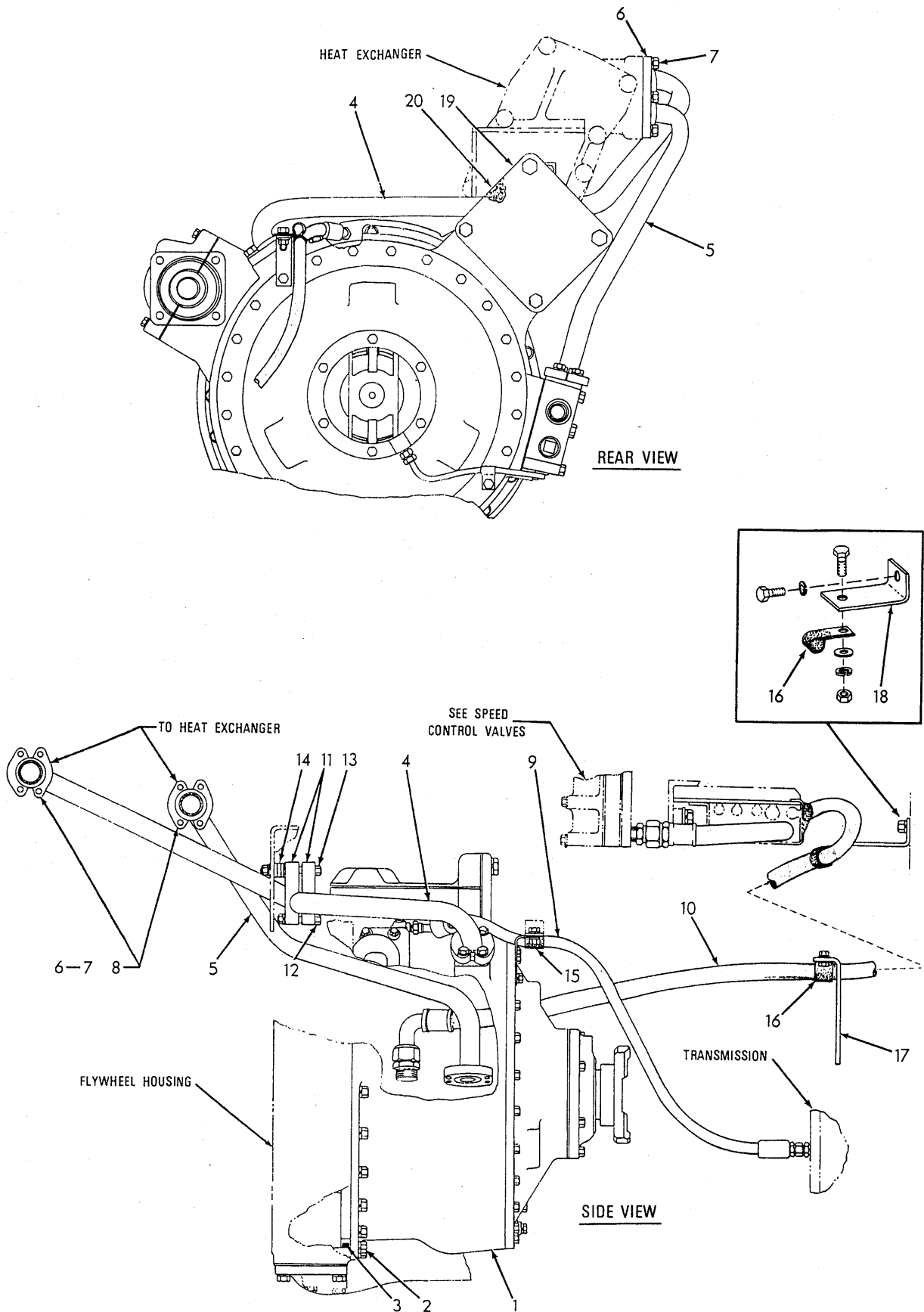
TORQUE CONVERTER LINES
