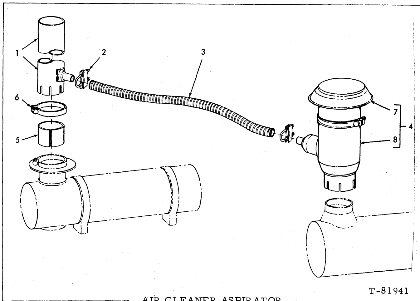
AIR CLEANER ASPIRATOR
