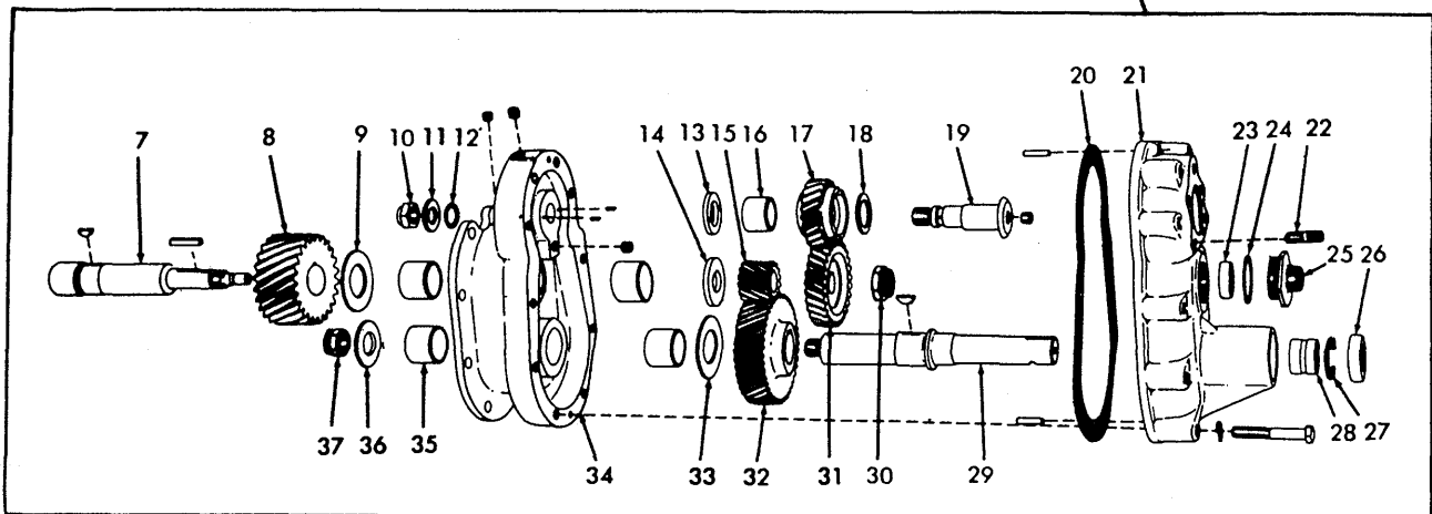
ACCESSORY DRIVE
