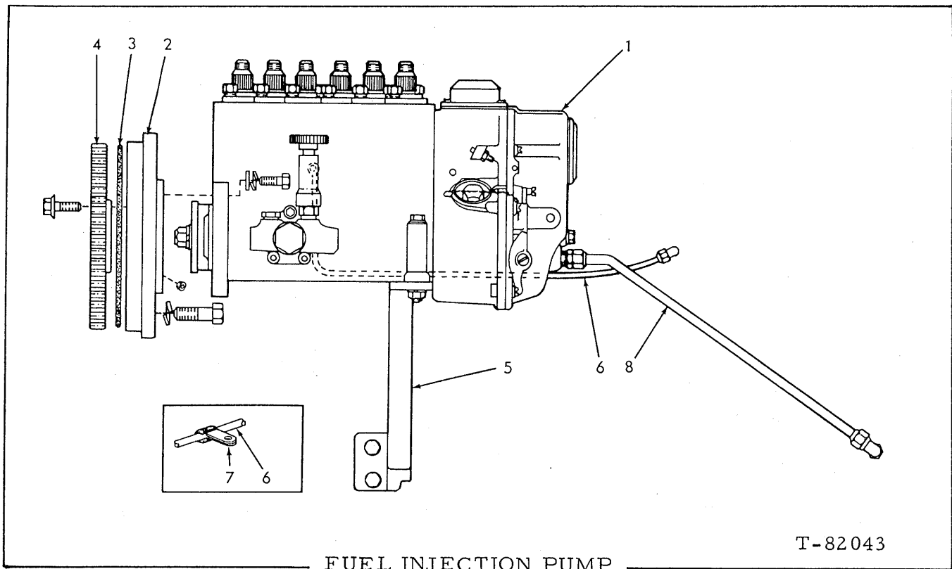
FUEL INJECTION PUMP
