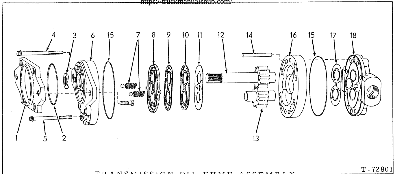
TRANSMISSION OIL PUMP ASSEMBLY
