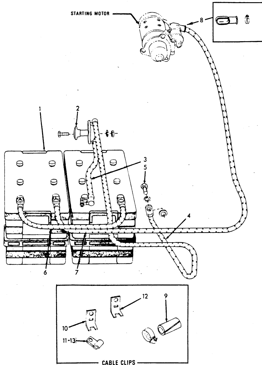
BATTERIES AND CABLES
