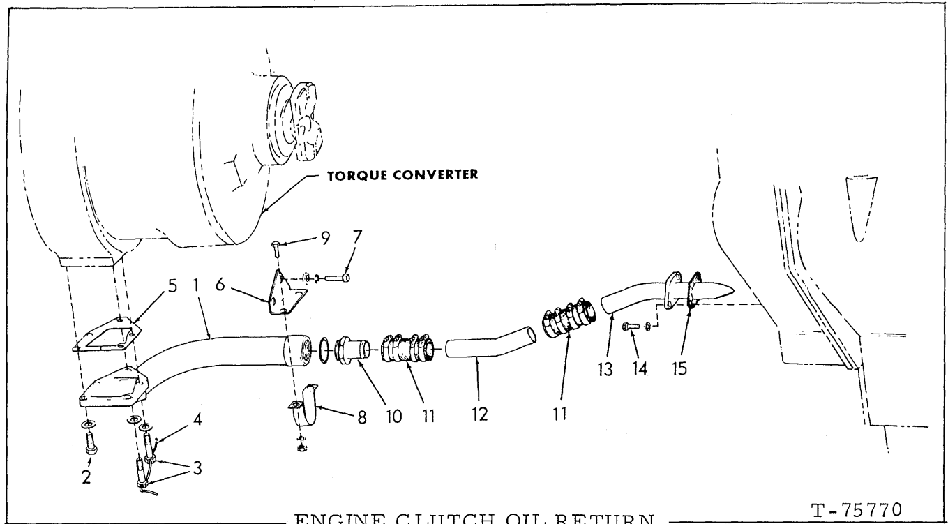
ENGINE CLUTCH OIL RETURN
