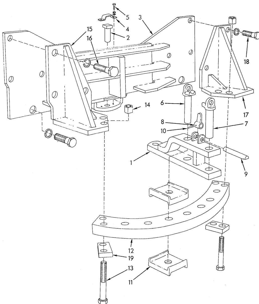
SWINGING DRAWBAR
