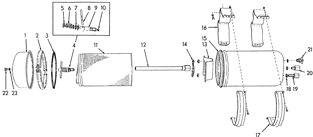
LUBER-FINER DESIGN
