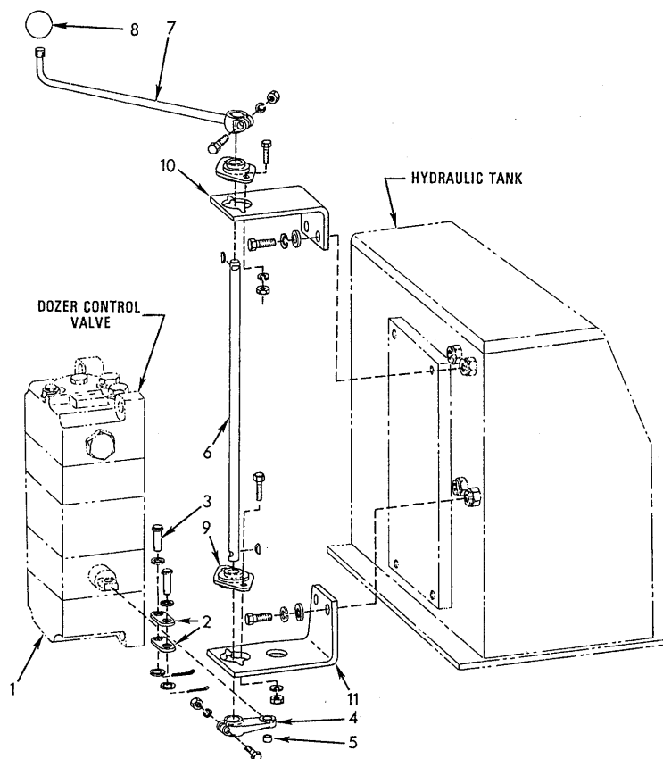
AUXILIARY VALVE CONTROL
