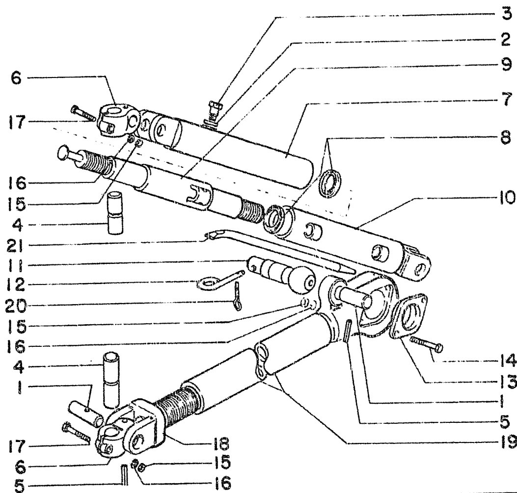
HYDRAULIC ANGLEDOZER
