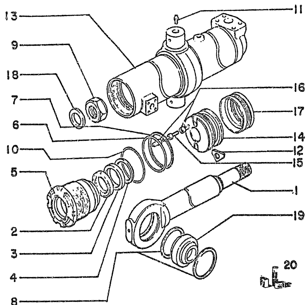
+-----+ | LIFTING CYLINDER (ANGLED OZER - BULLDOZER) | +-----+
