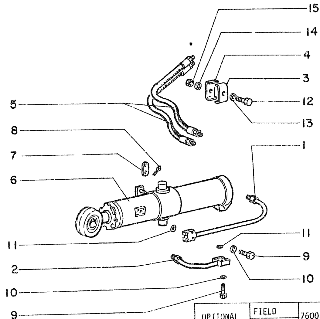
LIFTING CYLINDER ALL HYDRAULIC
