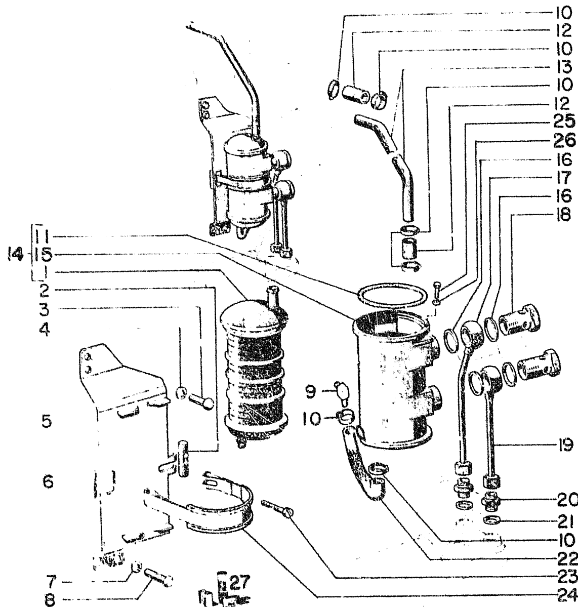
ENGINE OIL HEAT EXCHANGER - INTERCAMBIADOR OLEO DO MOTOR
