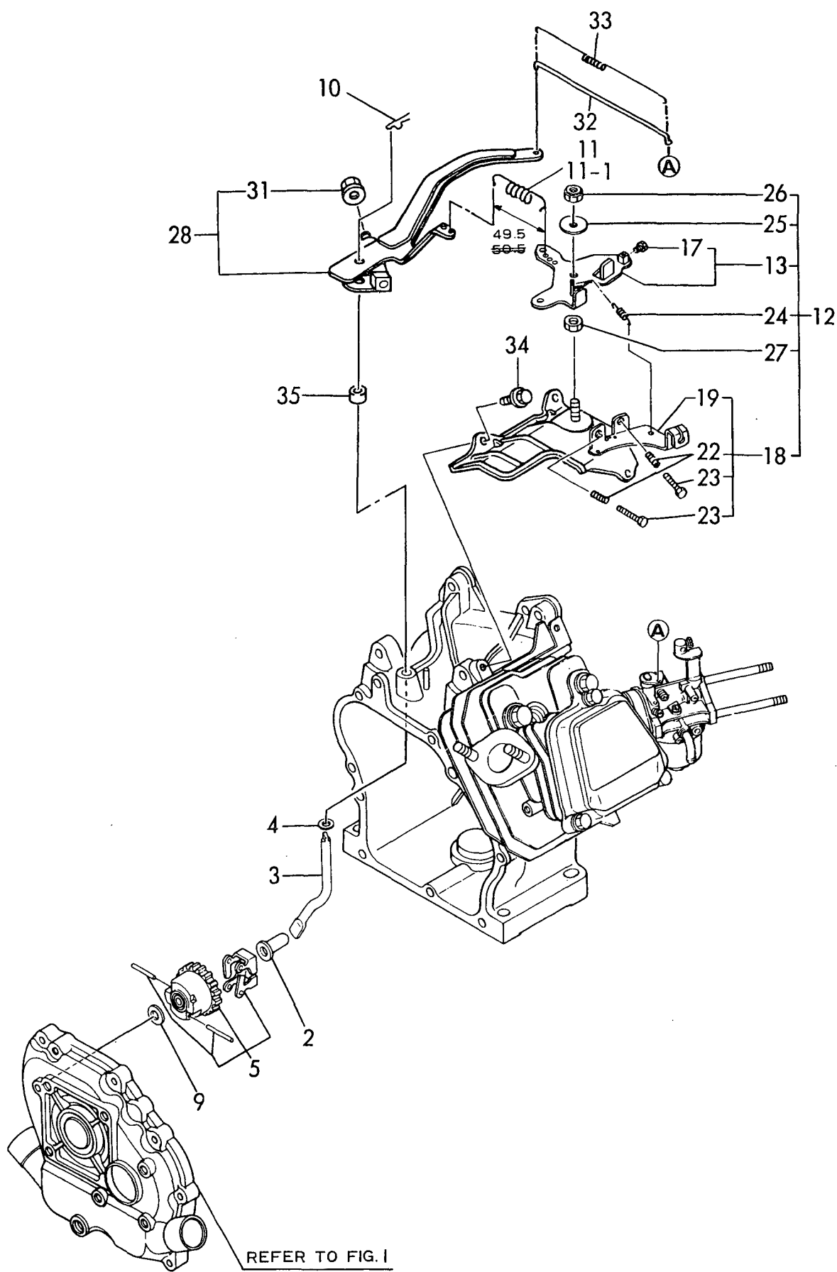
Fig. 7 ガバナ&操縦装置 GOVERNOR & CONTROL DEVICE
