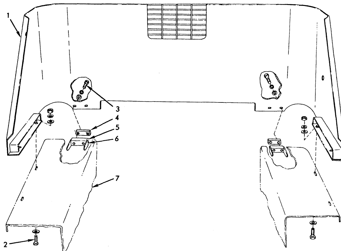
FUEL TANK AND SEAT GUARD
