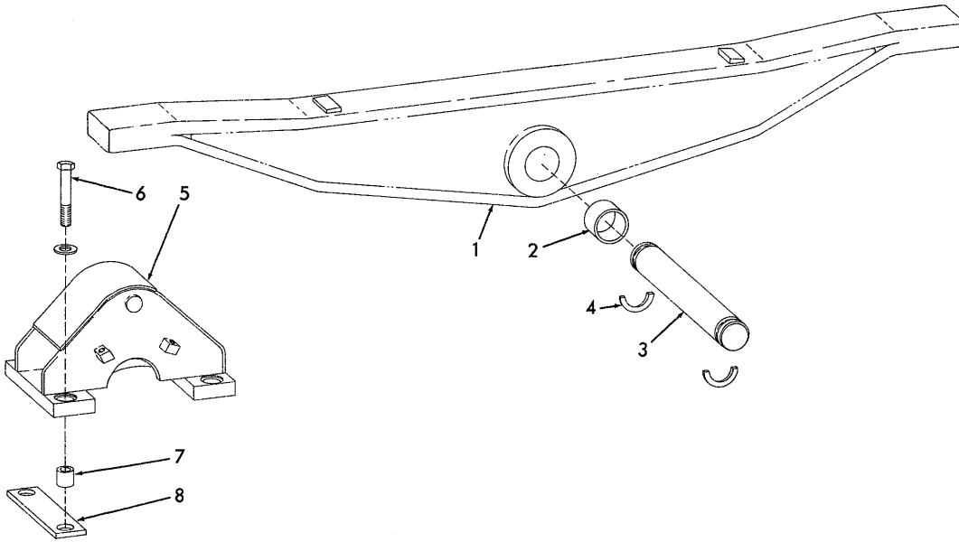
EQUALIZING BEAM
