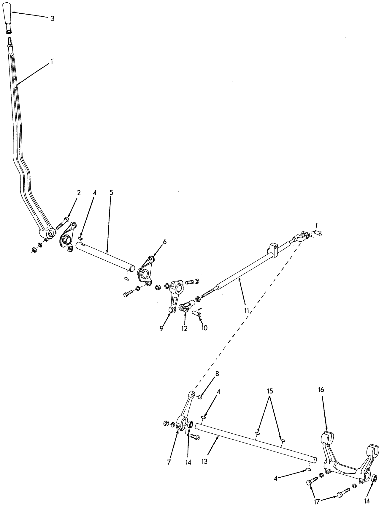
ENGINE CLUTCH CONTROL
