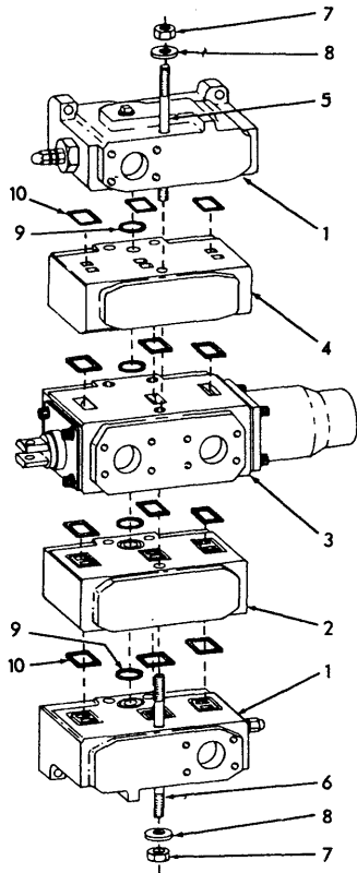
VALVE ASSY. 70660647, 70686090, 73110106
