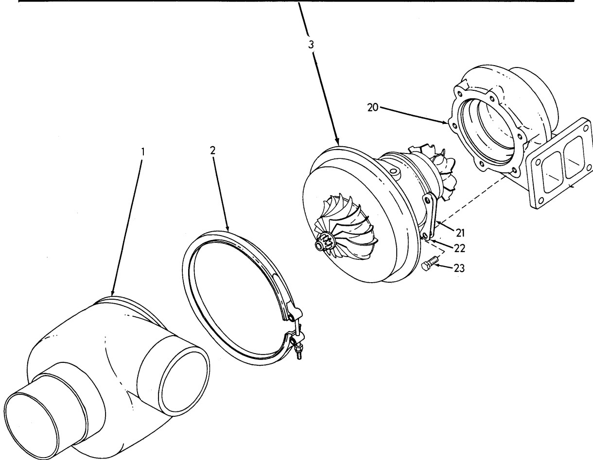
TURBOCHARGER ASSEMBLY
