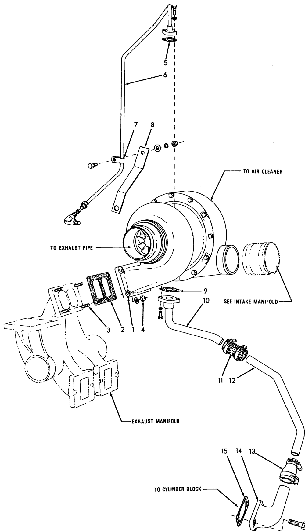
TURBOCHARGER CONNECTIONS
