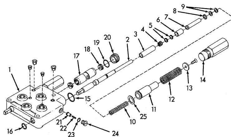
CONTROL VALVE ASSEMBLY
