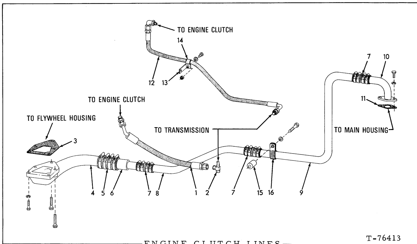
ENGINE CLUTCH LINES
