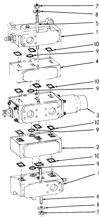
CONTROL VALVE
