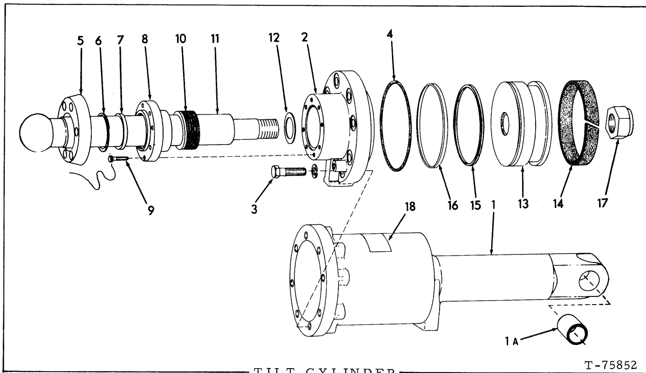
TILT CYLINDER
