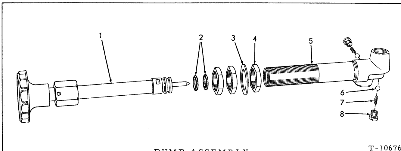
PUMP ASSEMBLY
