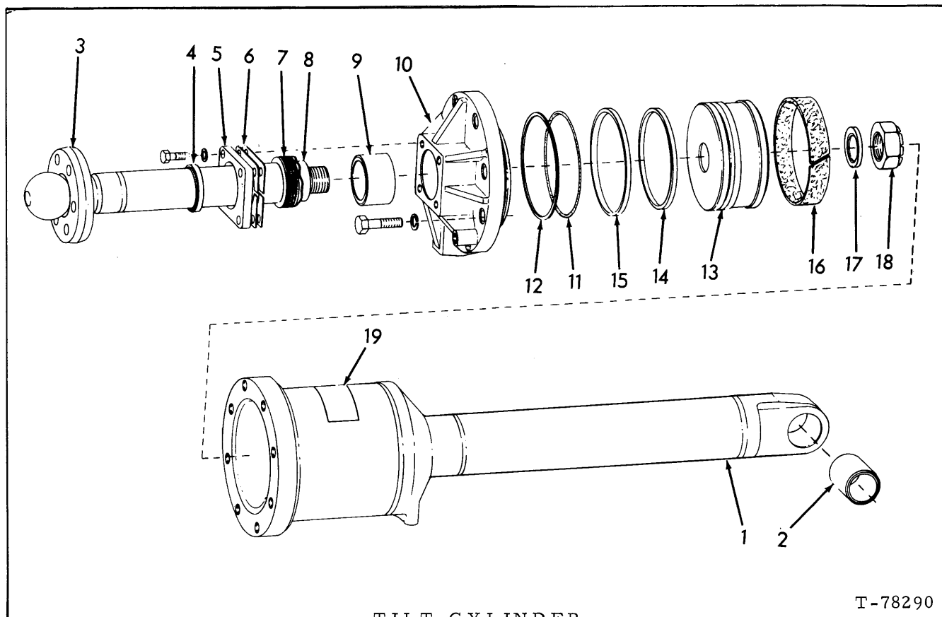
TILT CYLINDER
