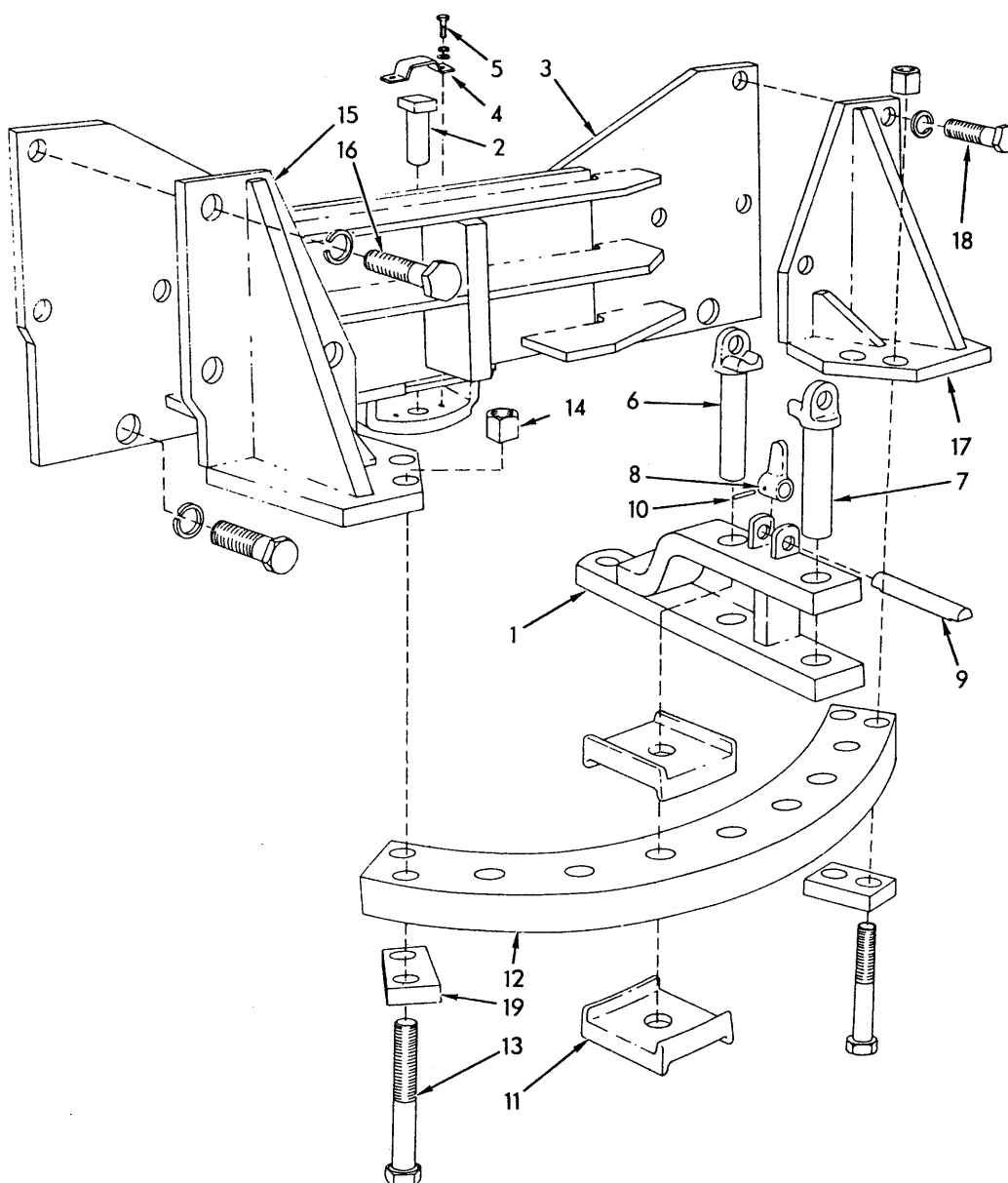
SWINGING DRAWBAR
