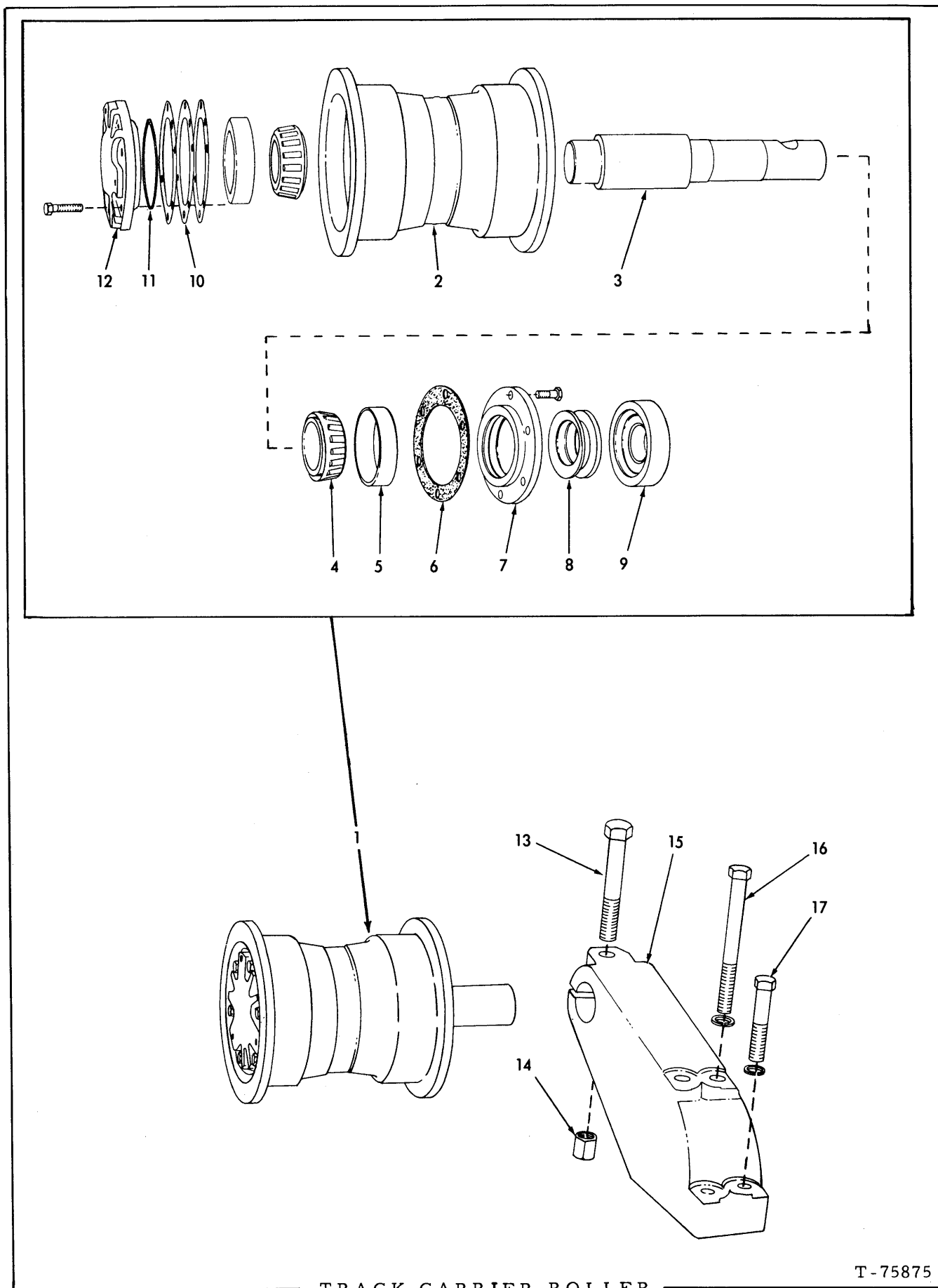
TRACK CARRIER ROLLER
