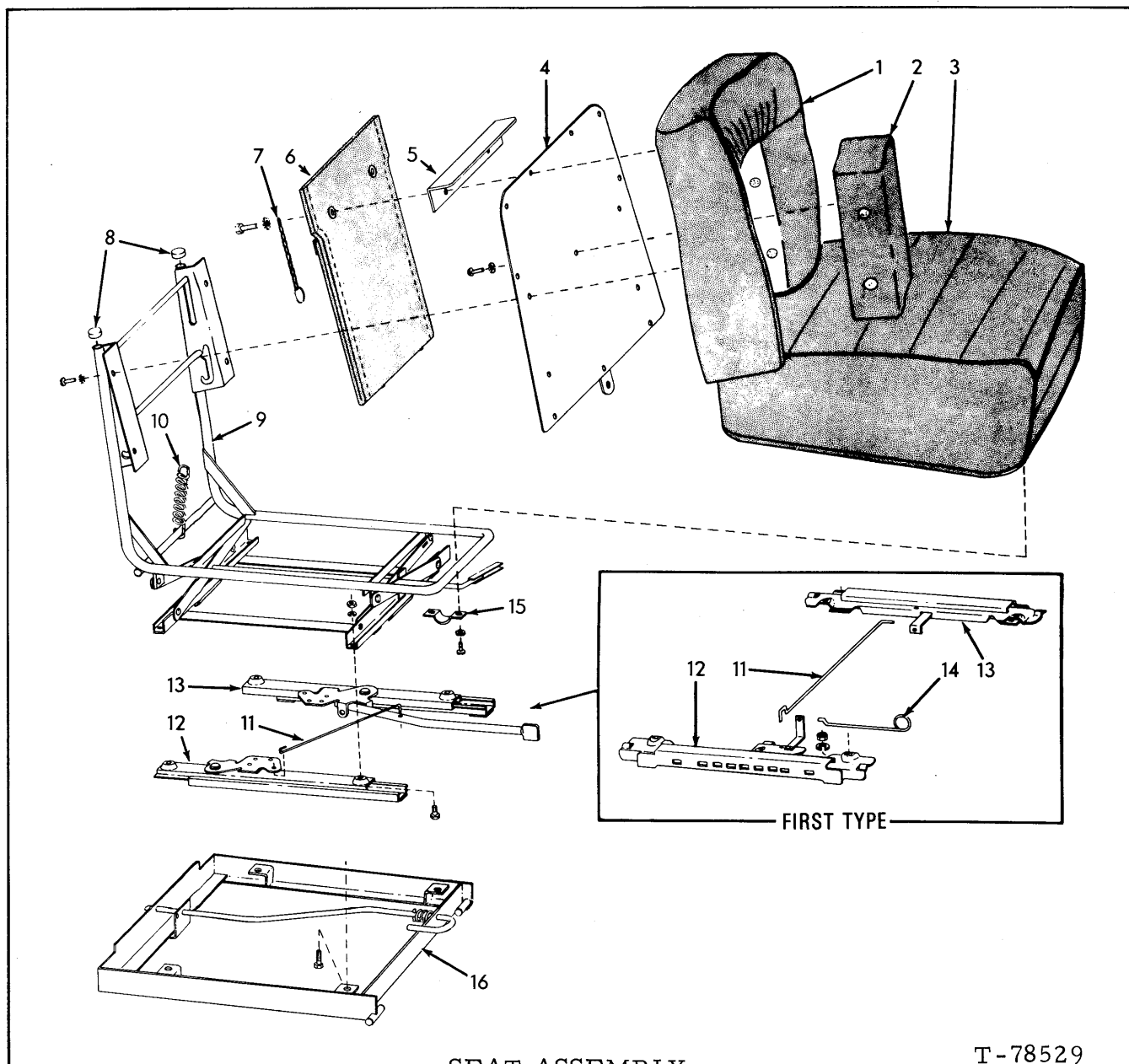
SEAT ASSEMBLY
