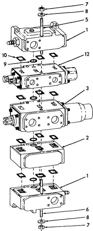
VALVE ASSY. 70665121
