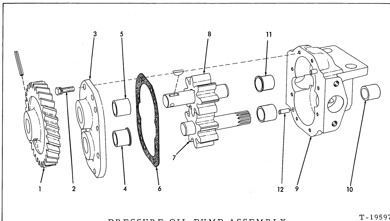
PRESSURE OIL PUMP ASSEMBLY
