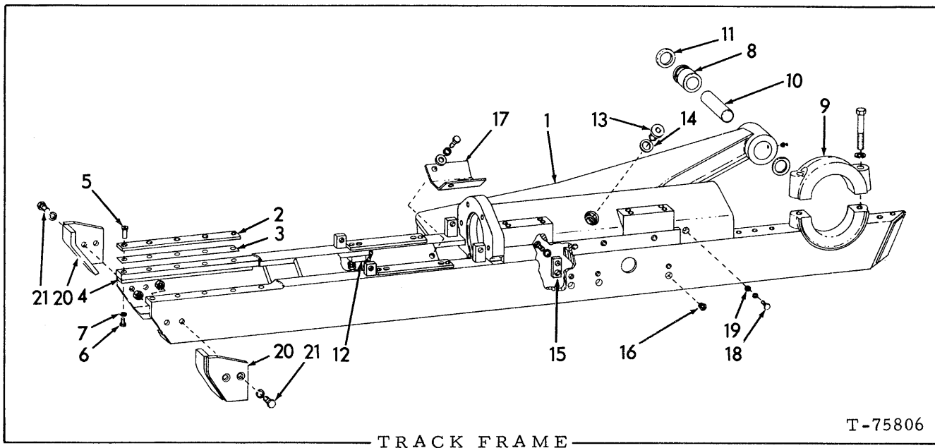
TRACK FRAME
