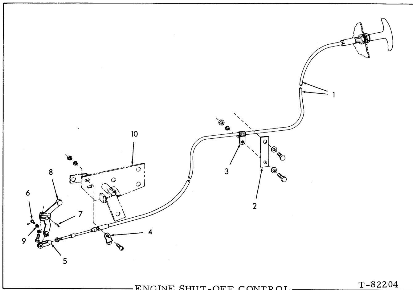
ENGINE SHUT-OFF CONTROL
