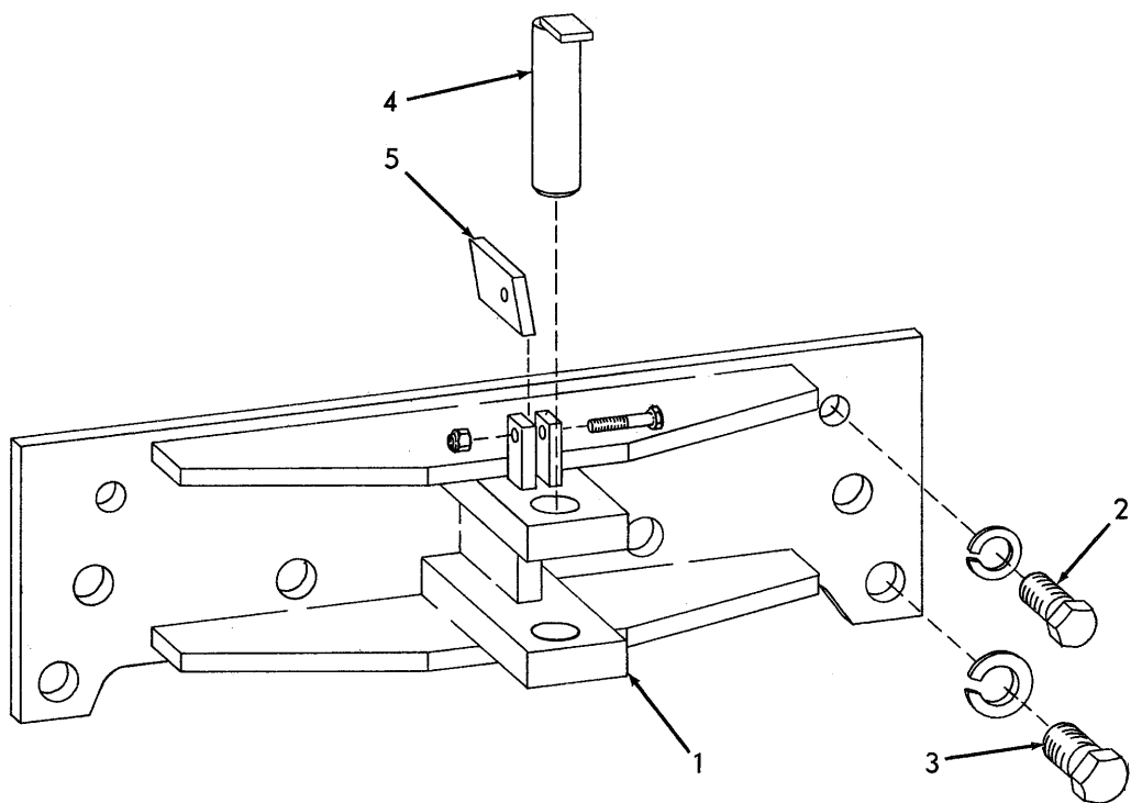
— FIXED DRAW BAR —
