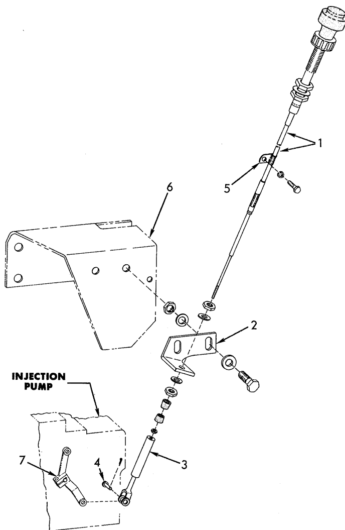
ENGINE SHUT-OFF CONTROL
