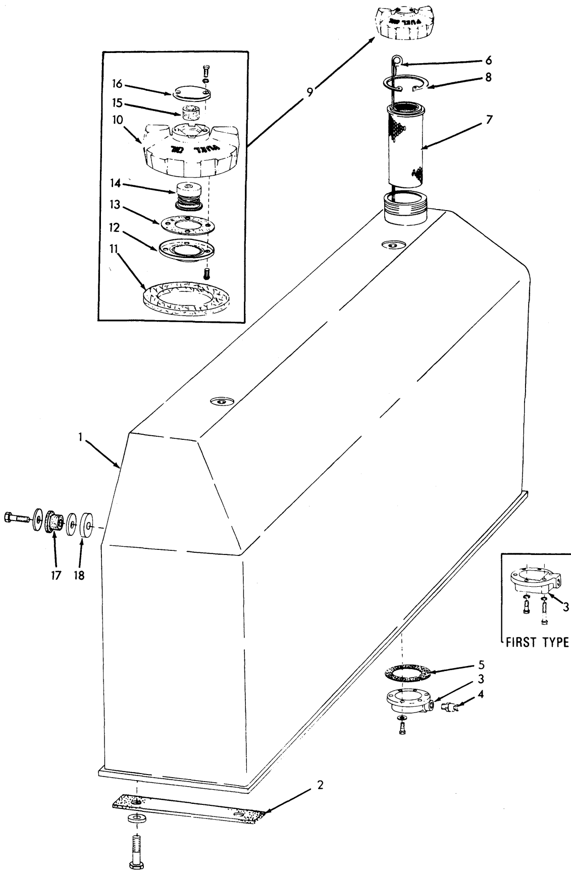
FUEL TANK
