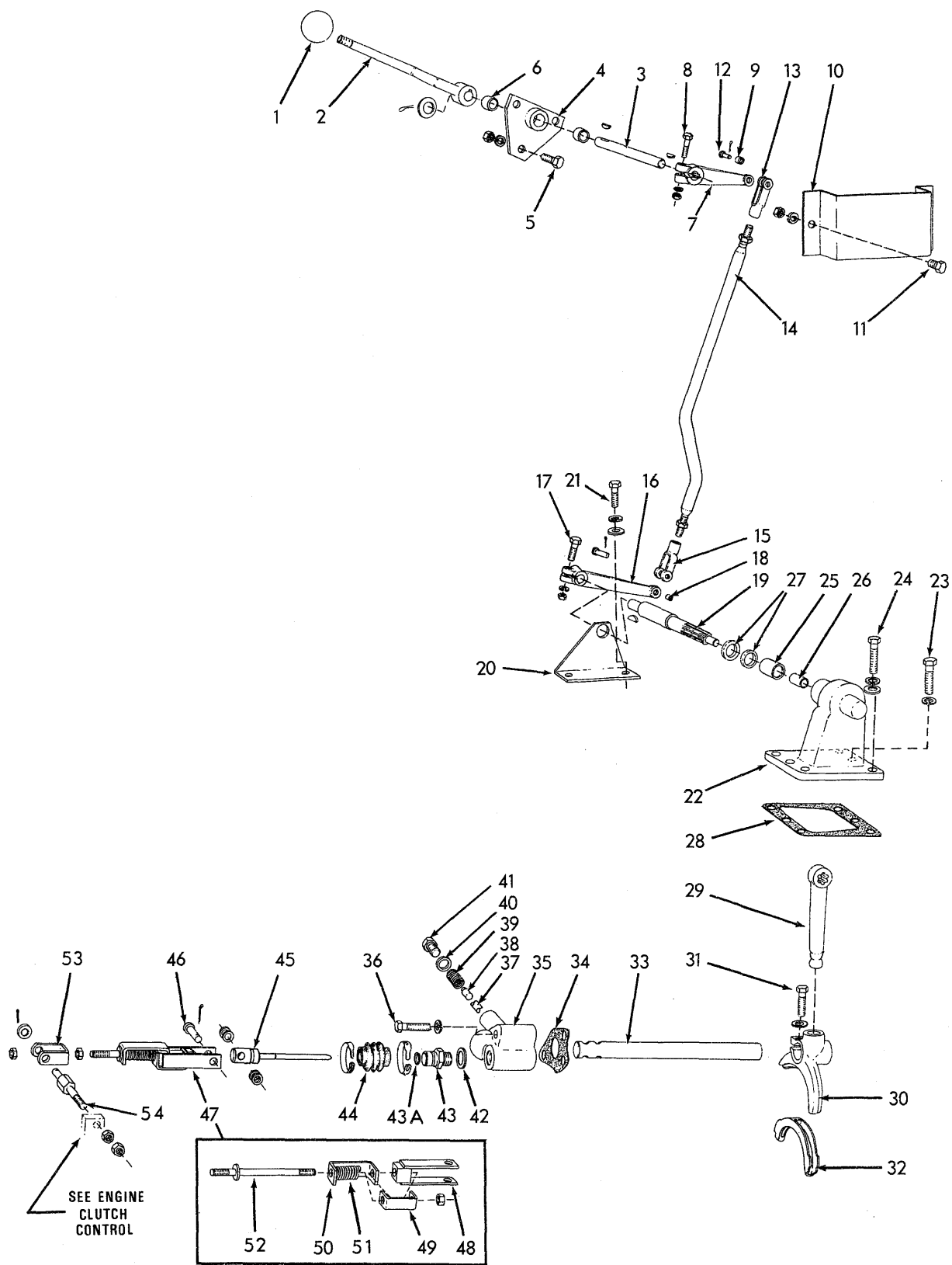
FORWARD HIGH-LOW GEAR SHIFT
