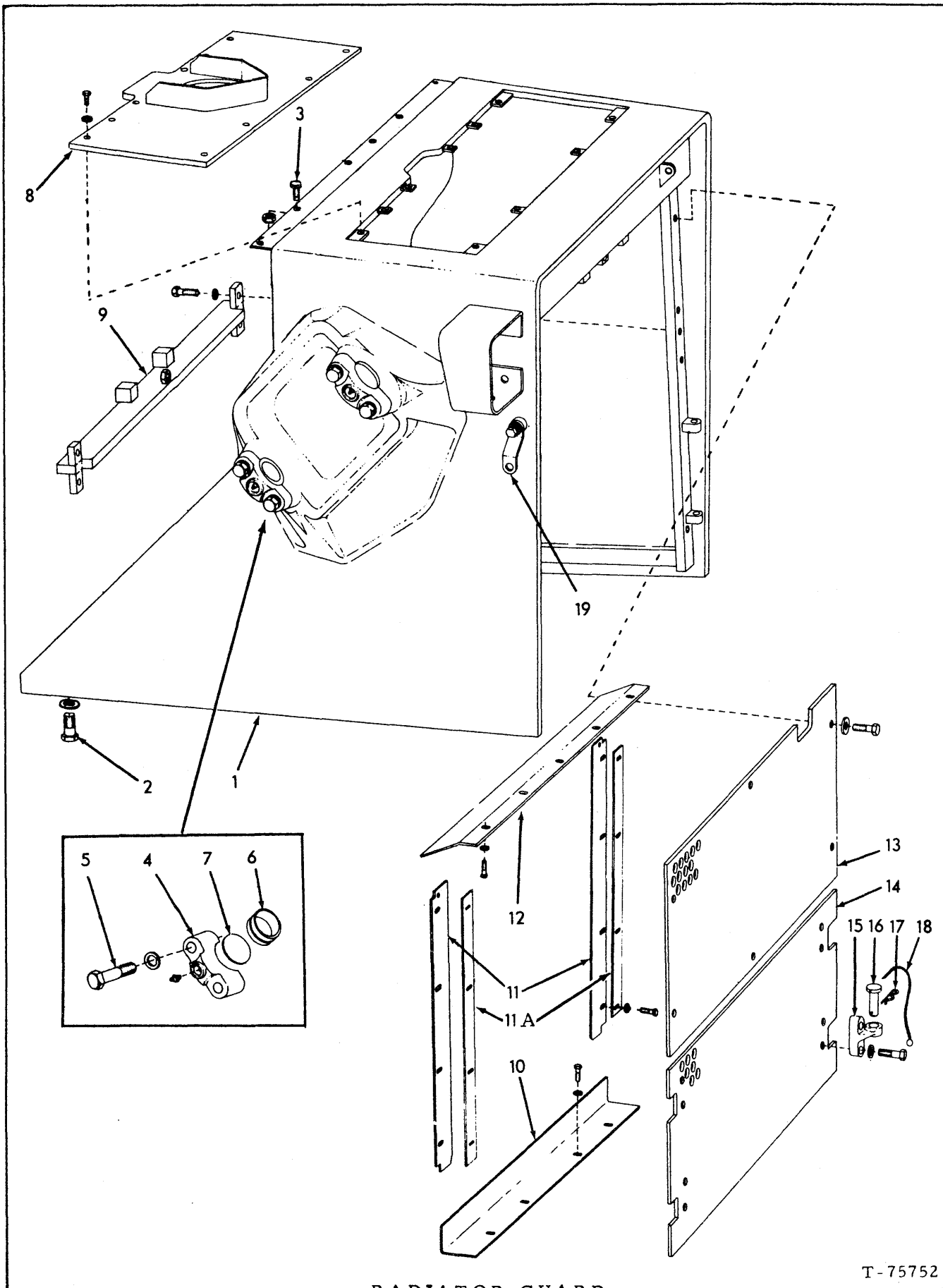
RADIATOR GUARD
