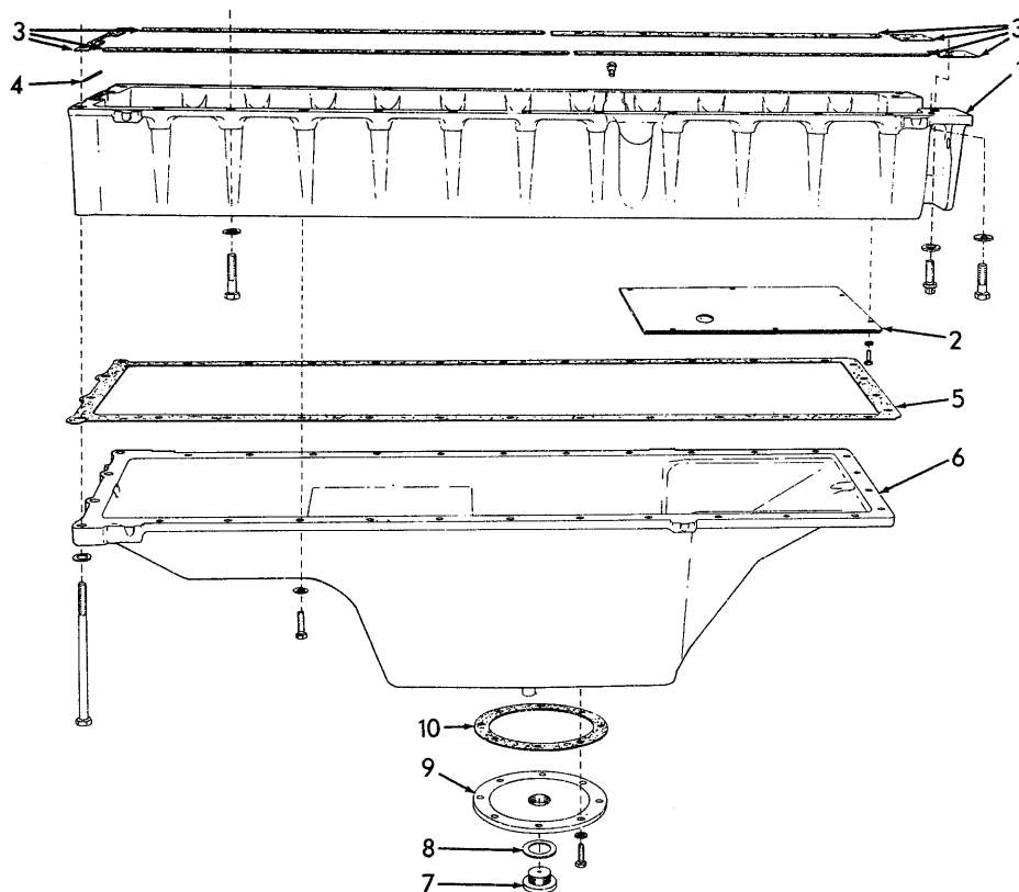
OIL PAN
