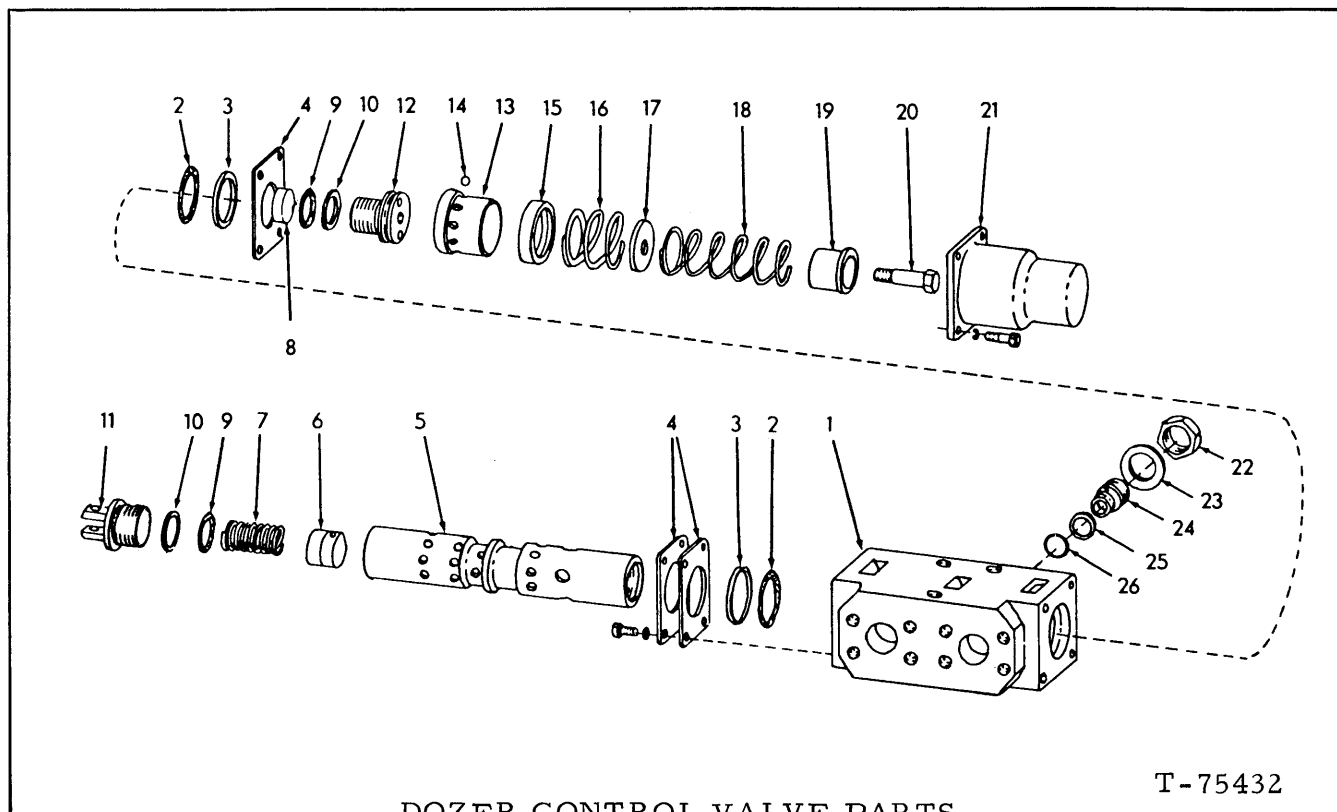
DOZER CONTROL VALVE PARTS
