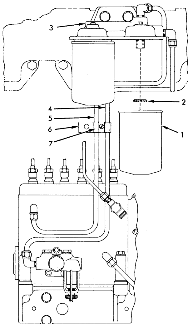
FUEL FILTER
