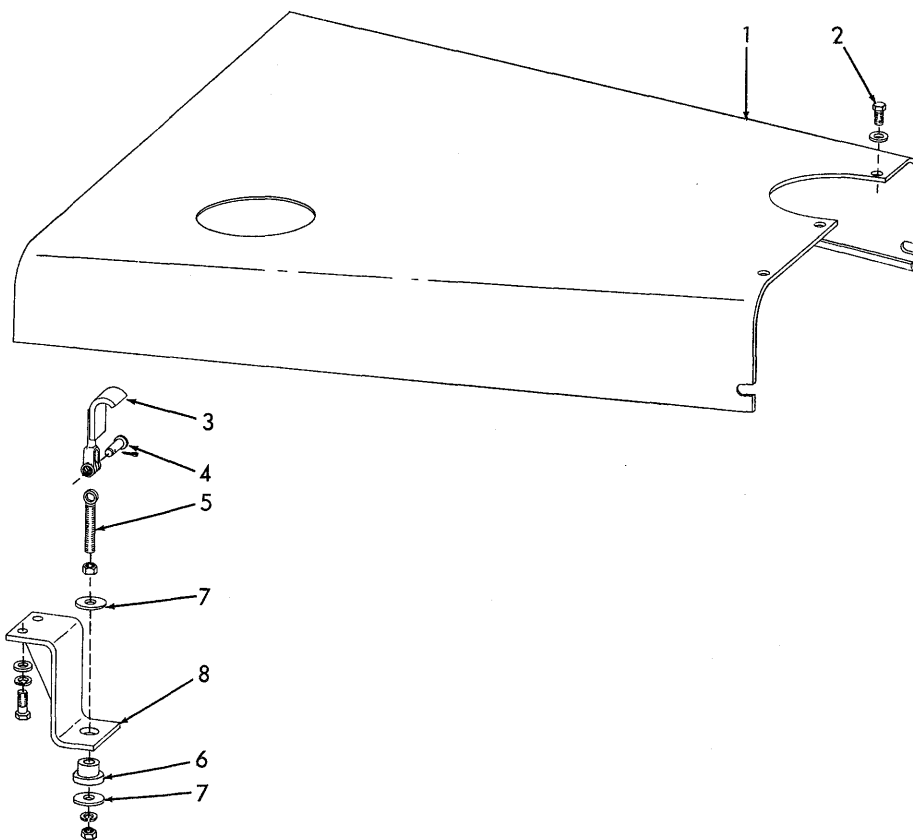
HOOD
