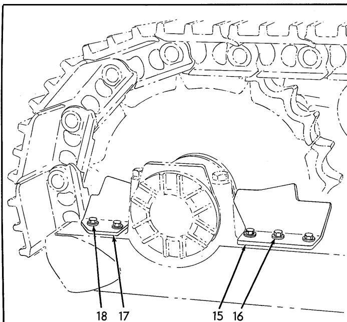
STANDARD SPROCKET GUARDS
