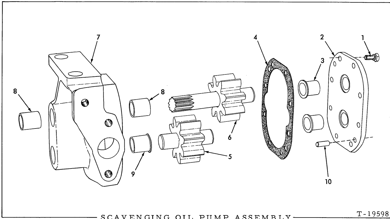
SCAVENGING OIL PUMP ASSEMBLY
