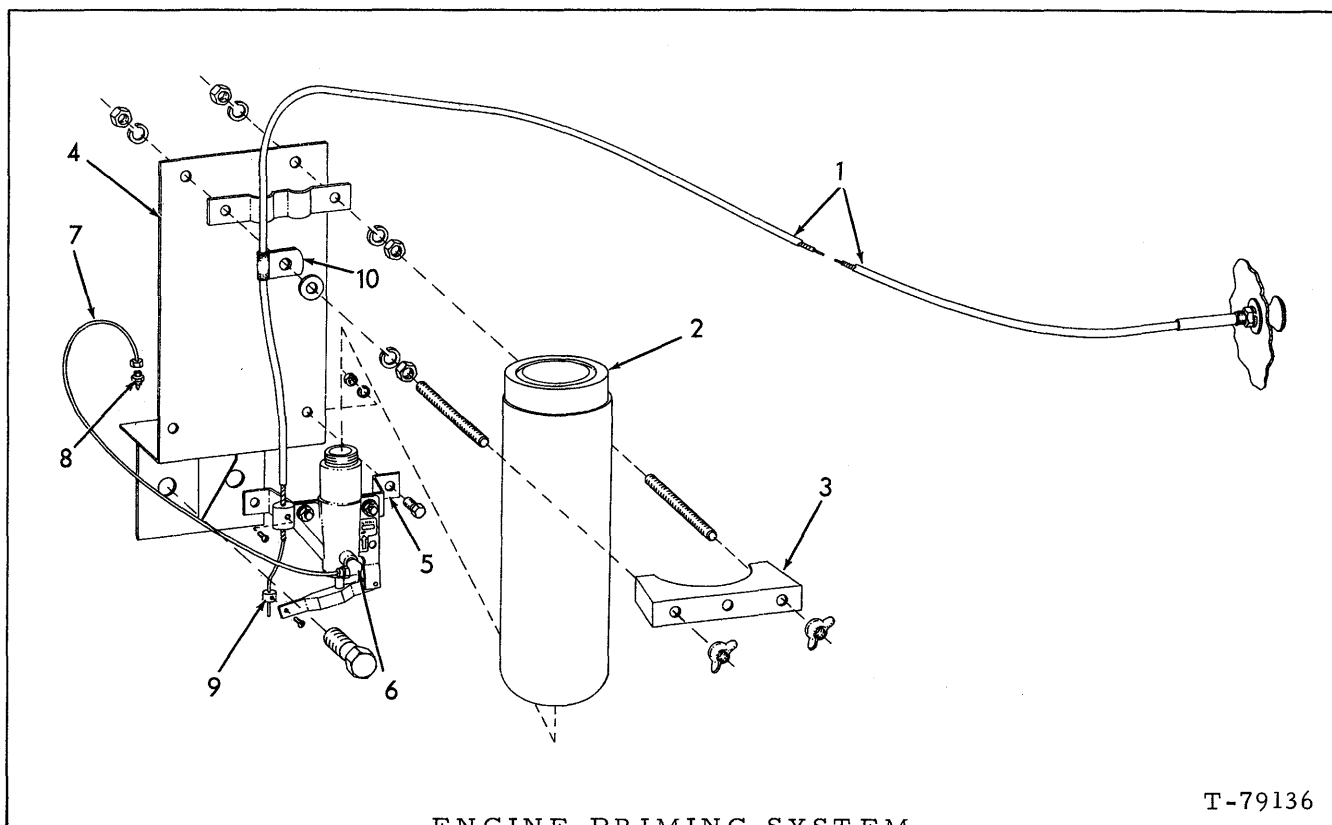
ENGINE PRIMING SYSTEM
