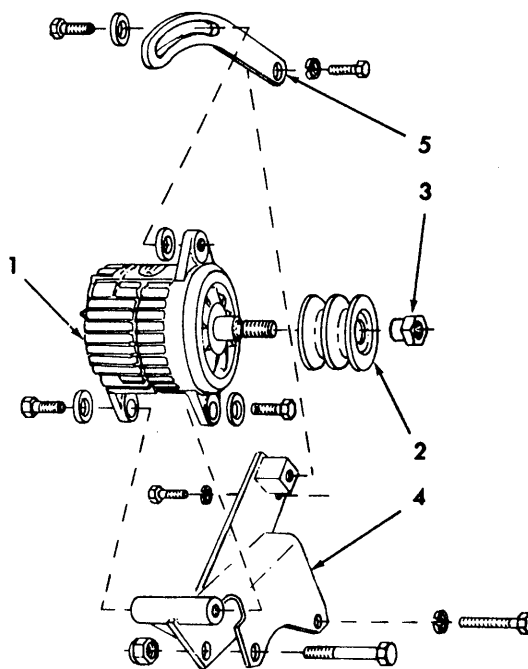
ALTERNATOR
