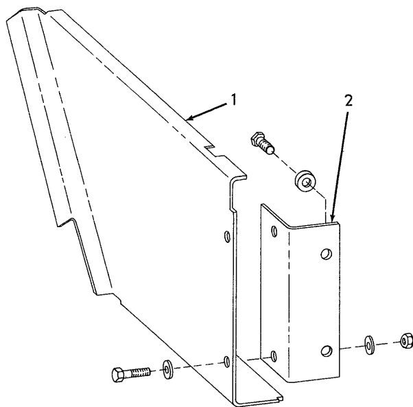
FRONT FENDERS
