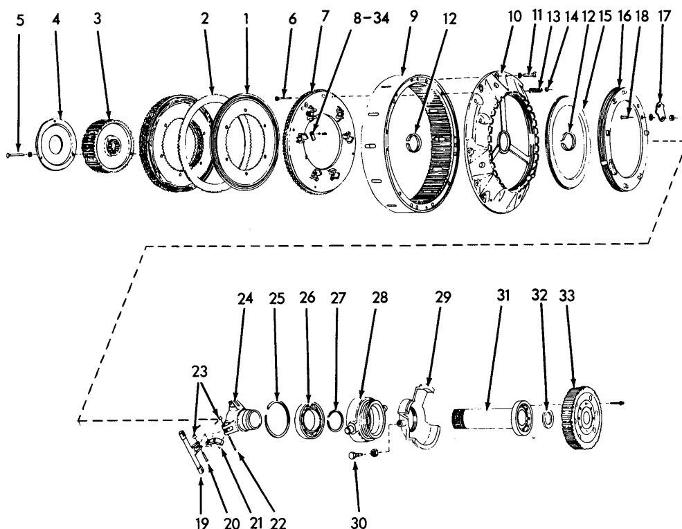
ENGINE CLUTCH PARTS
