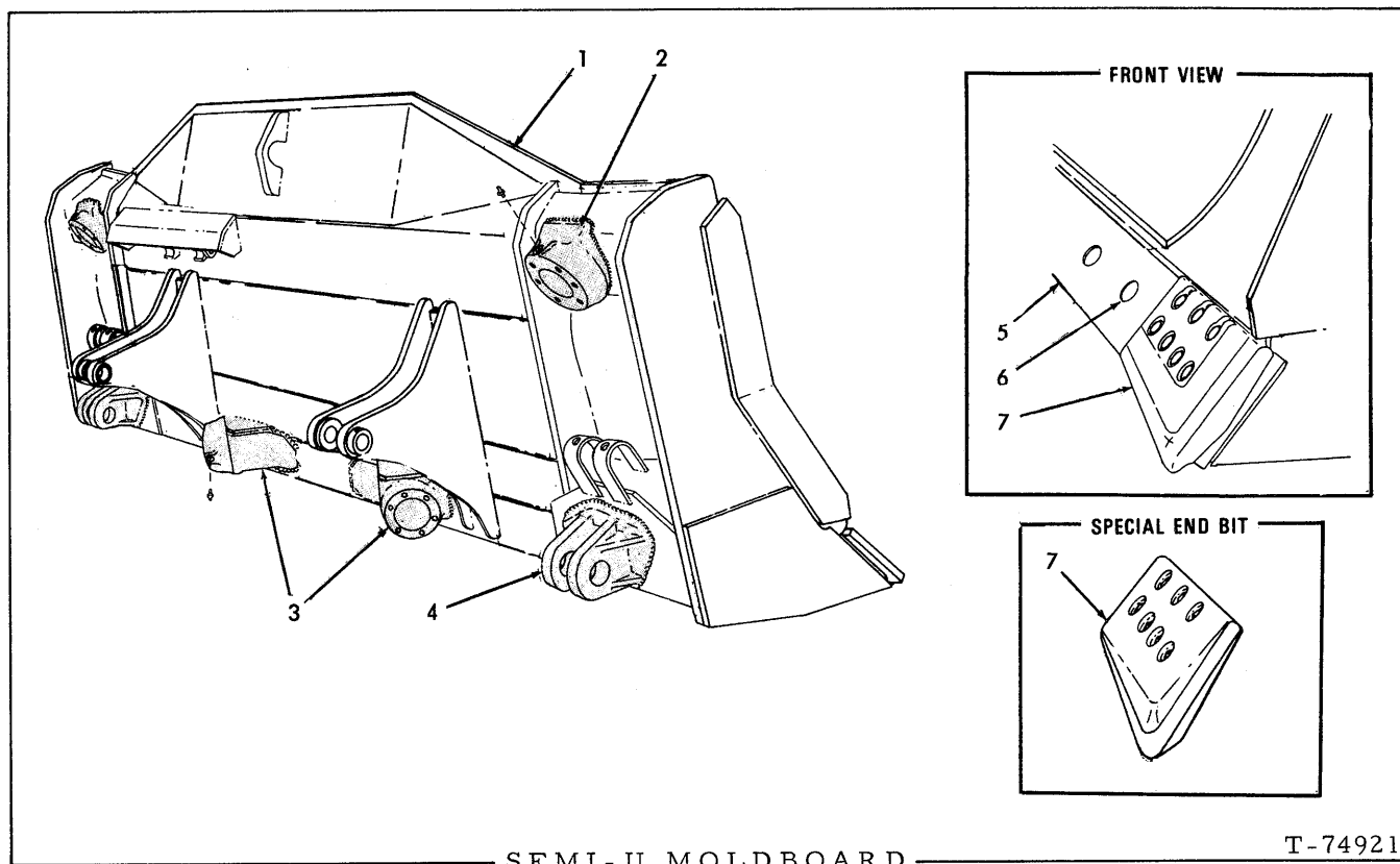
SEMI-U MOLDBOARD
