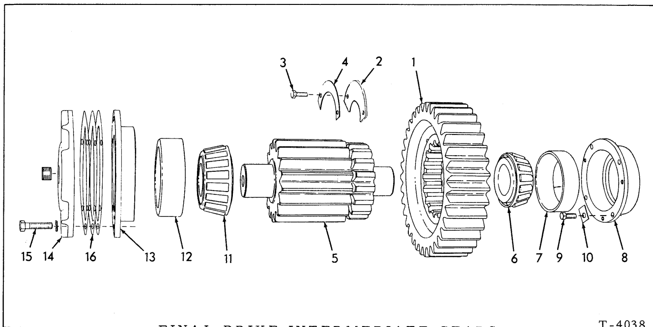
FINAL DRIVE INTERMEDIATE GEARS
