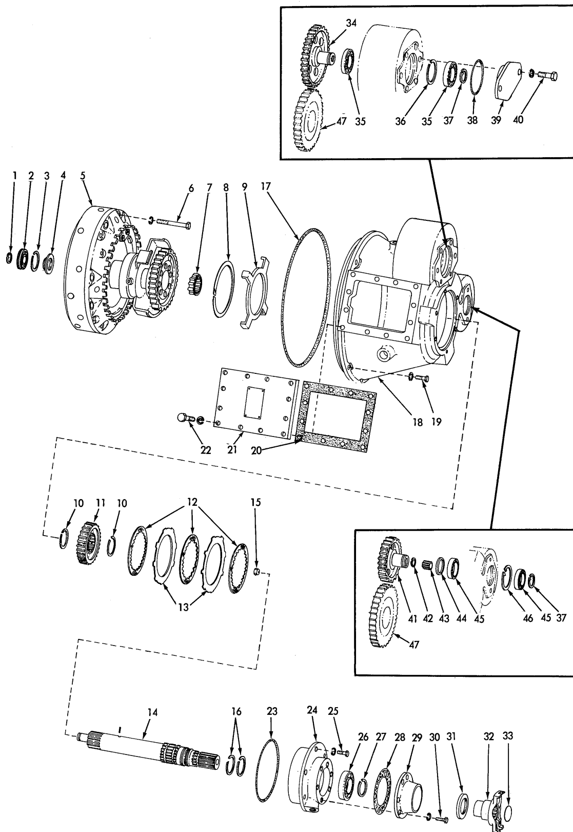
ENGINE CLUTCH AND HOUSING
