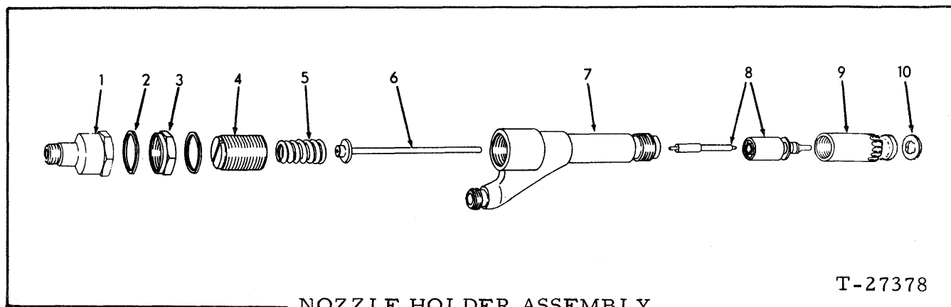
NOZZLE HOLDER ASSEMBLY
