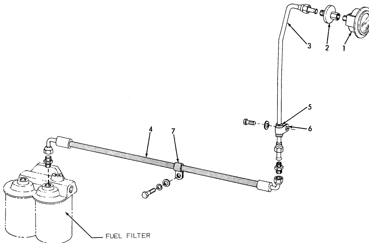
FUEL PRESSURE GAUGE
