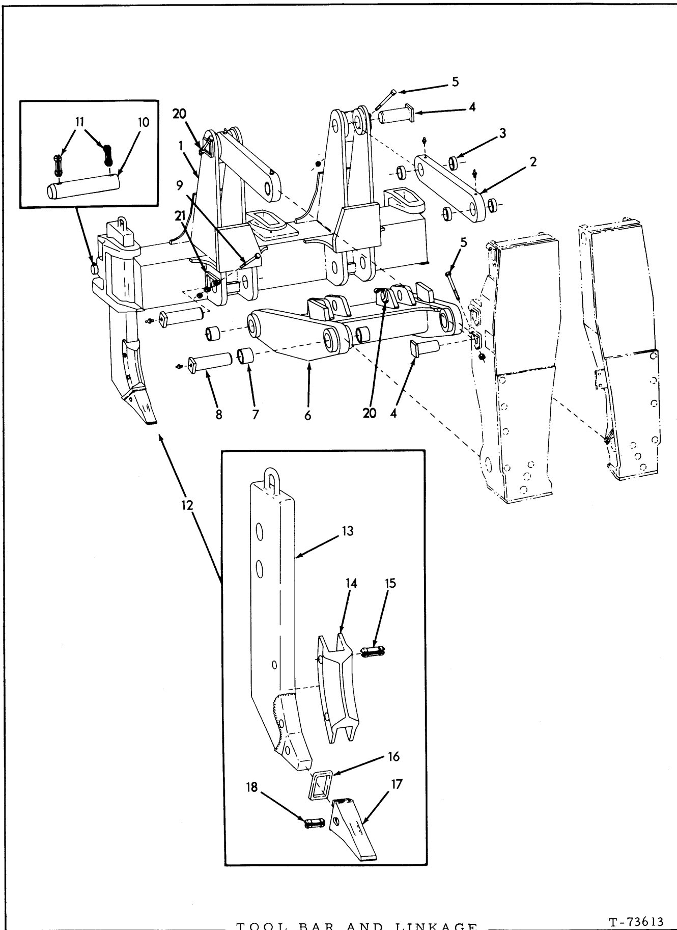
TOOL BAR AND LINKAGE
