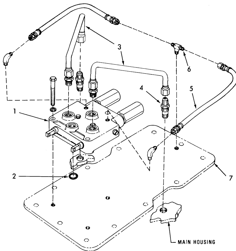
CONTROL VALVE LINES
