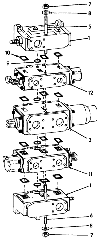
VALVE ASSY. 70662085, 70686070, 73110105
