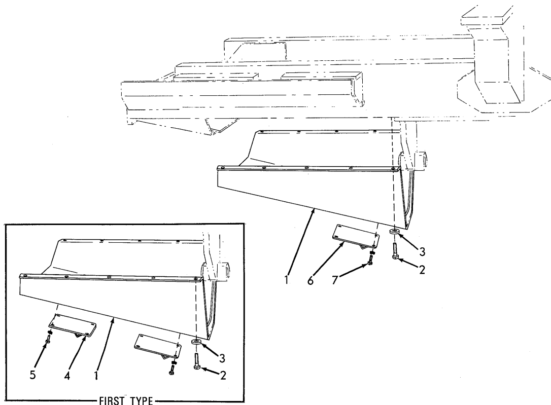
CRANKCASE GUARD
