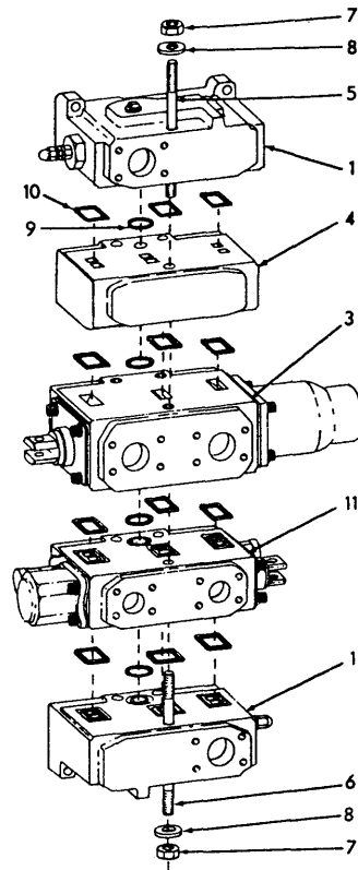
VALVE ASSY. 70665122
