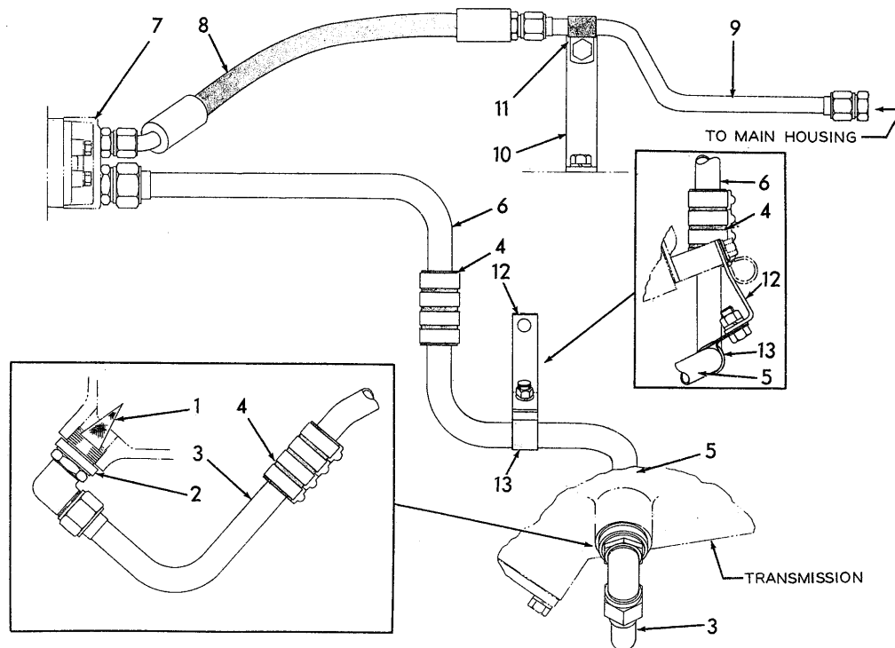
TRANSMISSION SCAVENGING LINES
