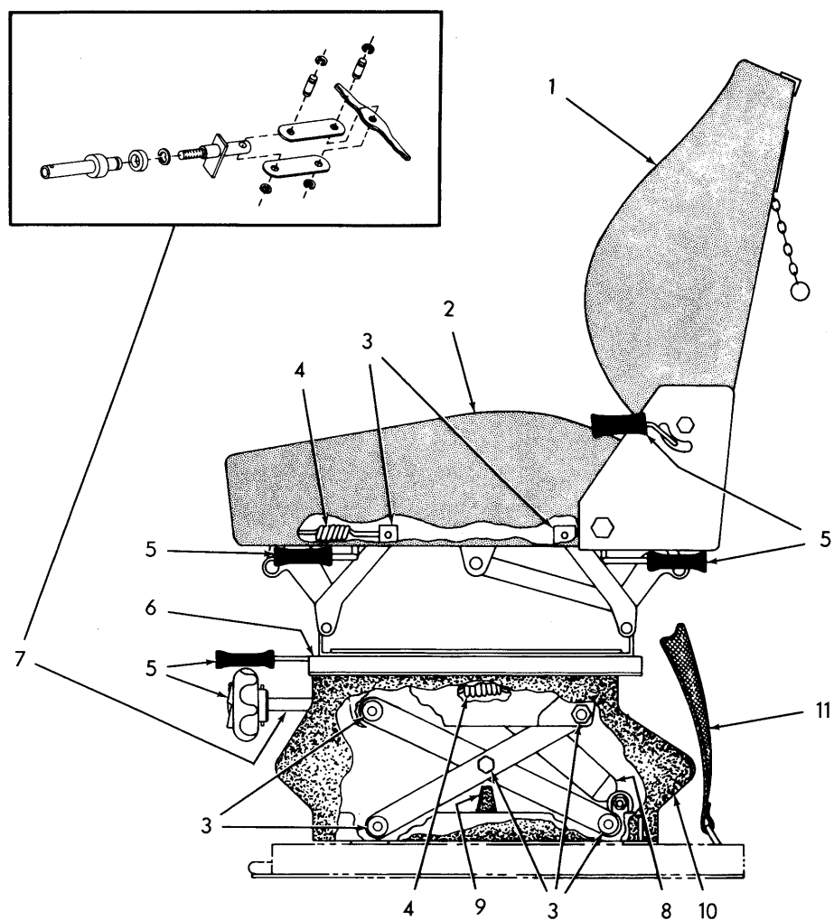
SEAT ASSEMBLY
