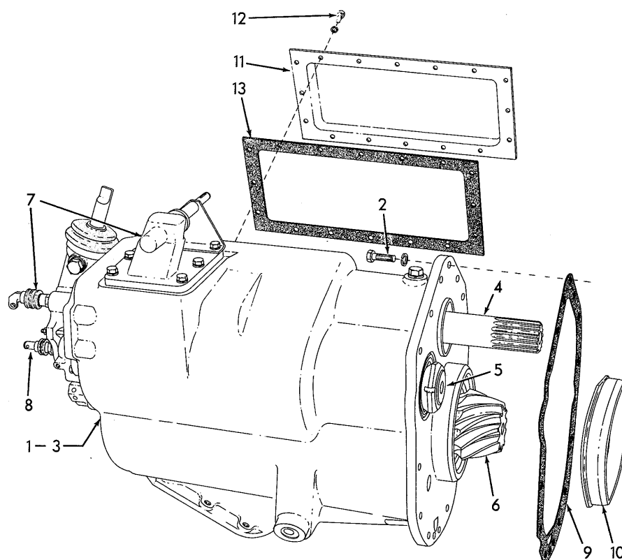
TRANSMISSION
