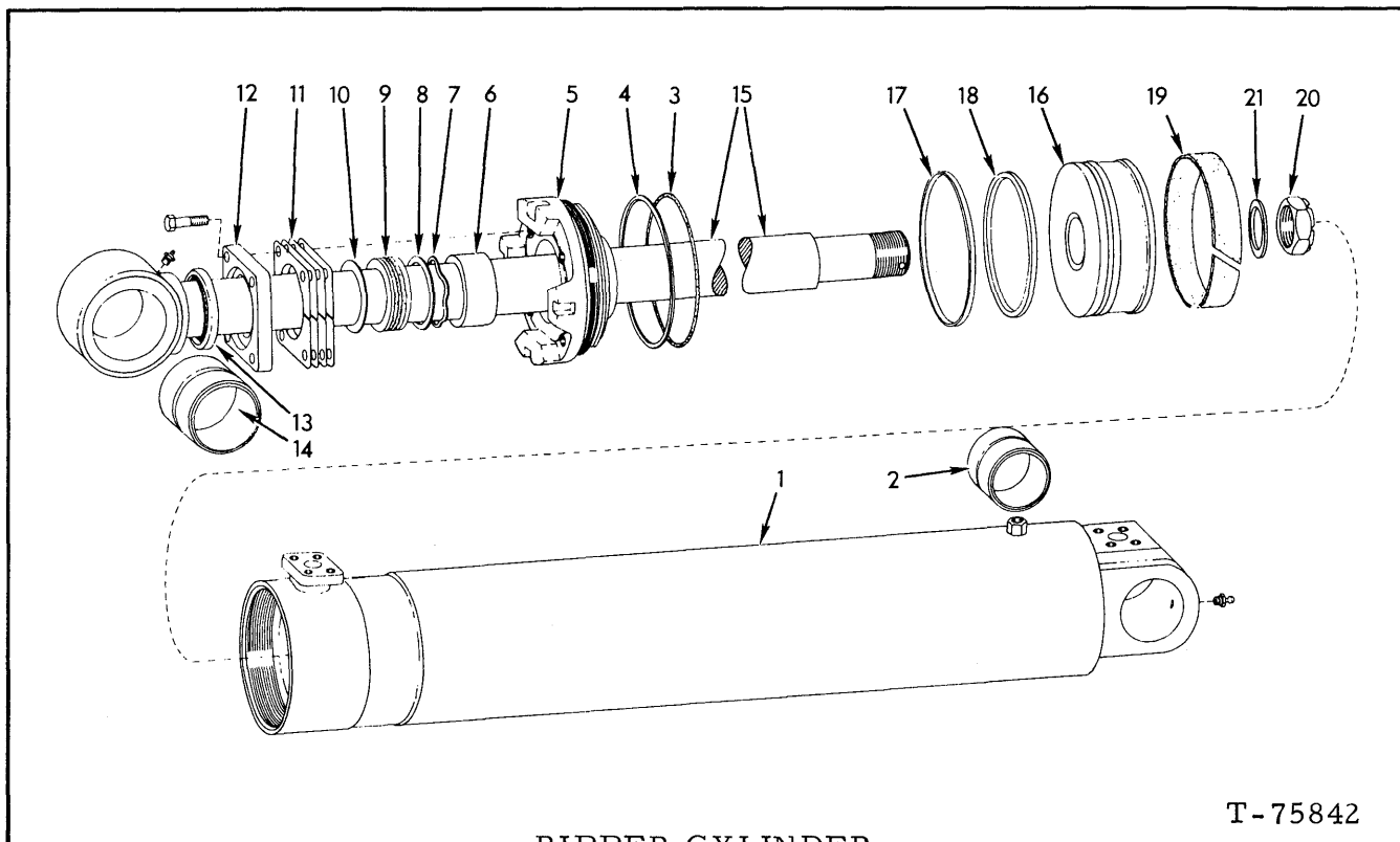
— RIPPER CYLINDER —
