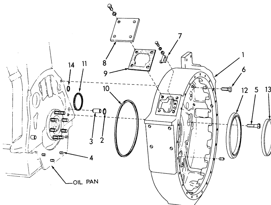
FLYWHEEL HOUSING
