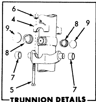
TRUNNION DETAILS
