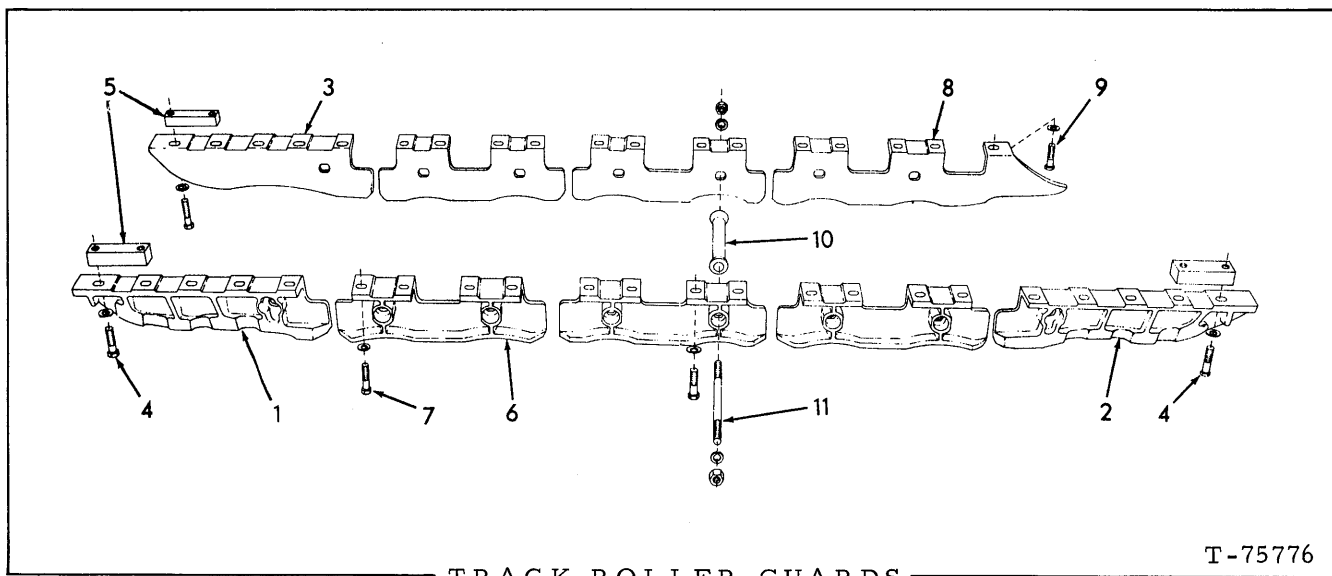
TRACK ROLLER GUARDS
