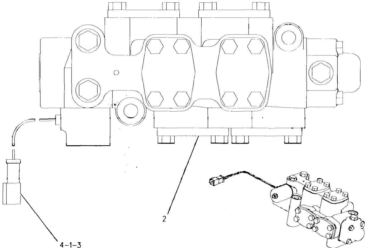
ISO VIEW OF VALVE GP
