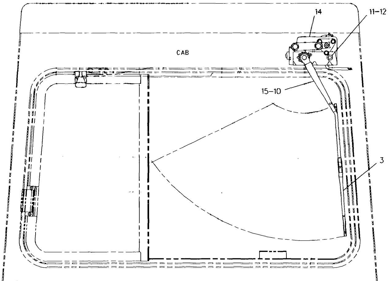
REAR VIEW
