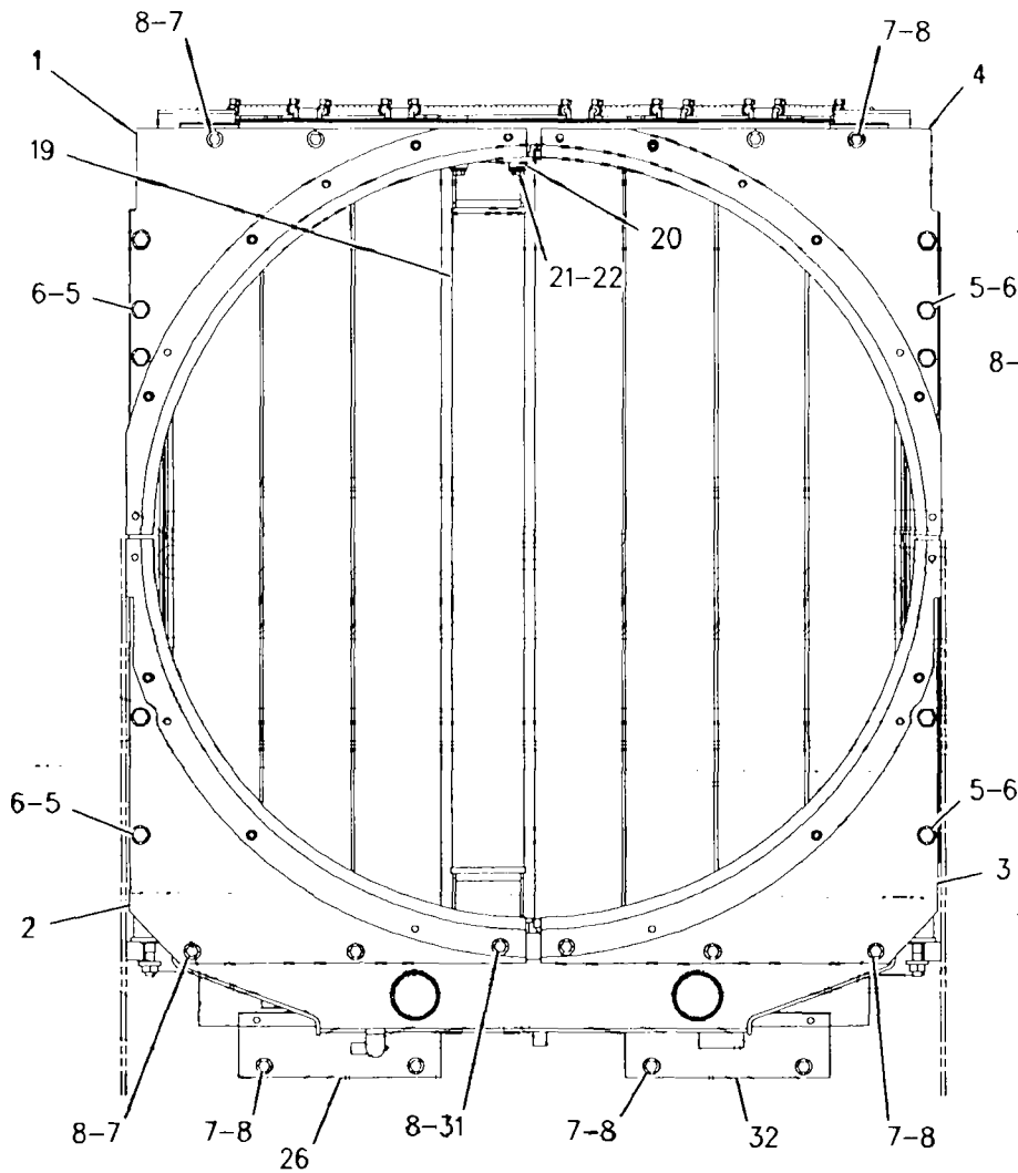
REAR VIEW
