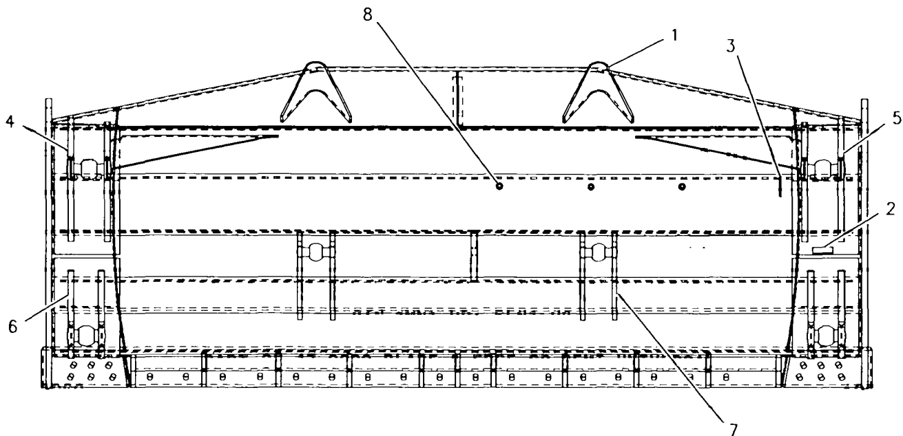
REAR VIEW
