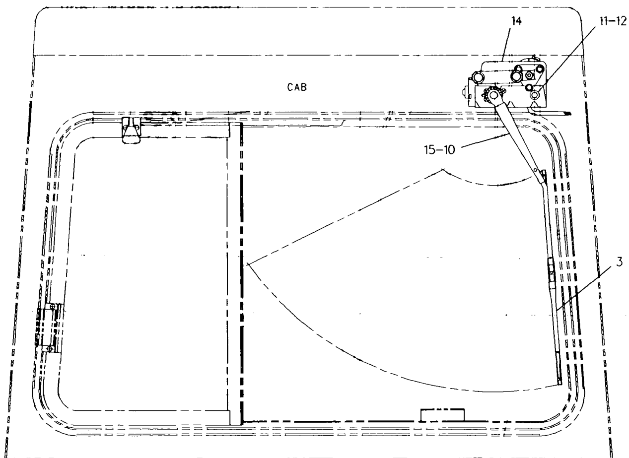
REAR VIEW
