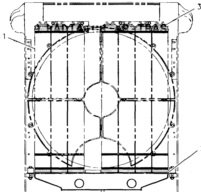
REAR VIEW
