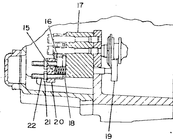
VIEW B-B
