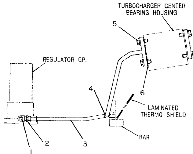
END VIEW
