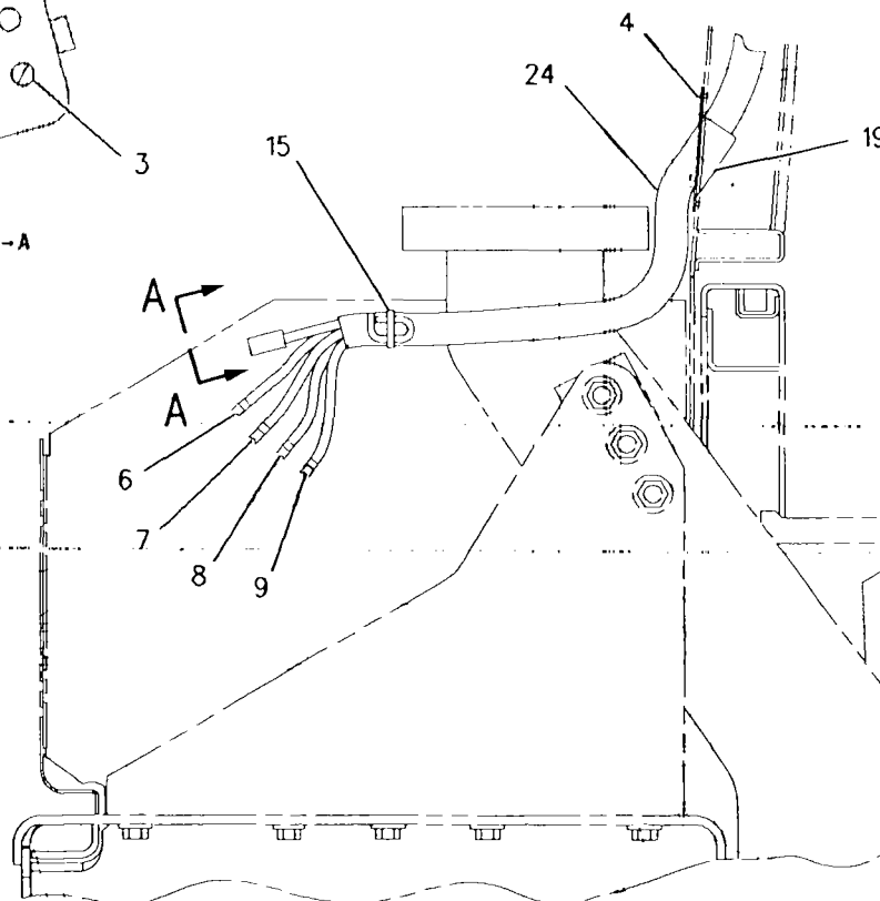
REAR VIEW
