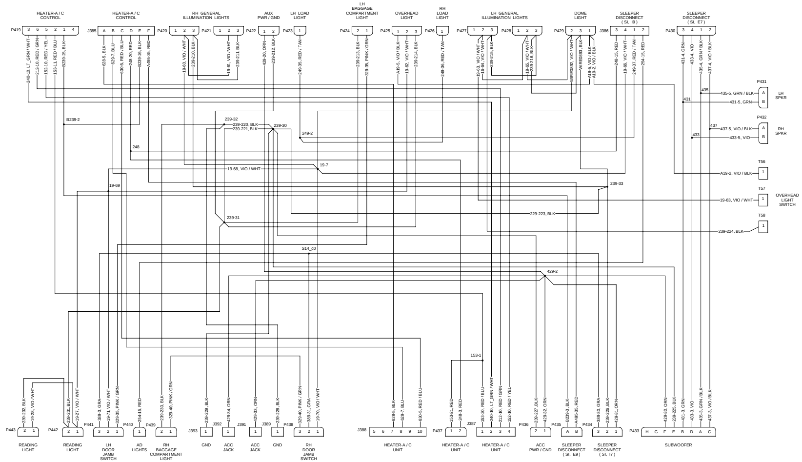
SLEEPER HARNESS - 48" / 63"
