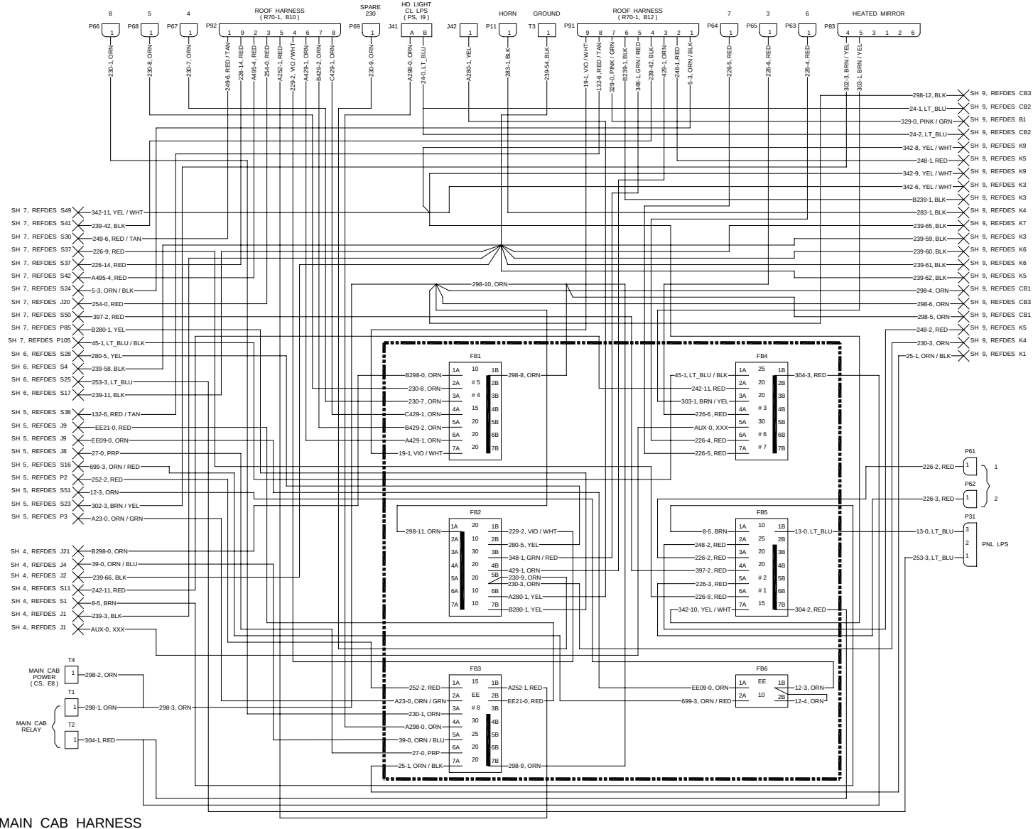
MAIN CAB HARNESS
