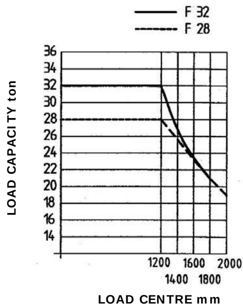
LOAD DIAGRAM – F 28 – F 32
