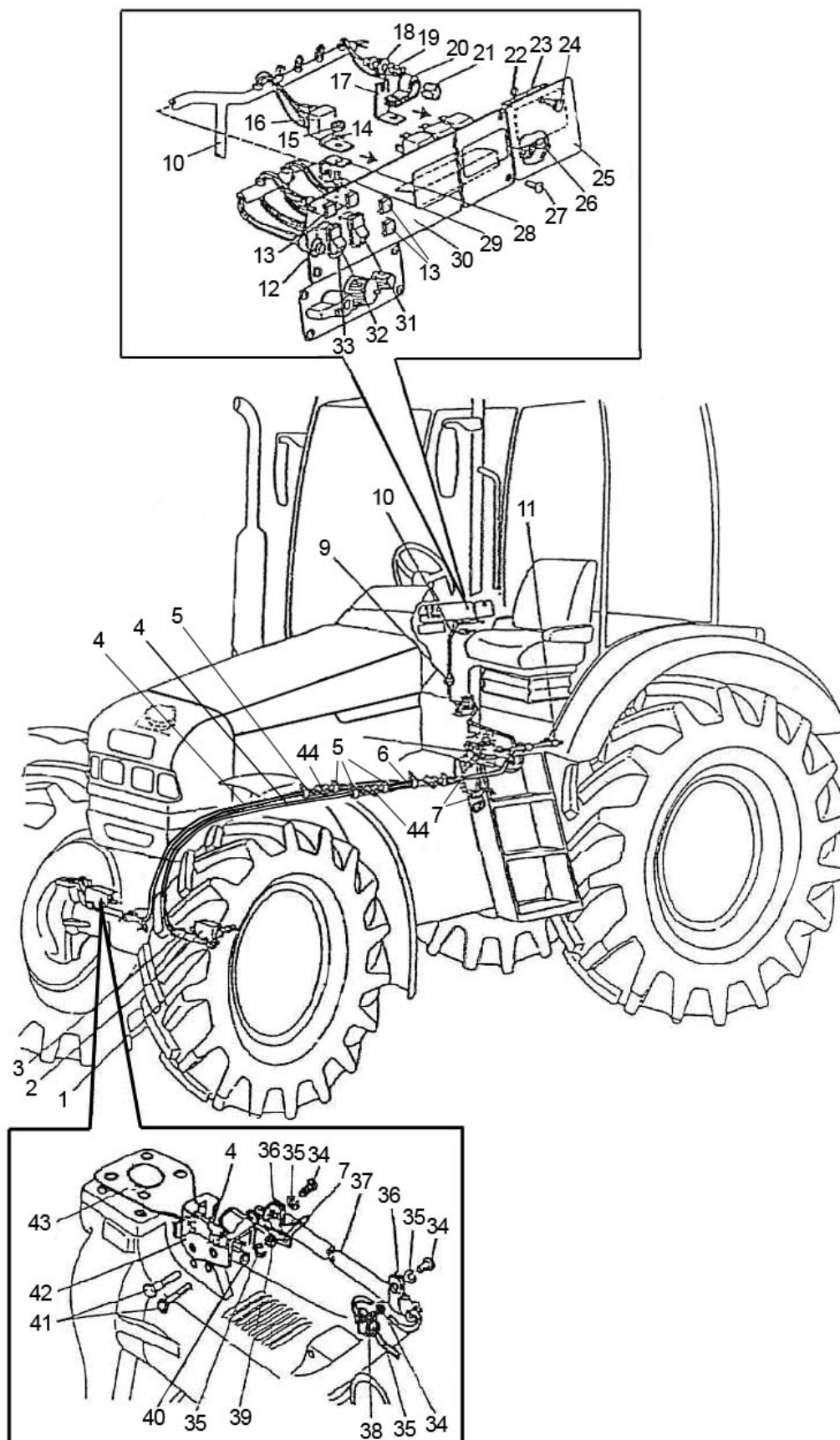
Fig.87.3 Control of DL, FDA and reduction unit (with GB 24x12 and FDA 1525-2300020)
