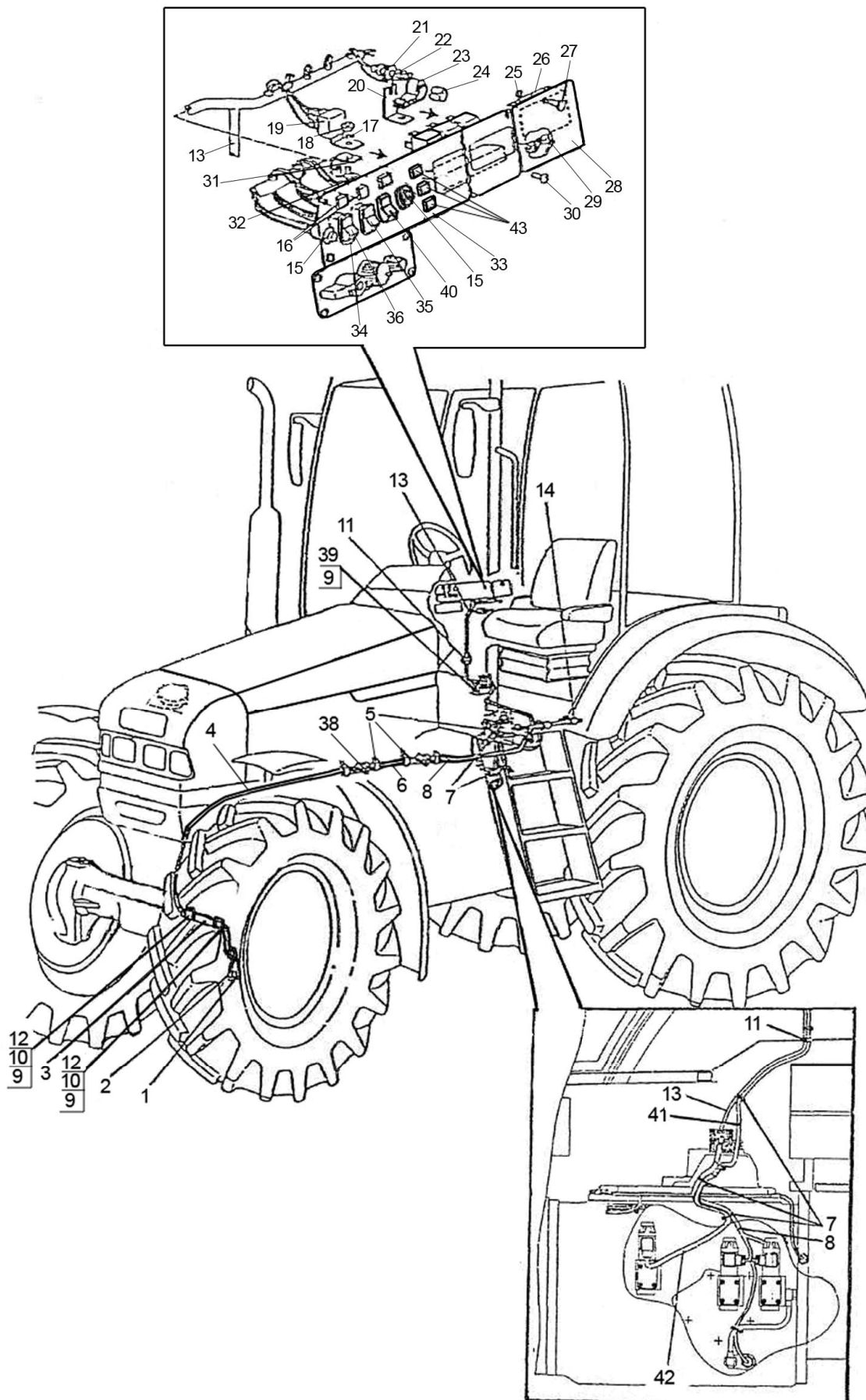
Fig.87.2 Control of DL, FDA and front PTO shaft 1523-8700210-Д
