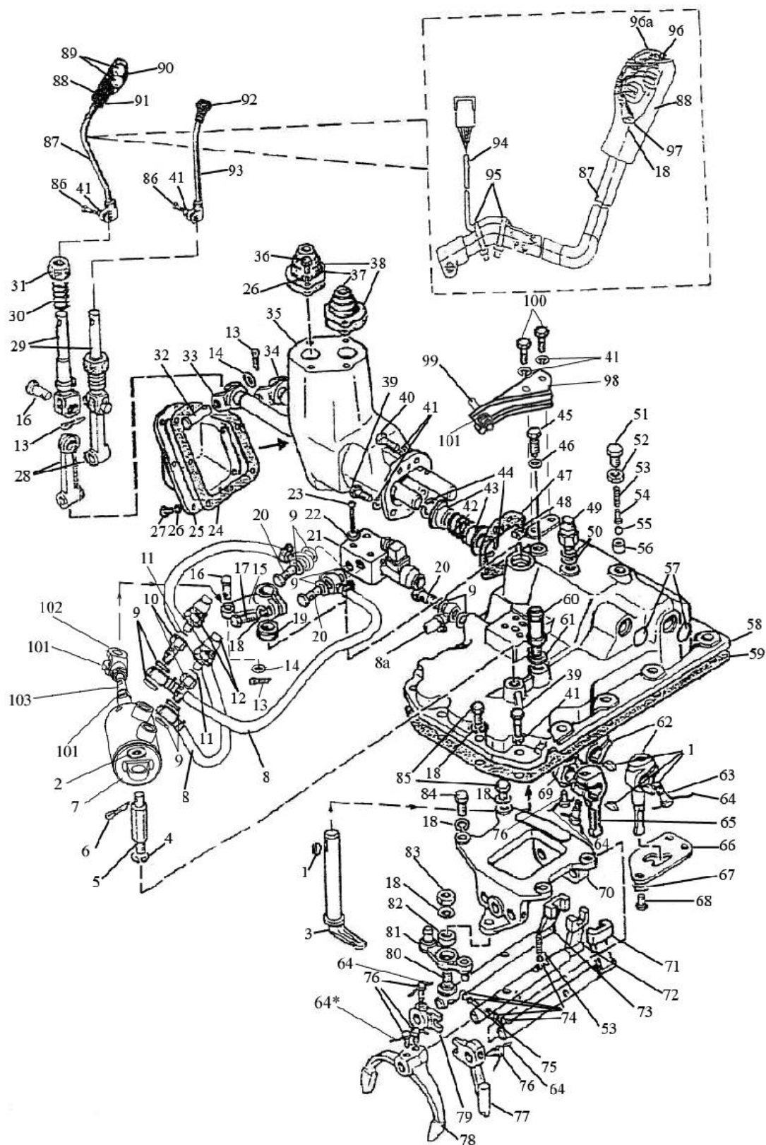
Fig. 17.13 GB control mechanism
