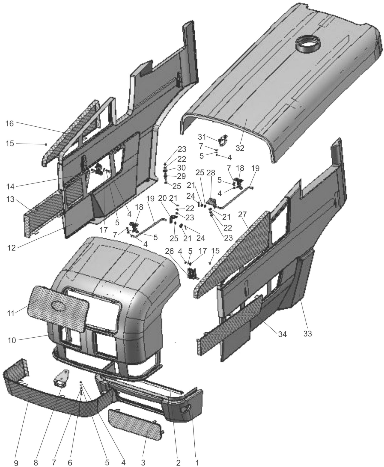
Fig.84.1 Facing
