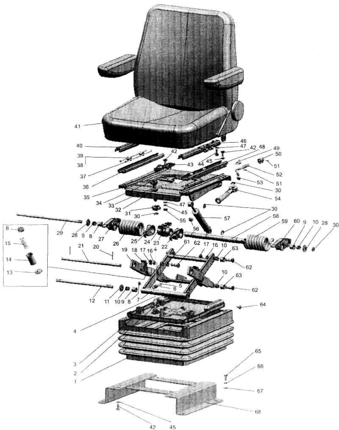
Fig. 68.1 Operator seat
