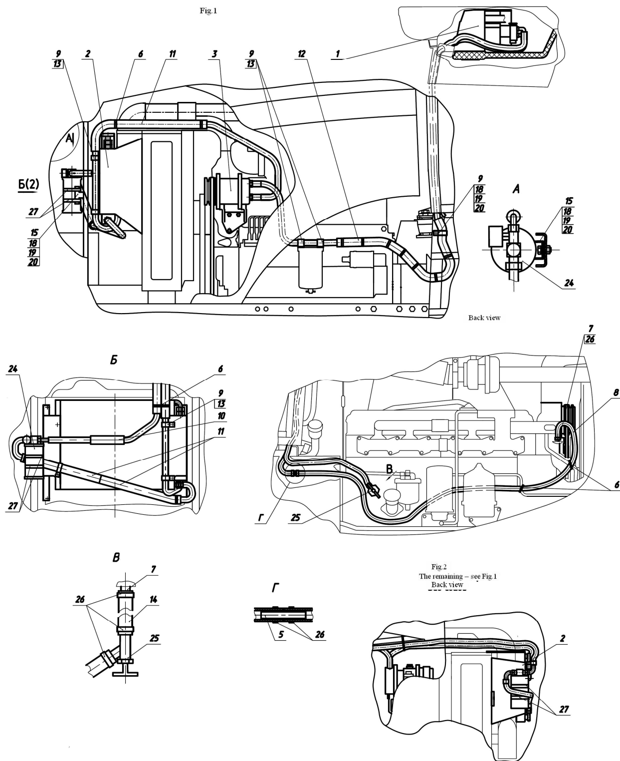
Fig.81.1 Air conditioner installation
