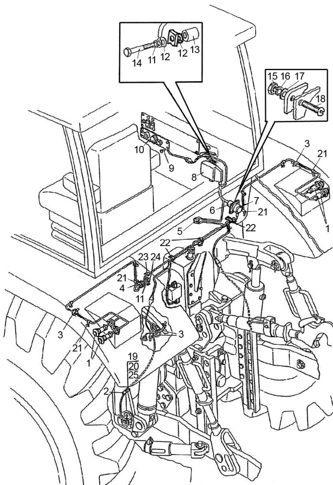
Fig.87.4 Control of lift linkage 1522-8700610
