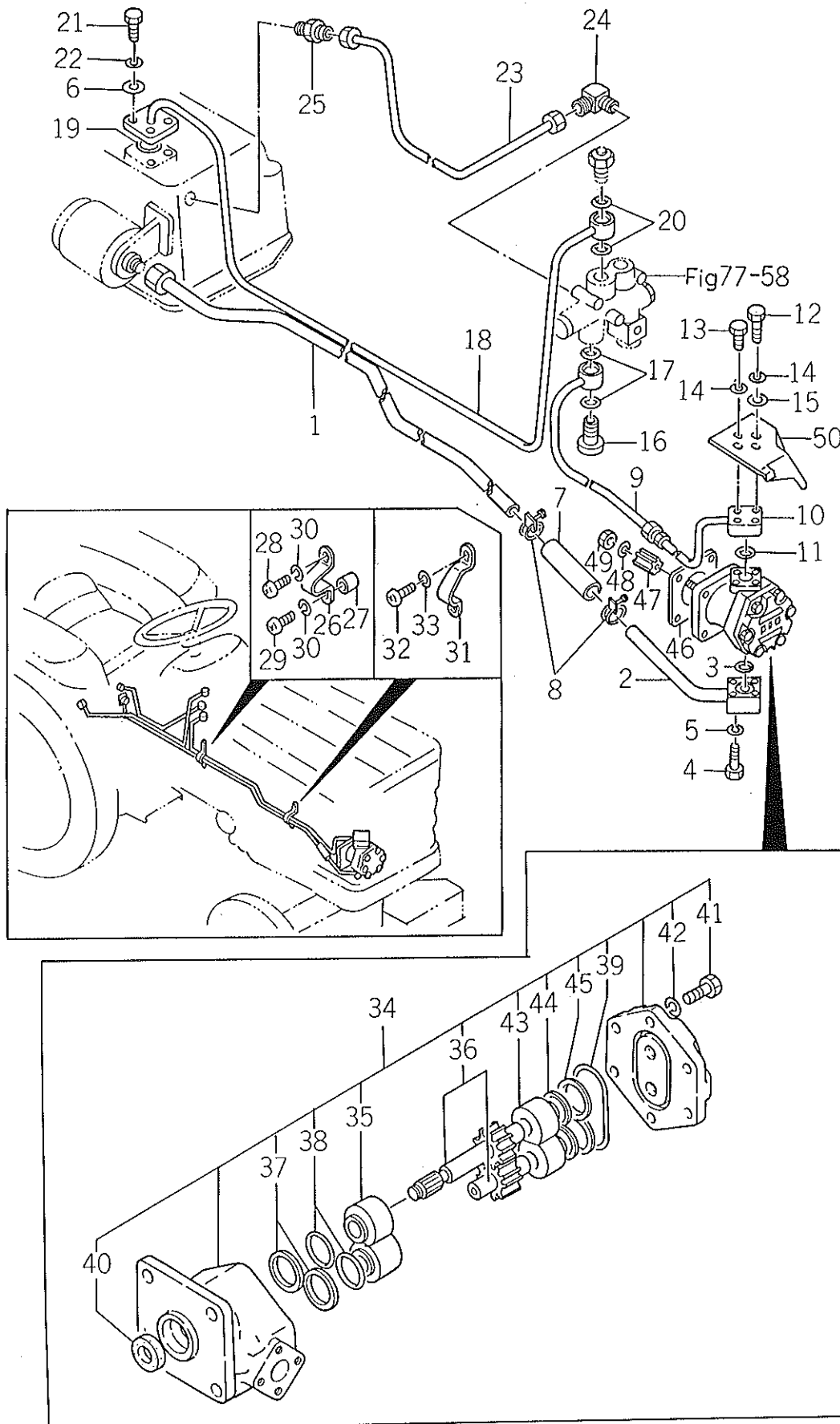
Fig. 65 HYDRAULIC PIPING (FOR DUG, F-UG, F-DUG, LF-DUG TYPE)
