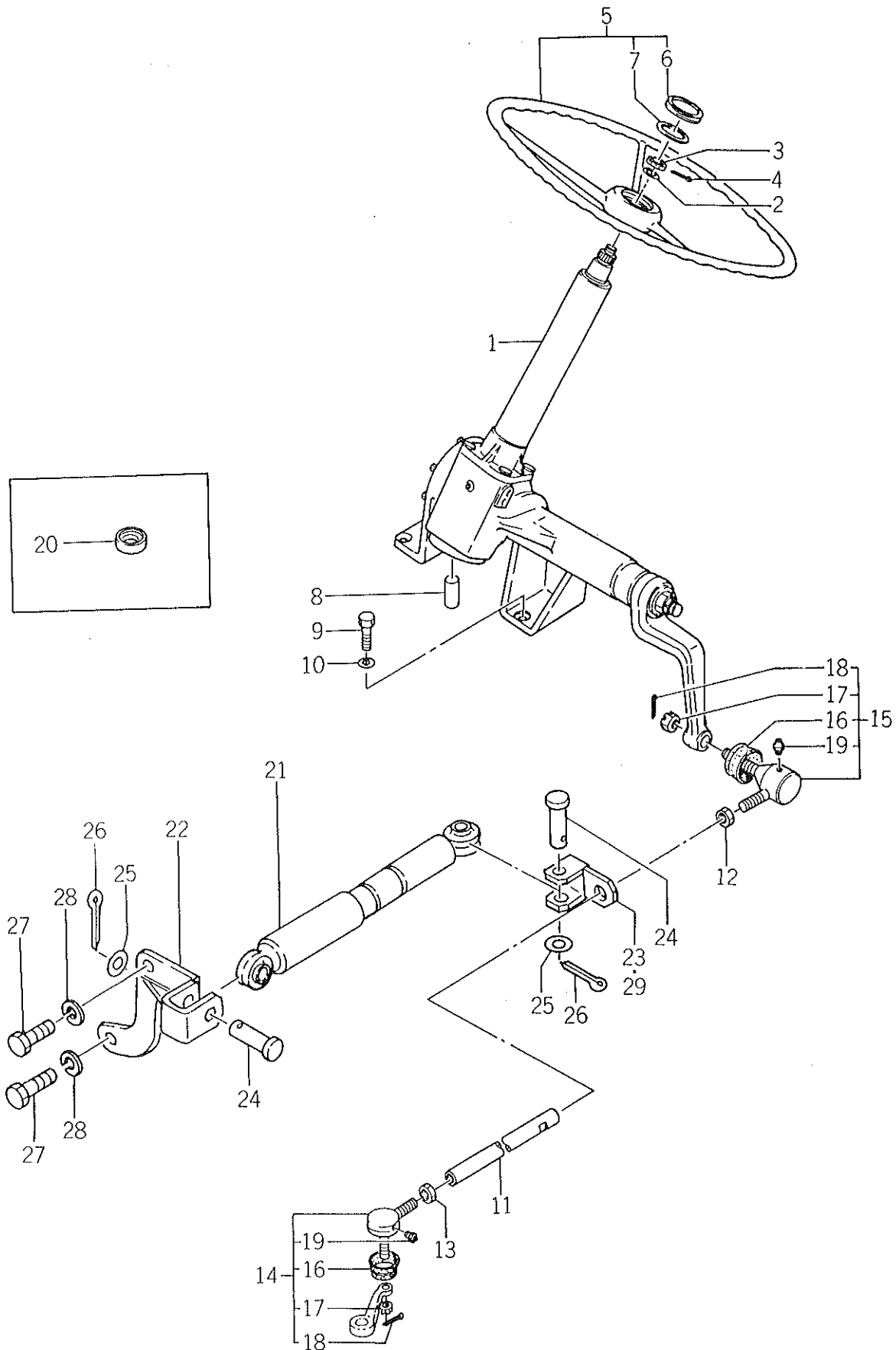
Fig. 35 STEERING WHEEL (MECHANICAL TYPE) (FOR S, D, SG, DG TYPE)
