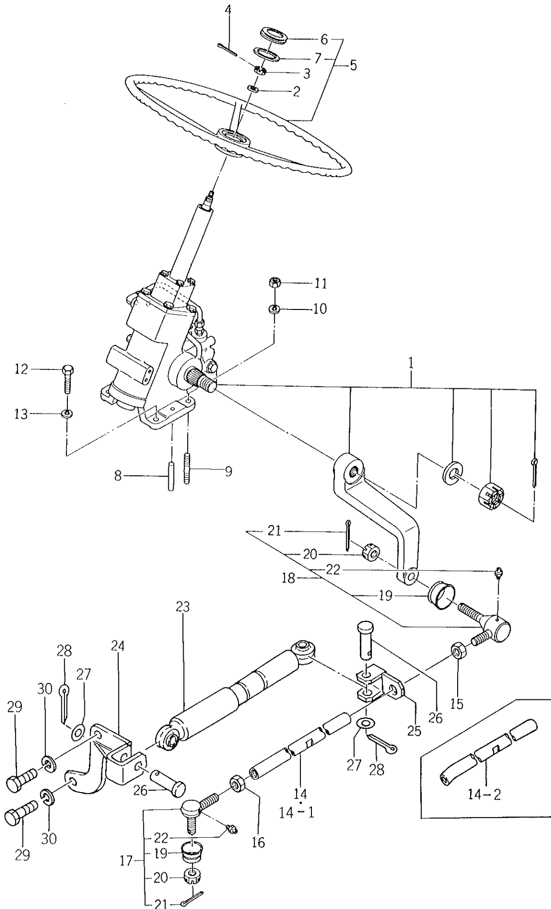
Fig. 36 STEERING WHEEL (POWER TYPE) (FOR DU, DUG, 4WD TYPE)
