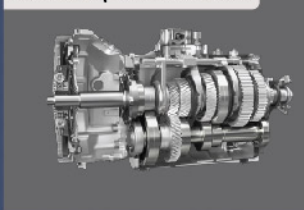
ET90 6 Speed Gearbox
