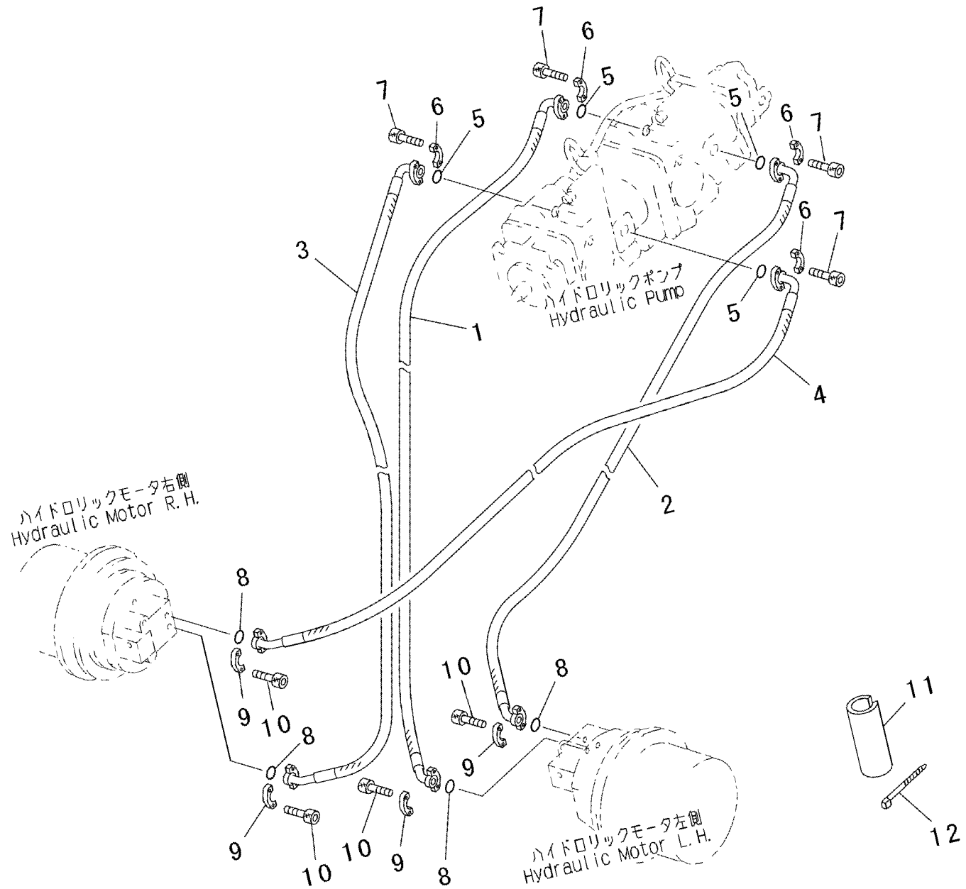
FIG. 503 HYDRAULIC OIL PIPING (HST MAIN LINE)
