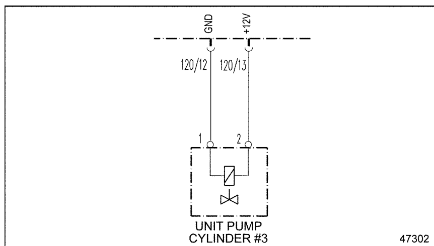
Figure 47-2 Electronic Unit Pump #3
