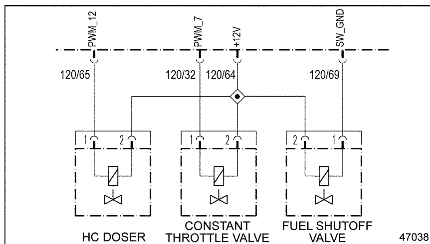
Figure 30-2 Constant Throttle Valve
