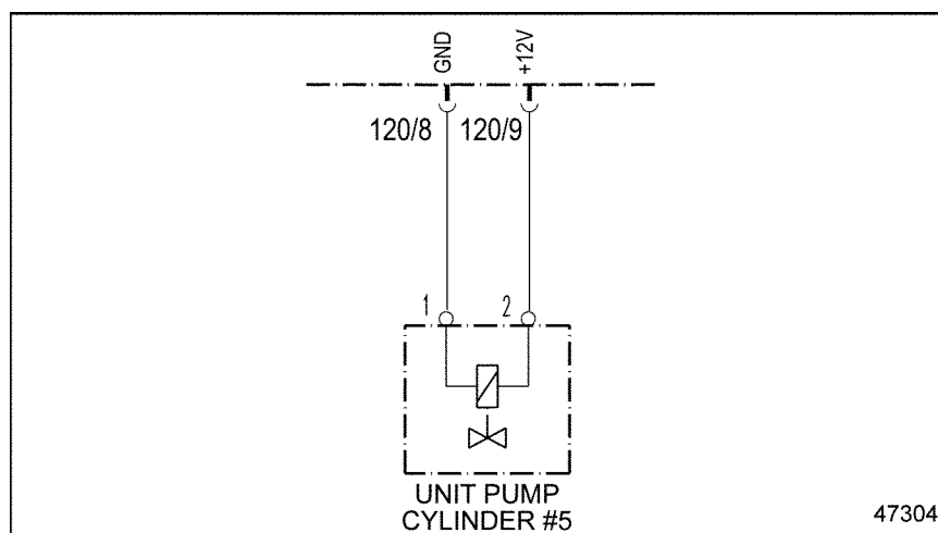
Figure 49-2 Electronic Unit Pump #5
