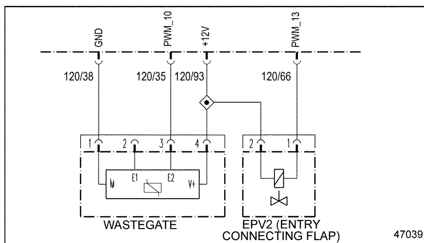
Figure 31-1 Wastegate
