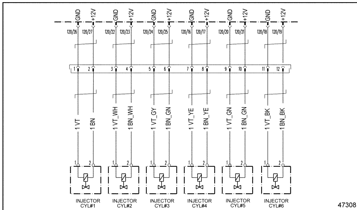
Figure 25-2 MBE 900 Injectors
