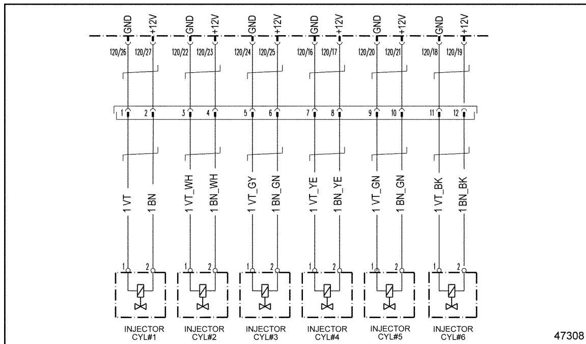
Figure 24-2 MBE 900 Injectors
