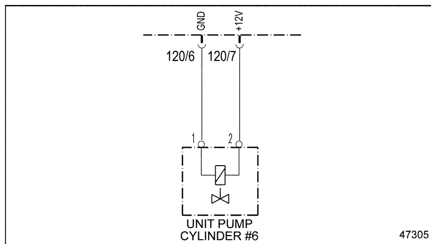
Figure 50-1 Electronic Unit Pump #6
