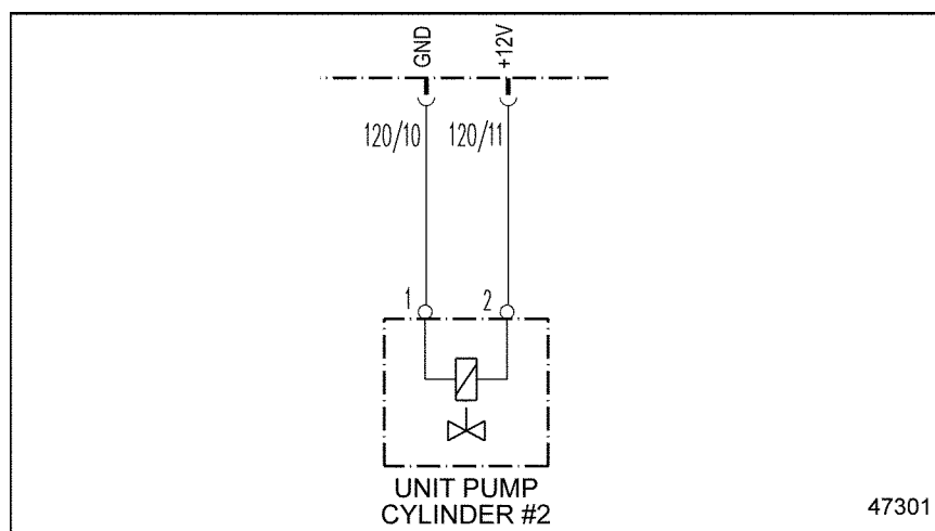
Figure 46-2 Electronic Unit Pump #2
