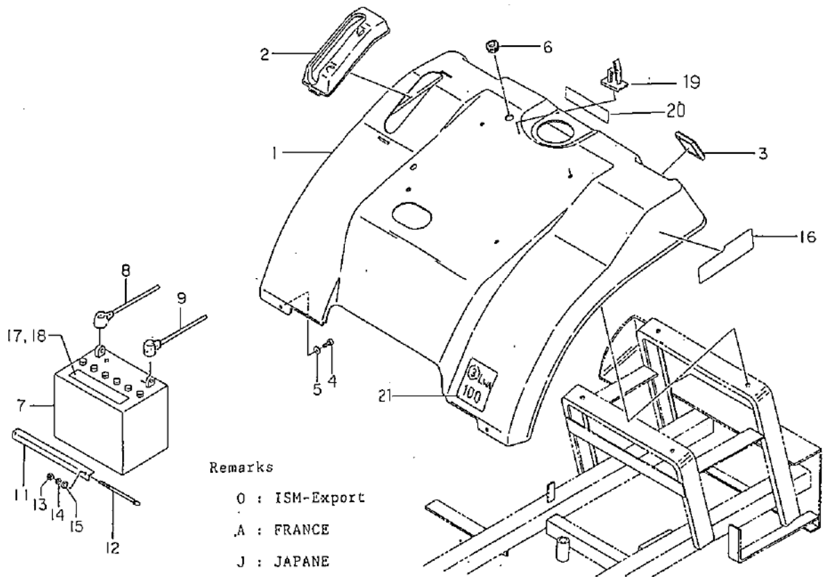
FIG.209 FENDER, BATTERY ; LT 14,16
