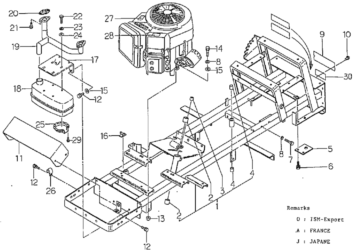
FIG.202 CHASSIS MUFFLER ; LT 16
