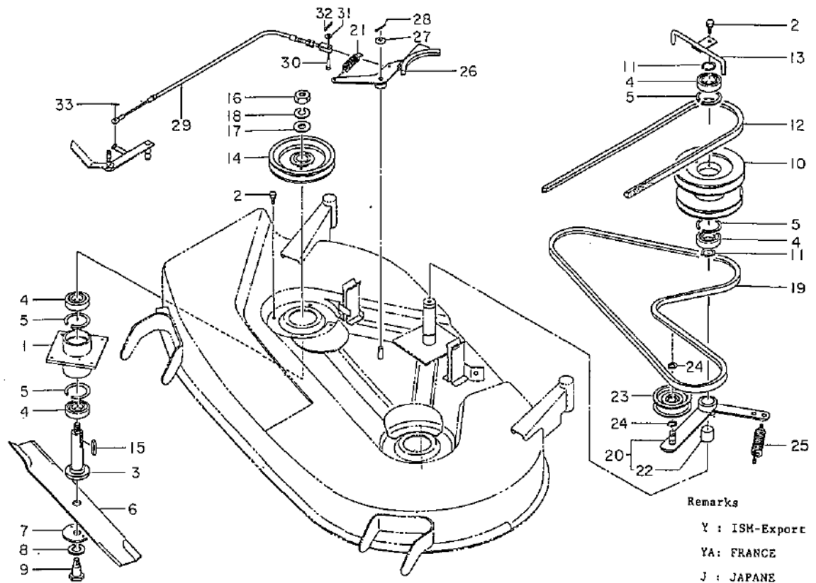
FIG.302 PULLEY, TENSION ; MM 40
