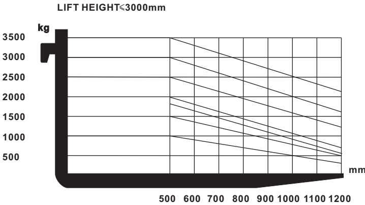
Load chart
