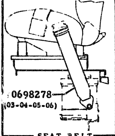
SEAT BELT
