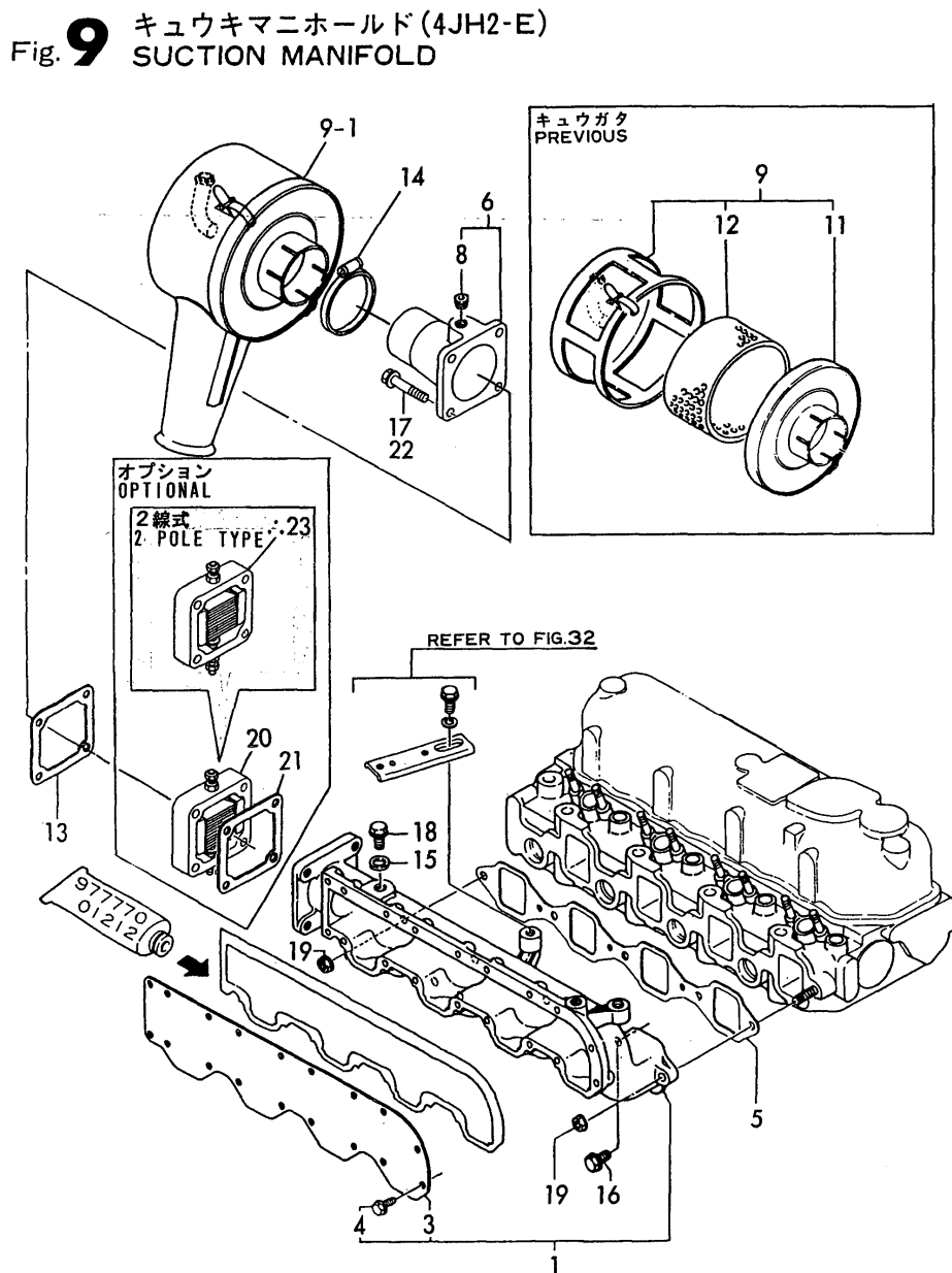
Fig.9.SUCTION MANIFOLD(4JH2E)
