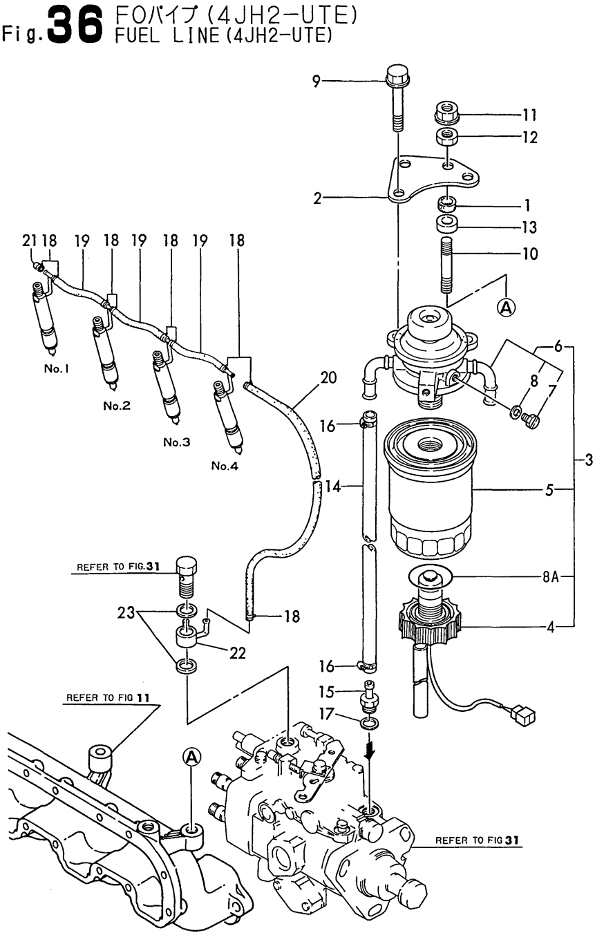
Fig.36.FUEL PIPE(4JH2-UTE)
