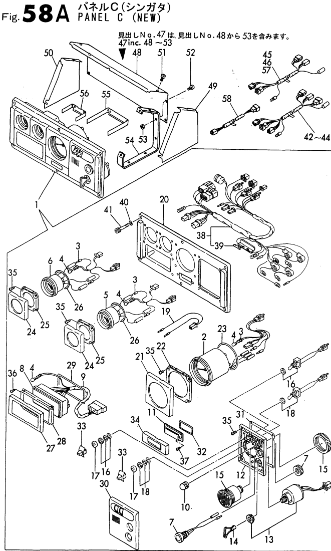
Fig.94.(58A)INSTRUMENT PANEL(C-TYPE,NEW)
