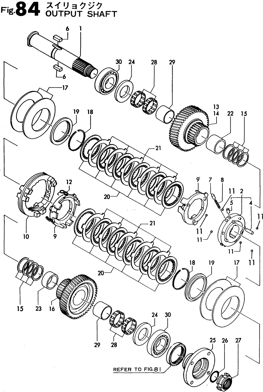
Fig.84.OUTPUT SHAFT
