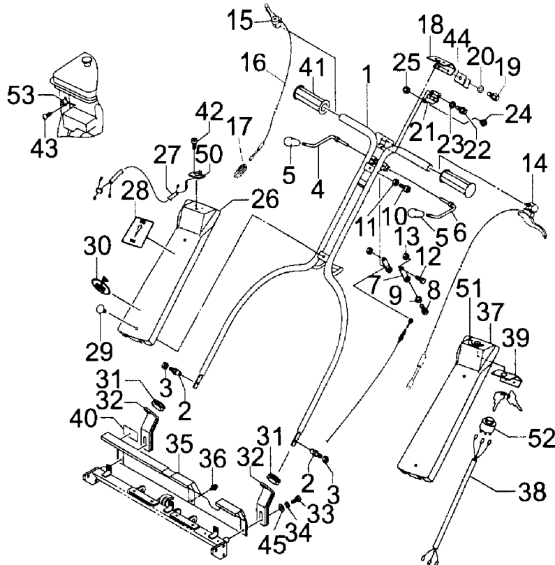
FIG.12 HANDLE
