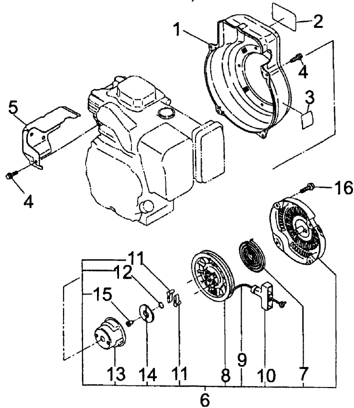
FIG.5 COOLING, STARTING
