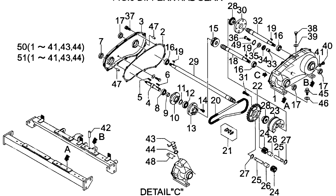
FIG.3 DIFFERENTIAL GEAR
