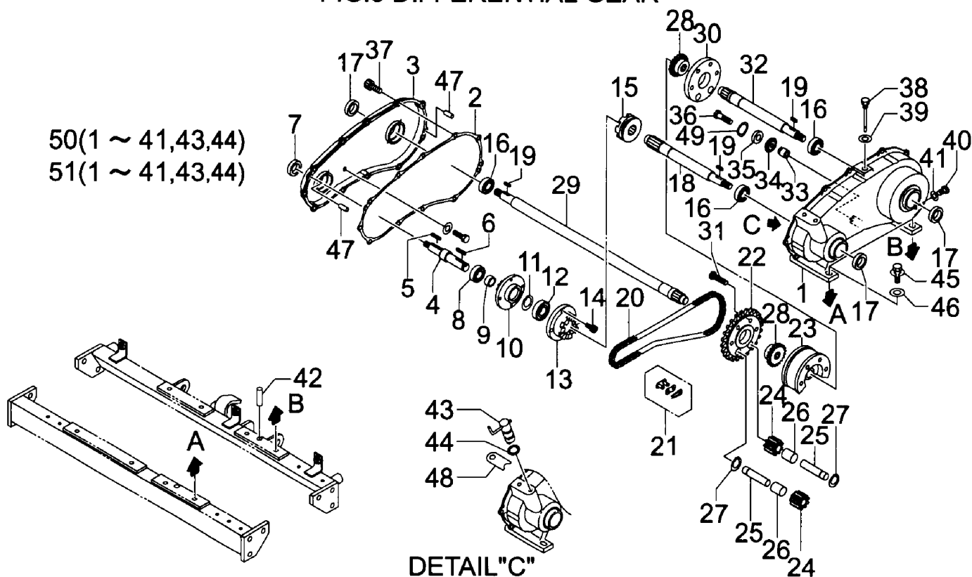
FIG.3 DIFFERENTIAL GEAR
