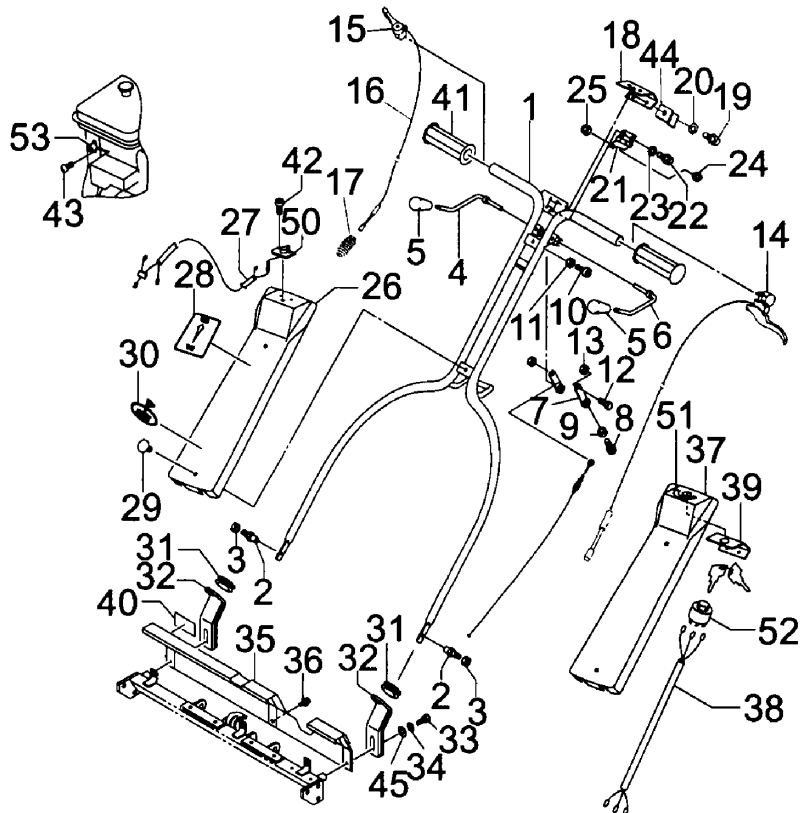
FIG.12 HANDLE
