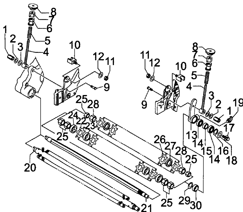
FIG.9 GROOMING CUTTER
