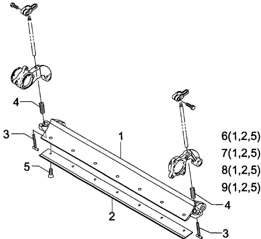
FIG.8-1 BED KNIFE SHOE
