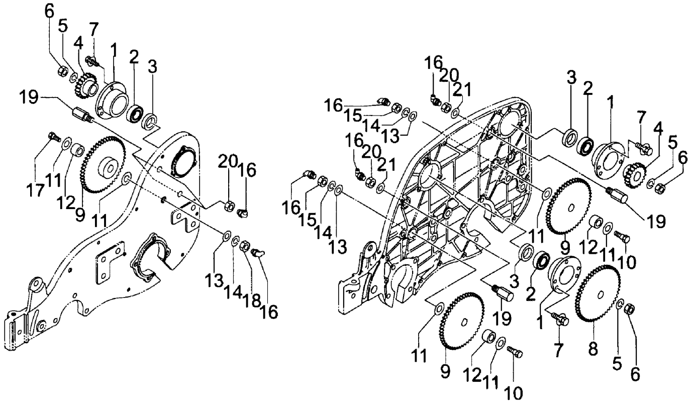
FIG.6 GEAR DRIVE
