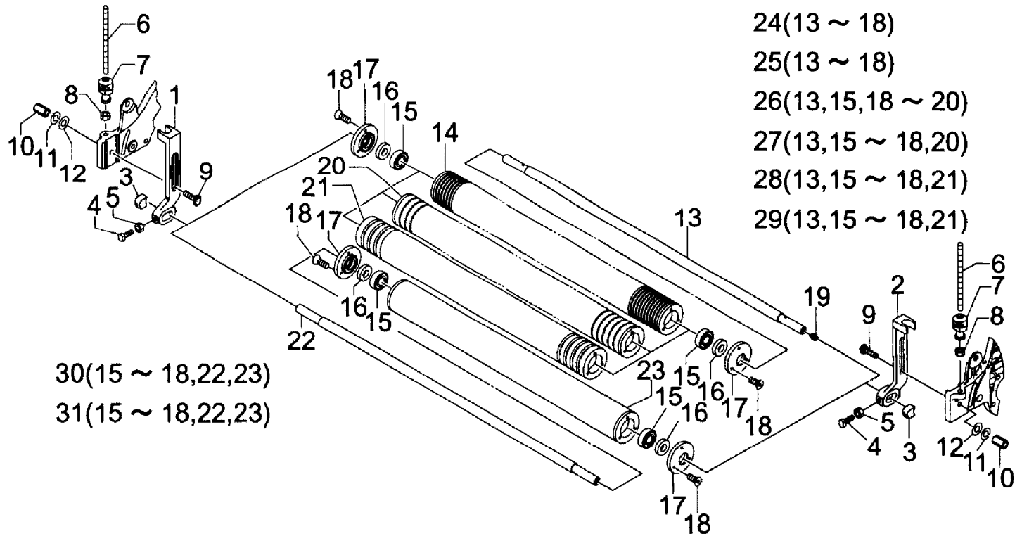
FIG.10 FRONT ROLLER
