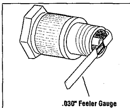
Figure 5-4: Spark plug.
