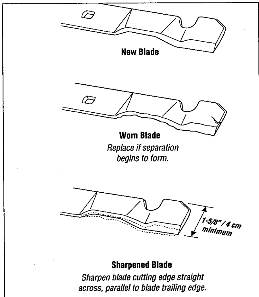
Figure 5-16: Blade Inspection.
