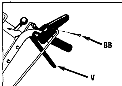
Figure 2-4: Attach wheel drive control rod to lever.
