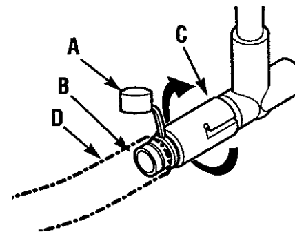
Figure 5-2: Oil drain.
