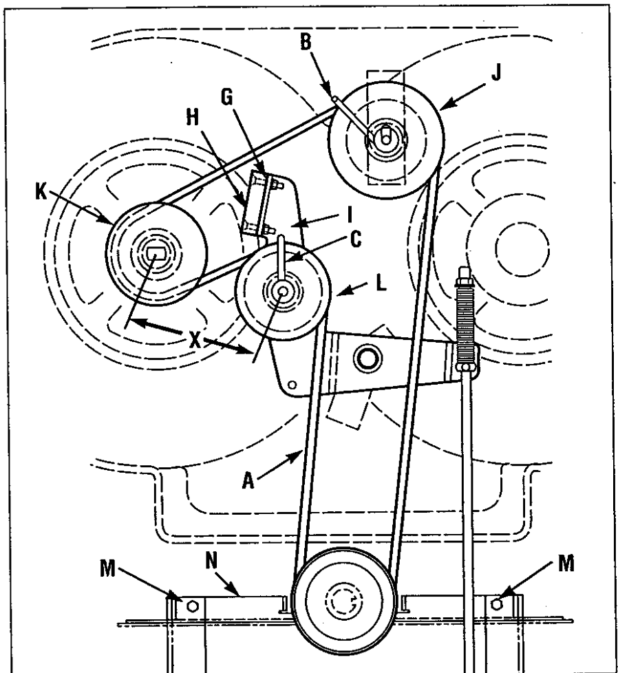
Figure 5-8: Blade drive.
