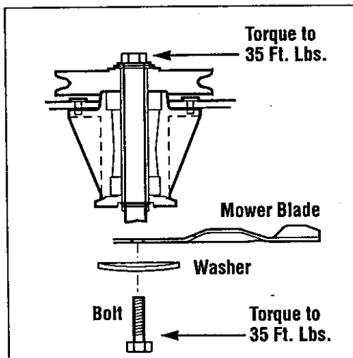
Figure 5-18: Blade spindle.
