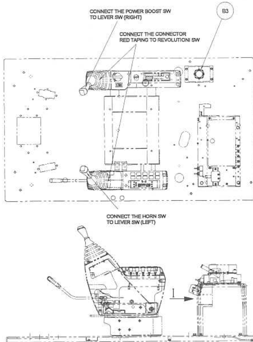
DETAIL OF FLOOR PLATE
