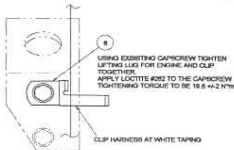
VIEW I (DETAIL OF LIFTING LUG FOR ENGINE)
