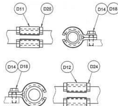
DETAIL OF CLAMP
