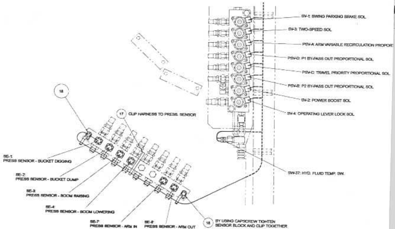
DETAIL OF 1. (PSV BLOCK & PRESSURE SENSOR)
