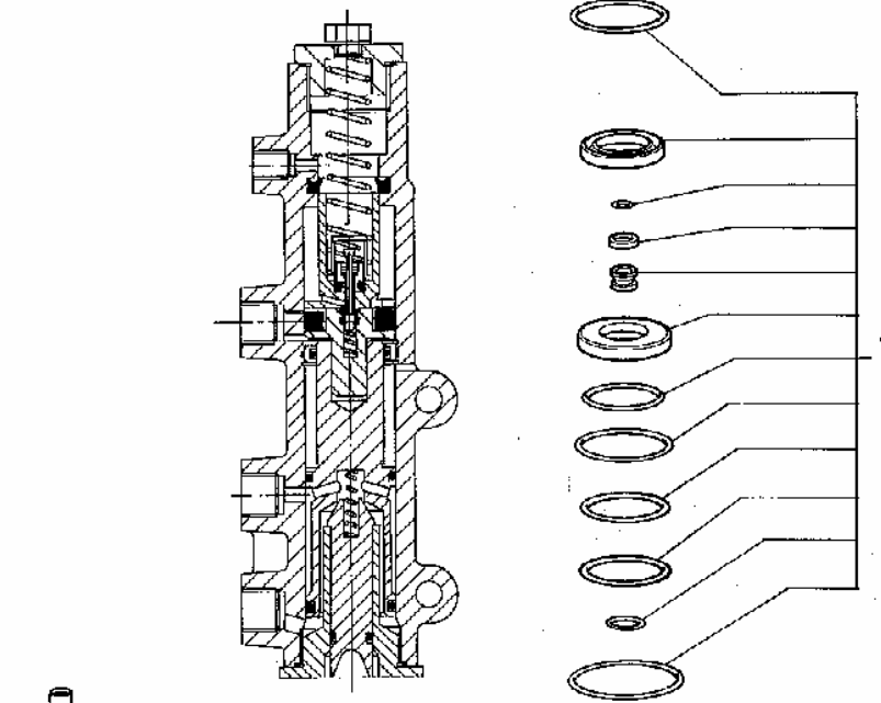
1 BRAKE PUMP POMPA FRENO
