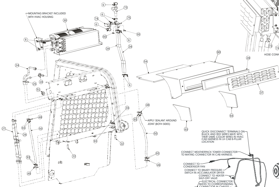
MTG PLATE EXPLODED VIEW
