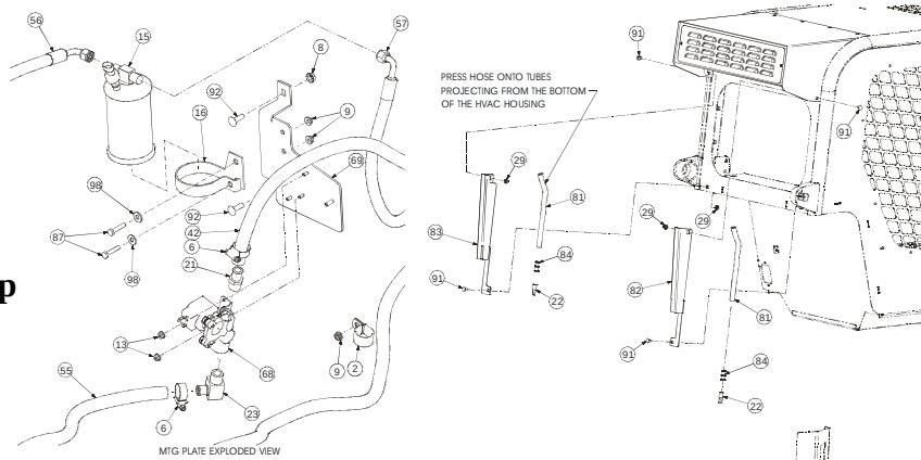
MTG PLATE EXPLODED VIEW
