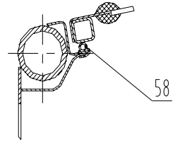
E-E Aligned view
