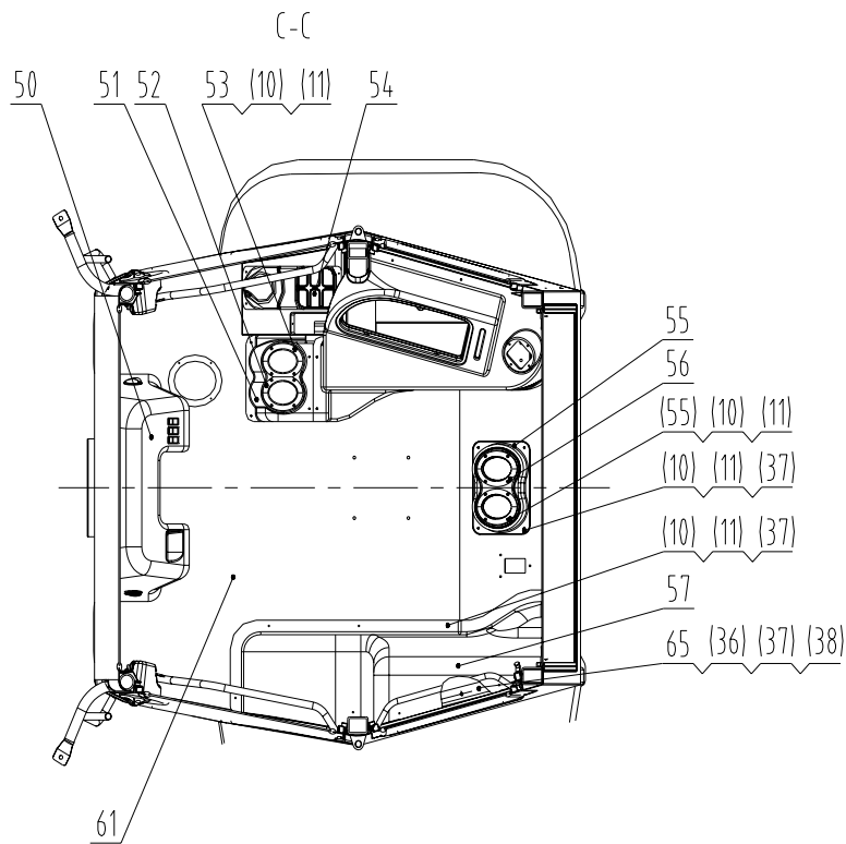
D-D Aligned view
