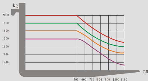
Load Chart (kg) LIFT HEIGHT ≤ 3000mm
