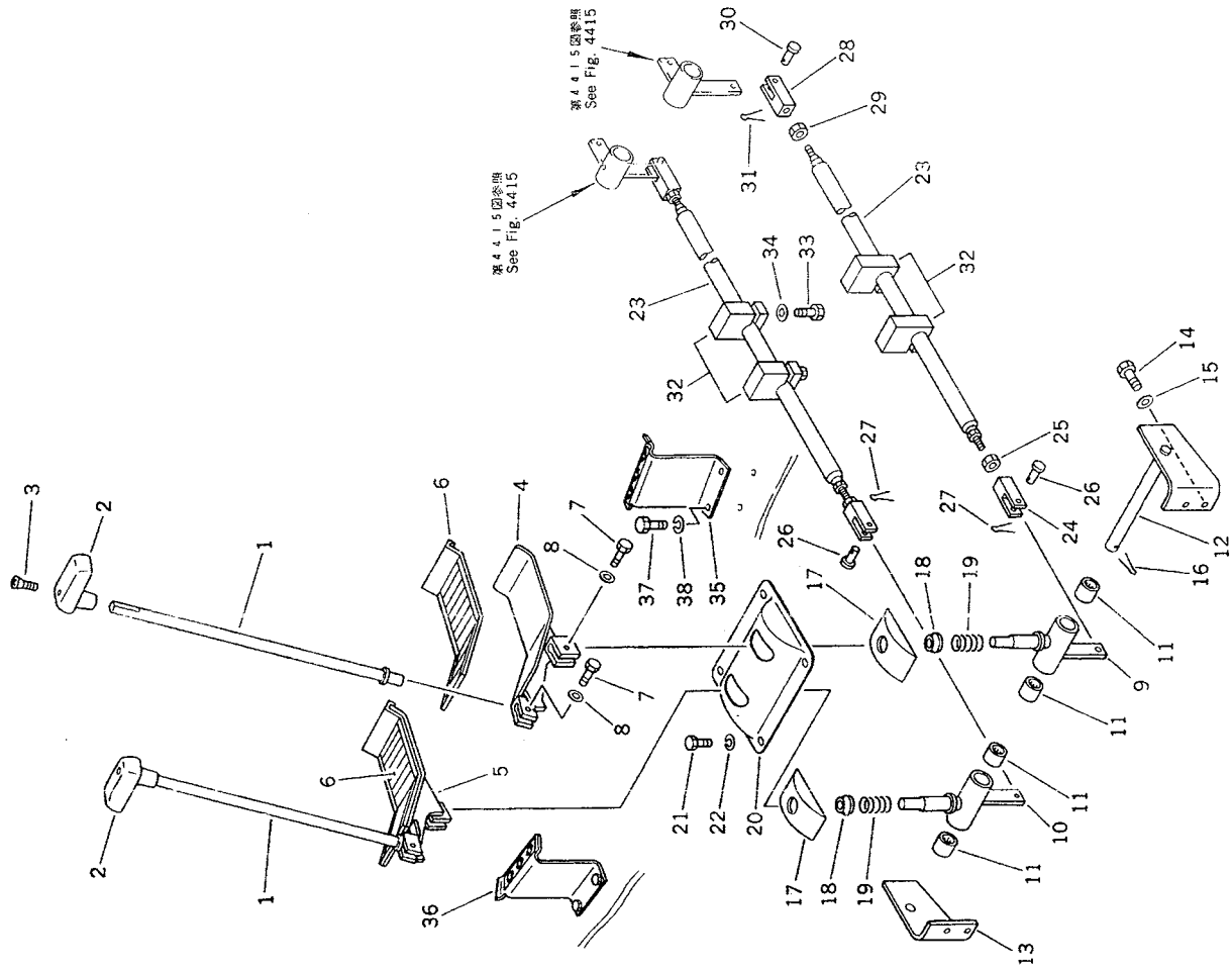
FIG. 8011 TRAVEL CONTROL LEVER AND PEDAL (TBG SPEC.)
