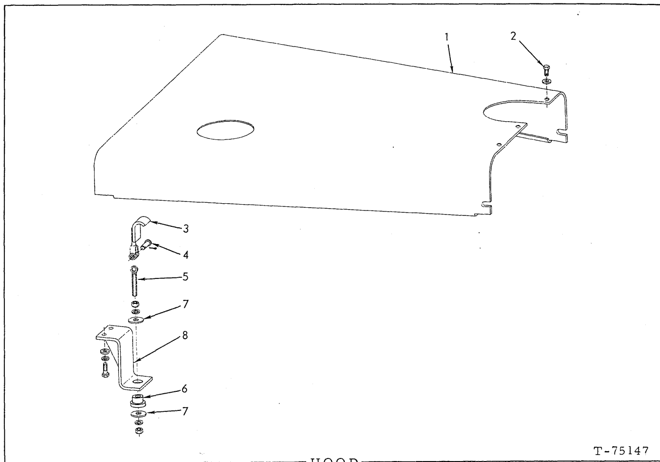
HOOD
