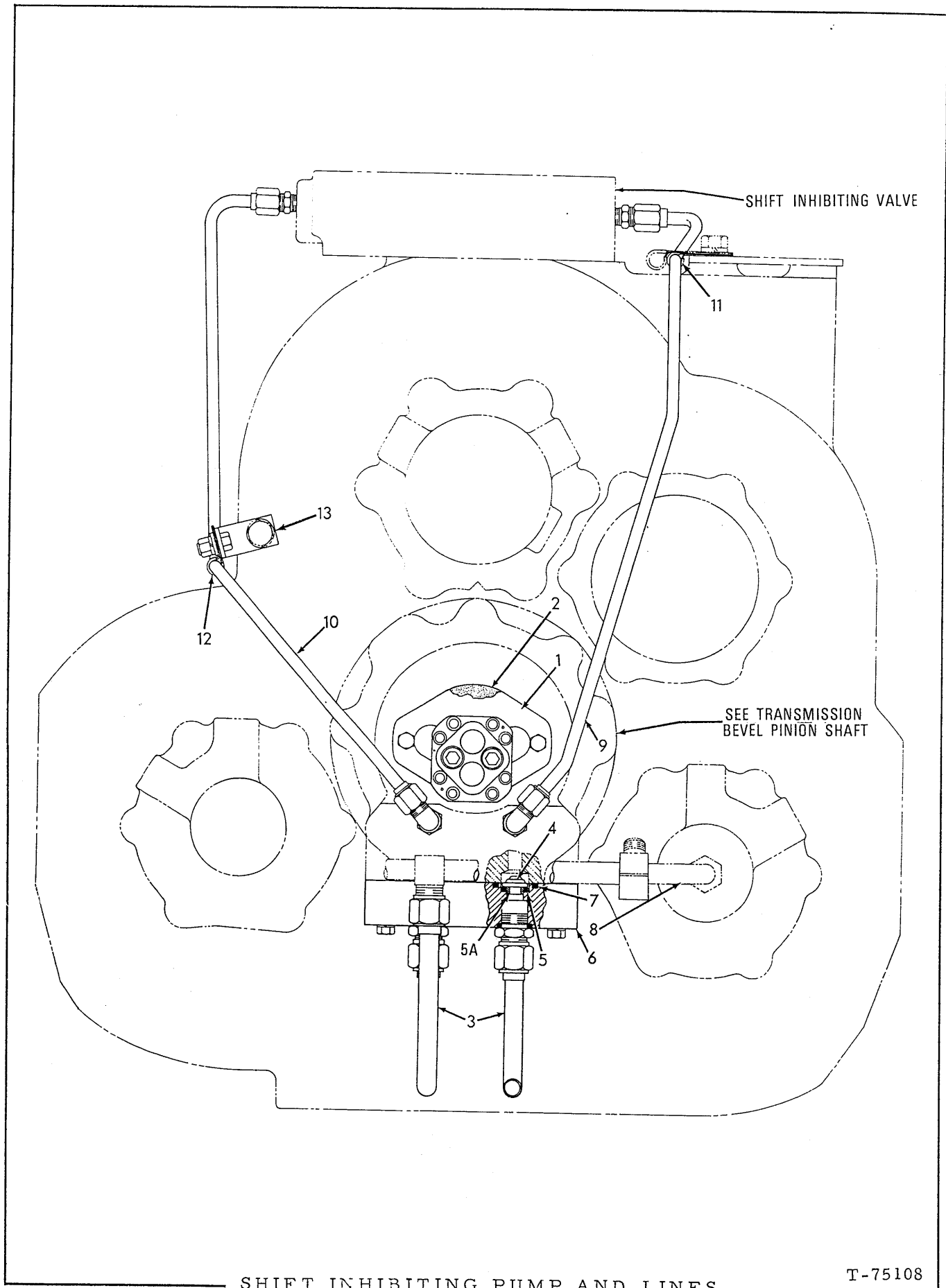
SHIFT INHIBITING PUMP AND LINES
