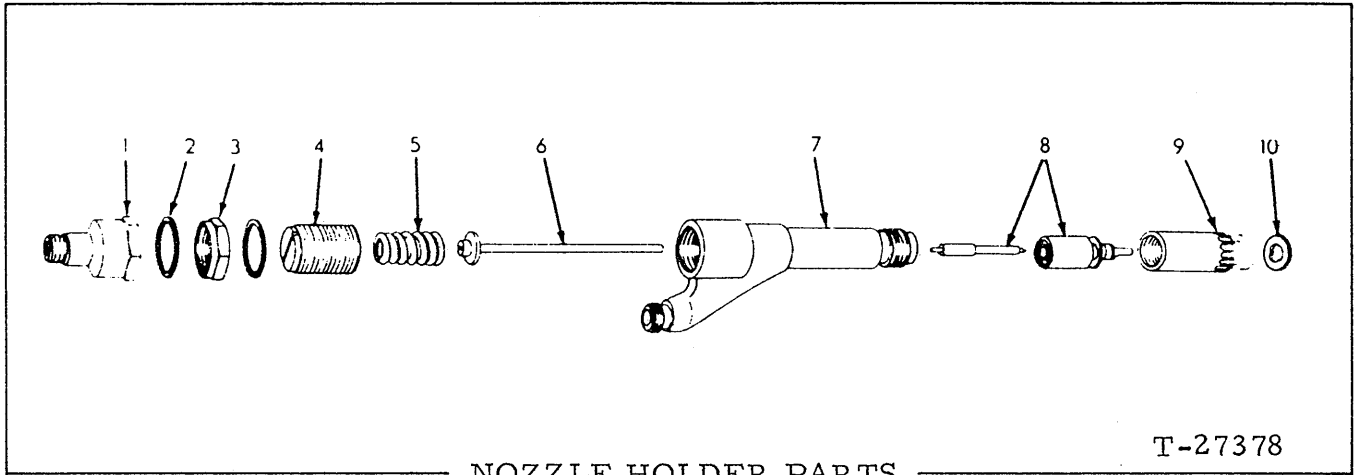
NOZZLE HOLDER PARTS
