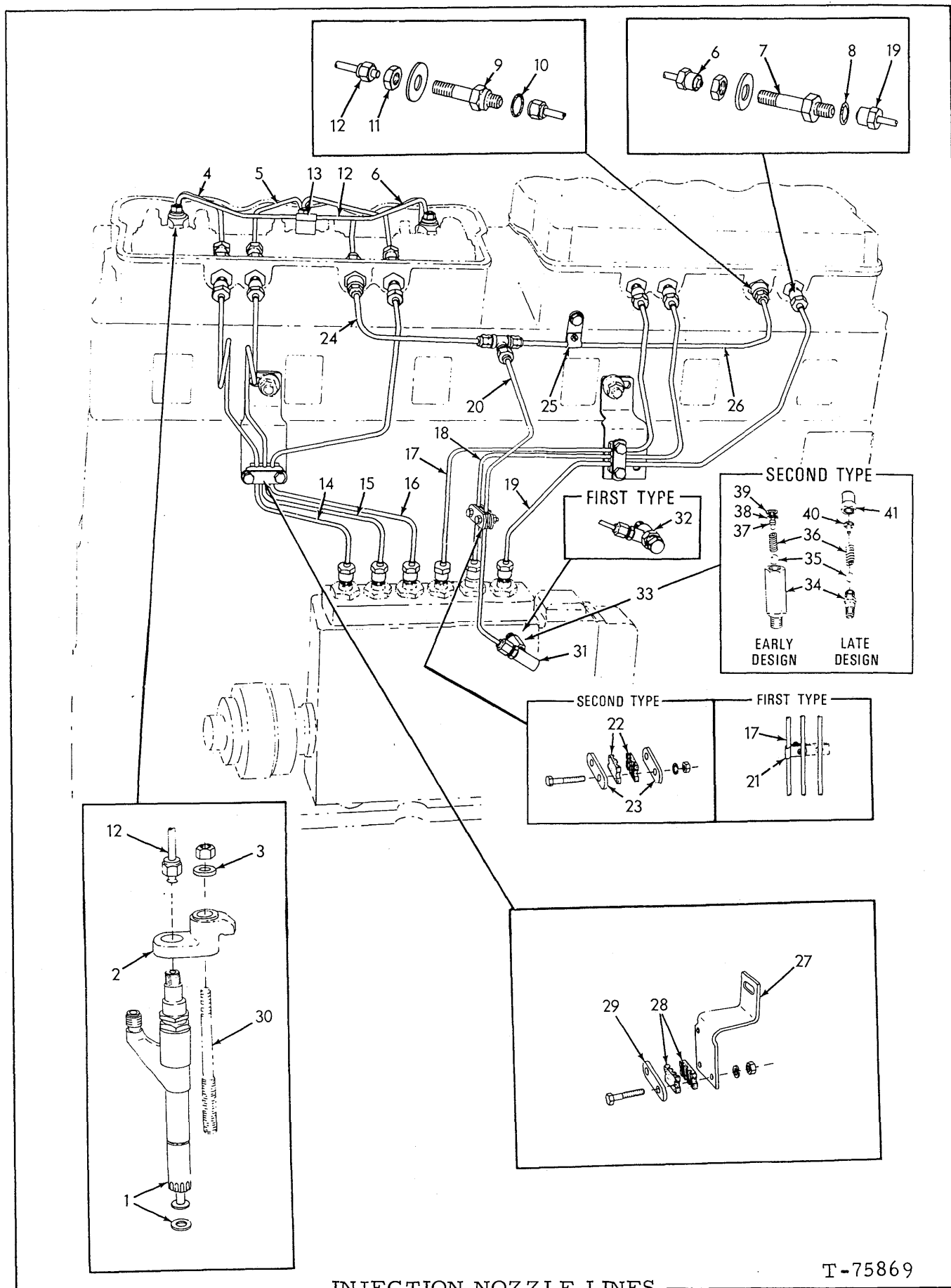
INJECTION NOZZLE LINES (Robert Bosch-Germany)
