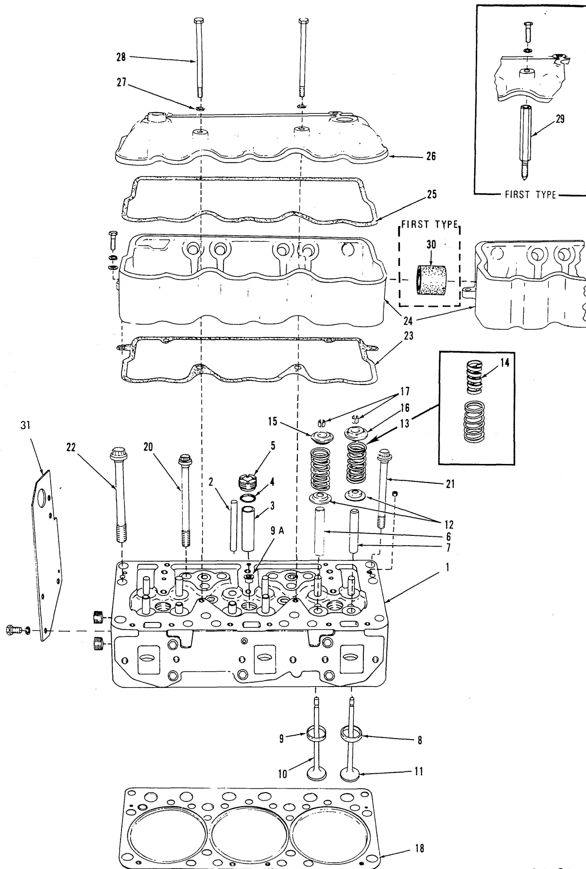
CYLINDER HEAD
