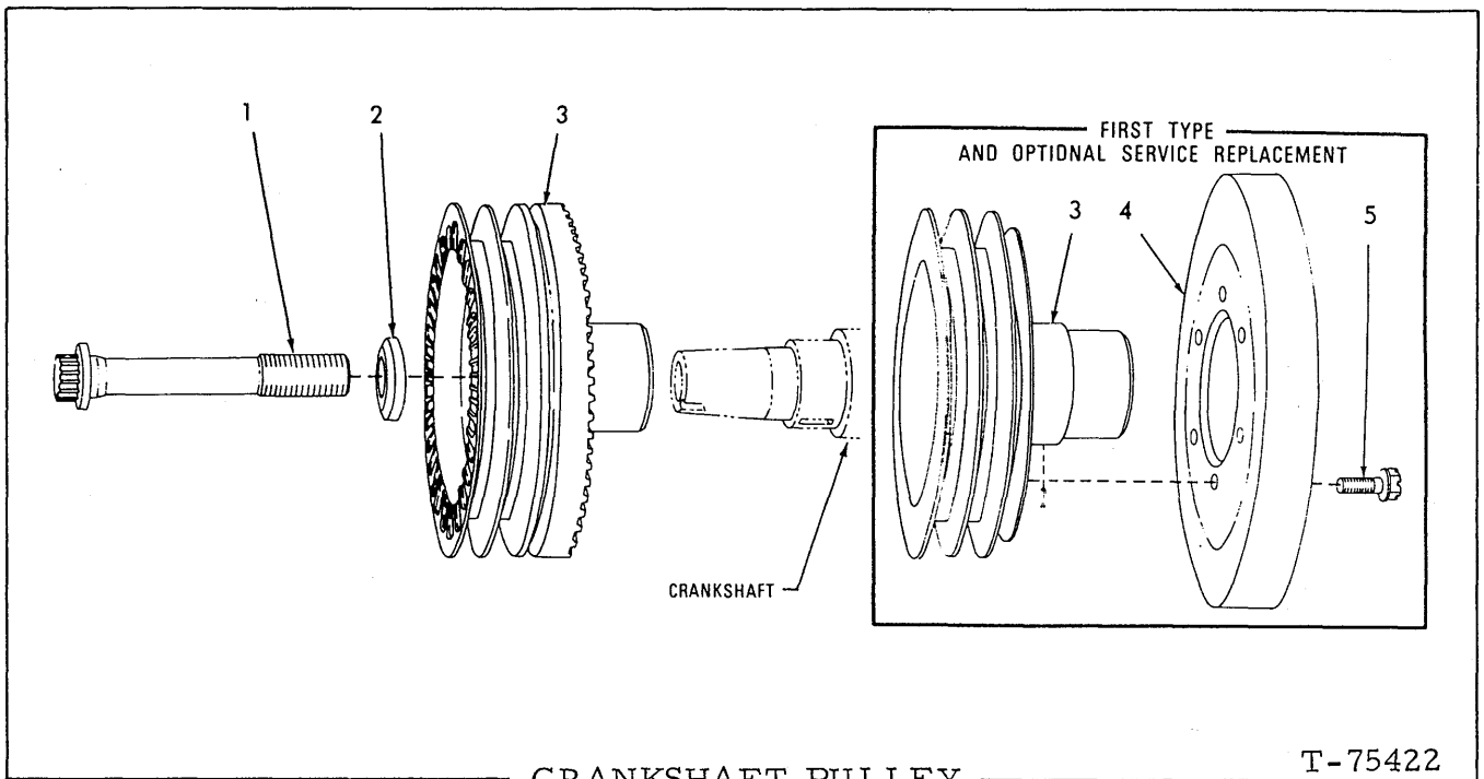
CRANKSHAFT PULLEY
