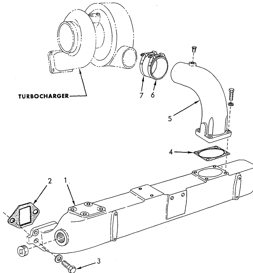
INTAKE MANIFOLD
