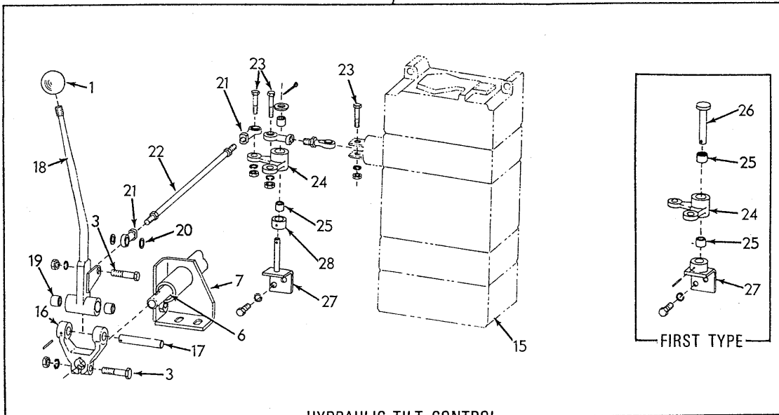
HYDRAULIC TILT CONTROL
