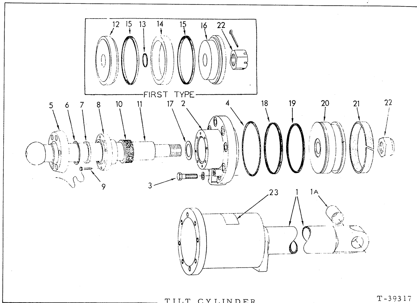
TILT CYLINDER
