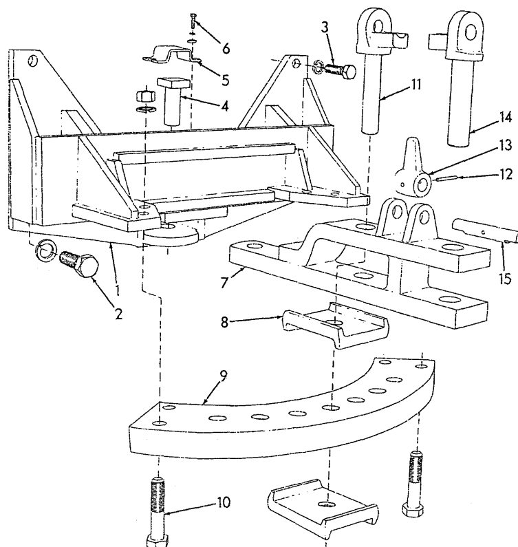
SWINGING DRAWBAR
