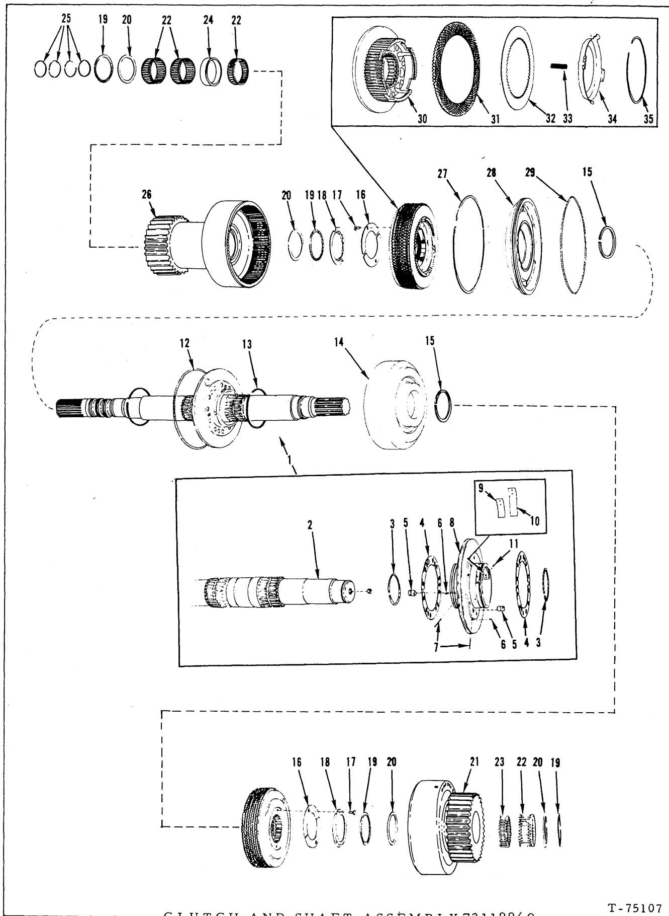
CLUTCH AND SHAFT ASSEMBLY 73118869
