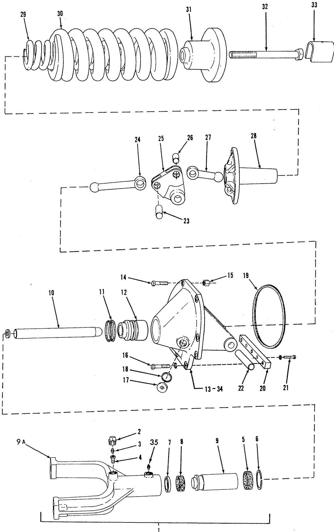
TRACK RELEASE
