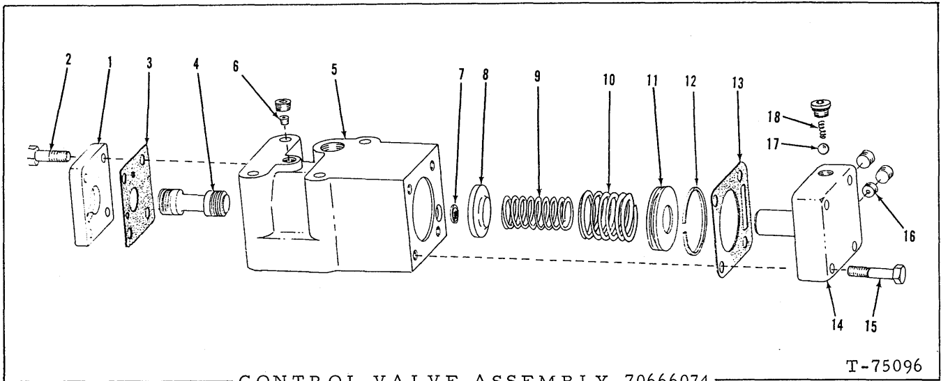
CONTROL VALVE ASSEMBLY 70666074
