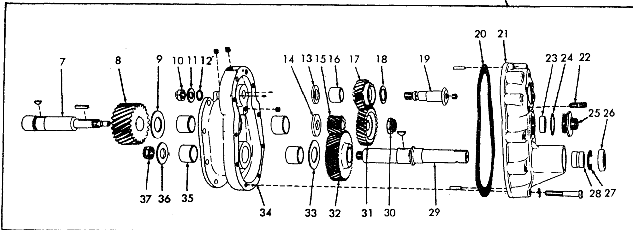
ACCESSORY DRIVE
