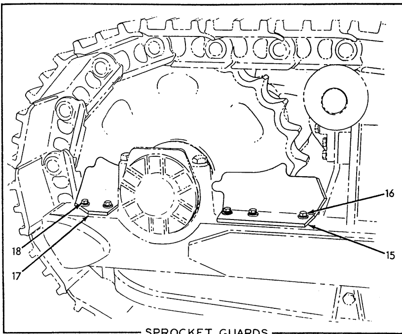
SPROCKET GUARDS
