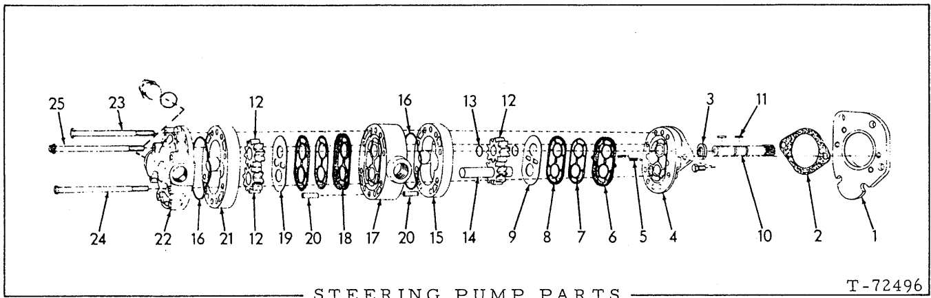
STEERING PUMP PARTS
