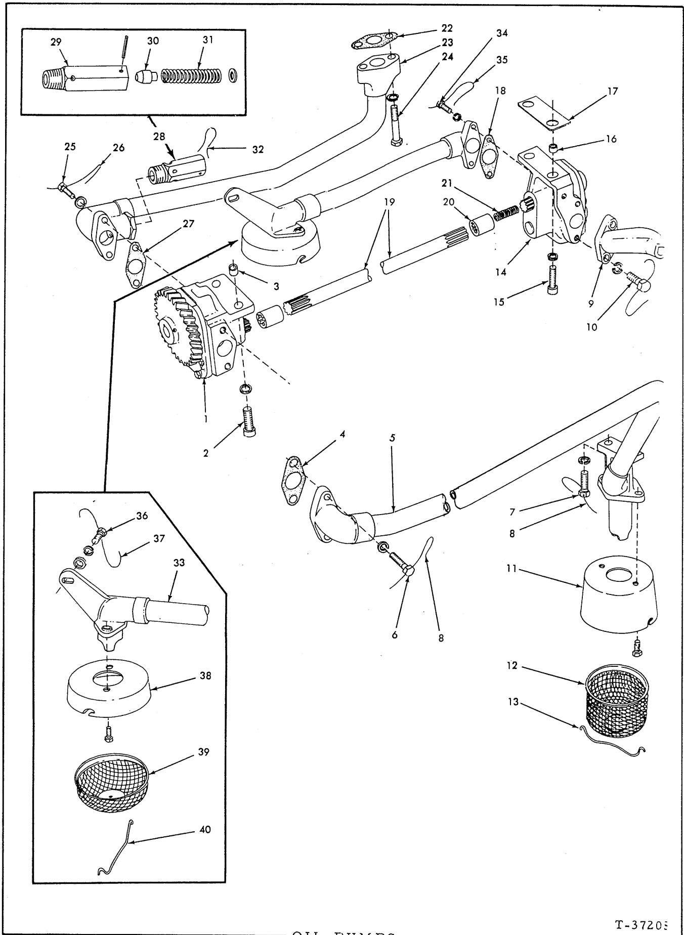
OIL PUMPS
