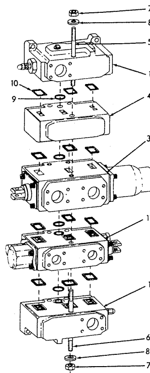
VALVE ASSY 70665122
