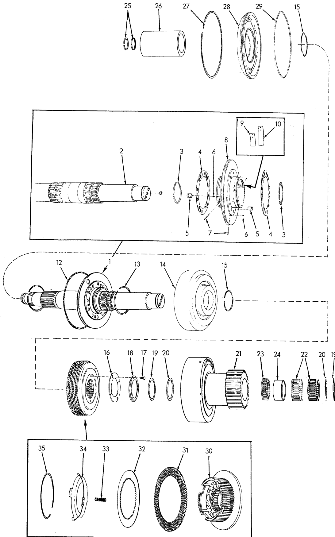
CLUTCH AND SHAFT ASSEMBLY 73118867
