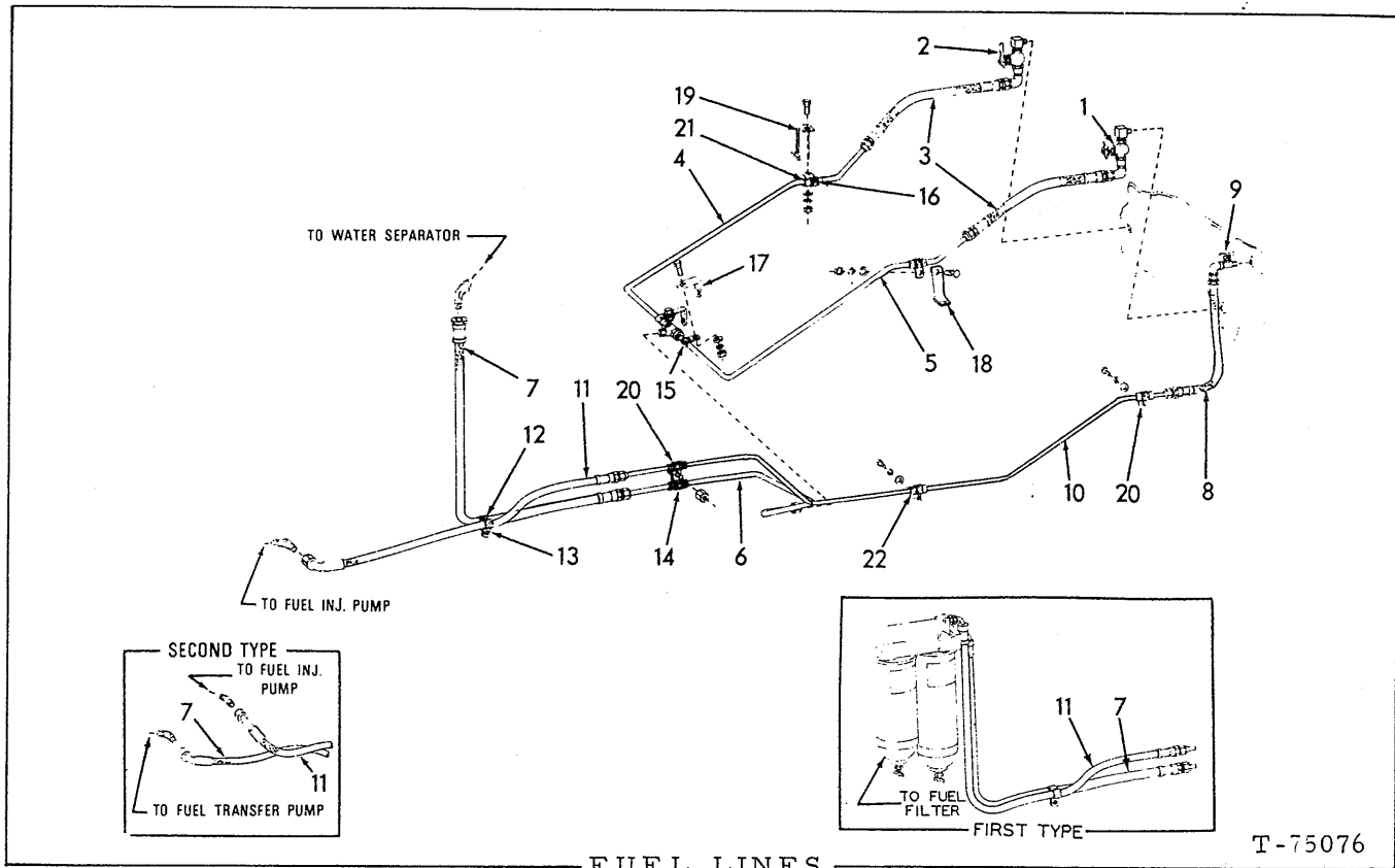
FUEL LINES
