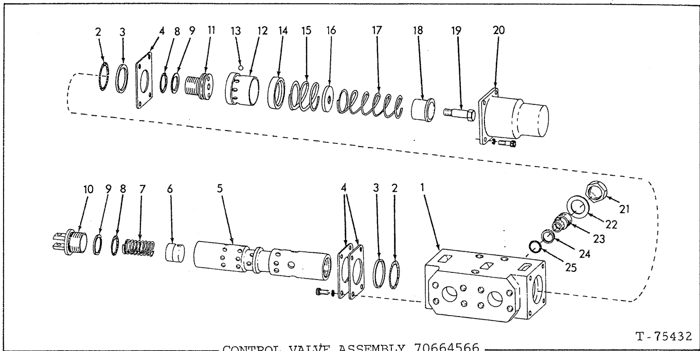
CONTROL VALVE ASSEMBLY 70664566
