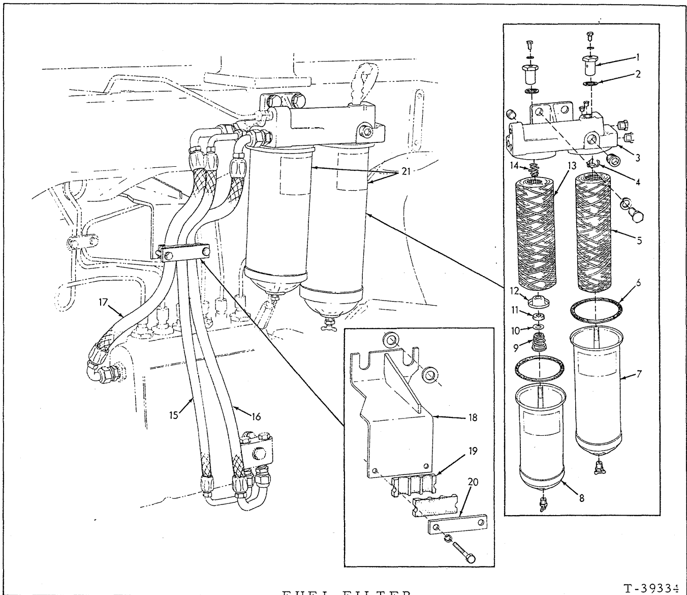
FUEL FILTER
