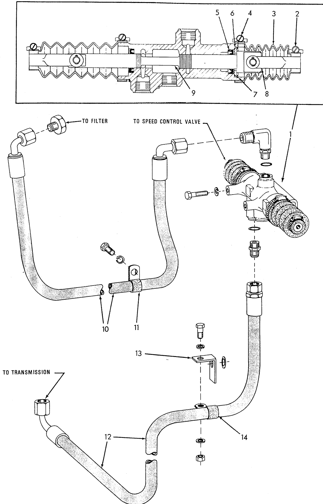
AUTOMATIC SAFETY BRAKE VALVE AND LINES
