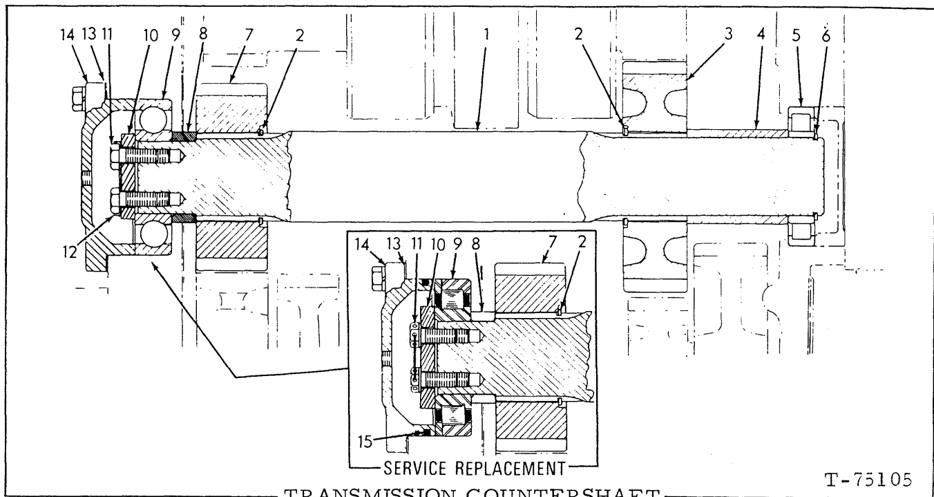
TRANSMISSION COUNTERSHAFT
