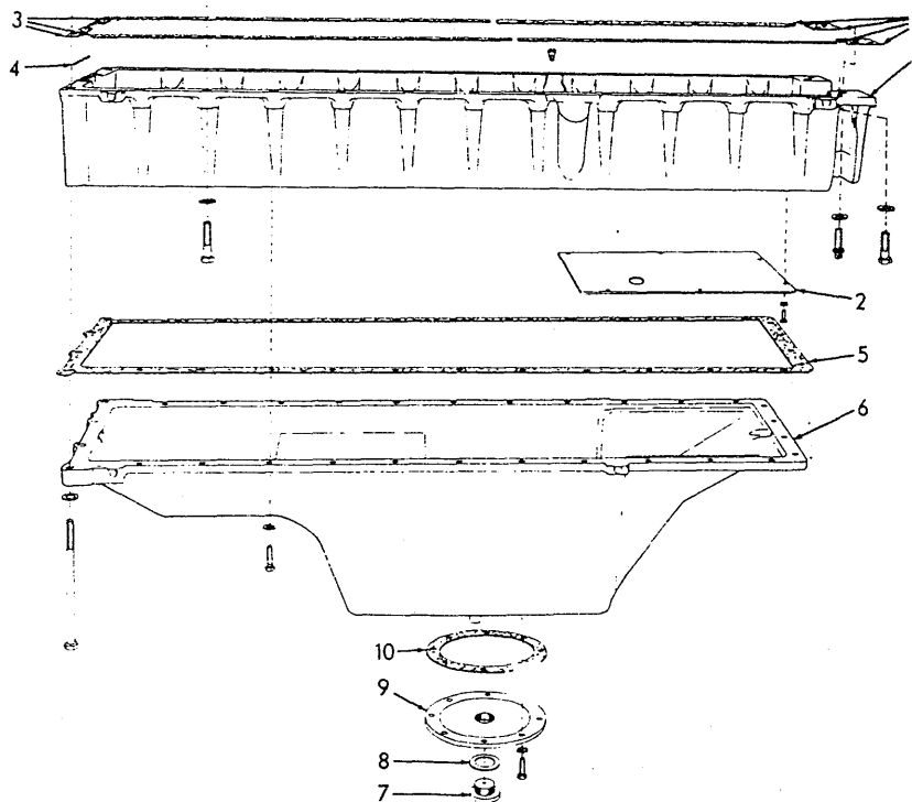
OIL PAN
