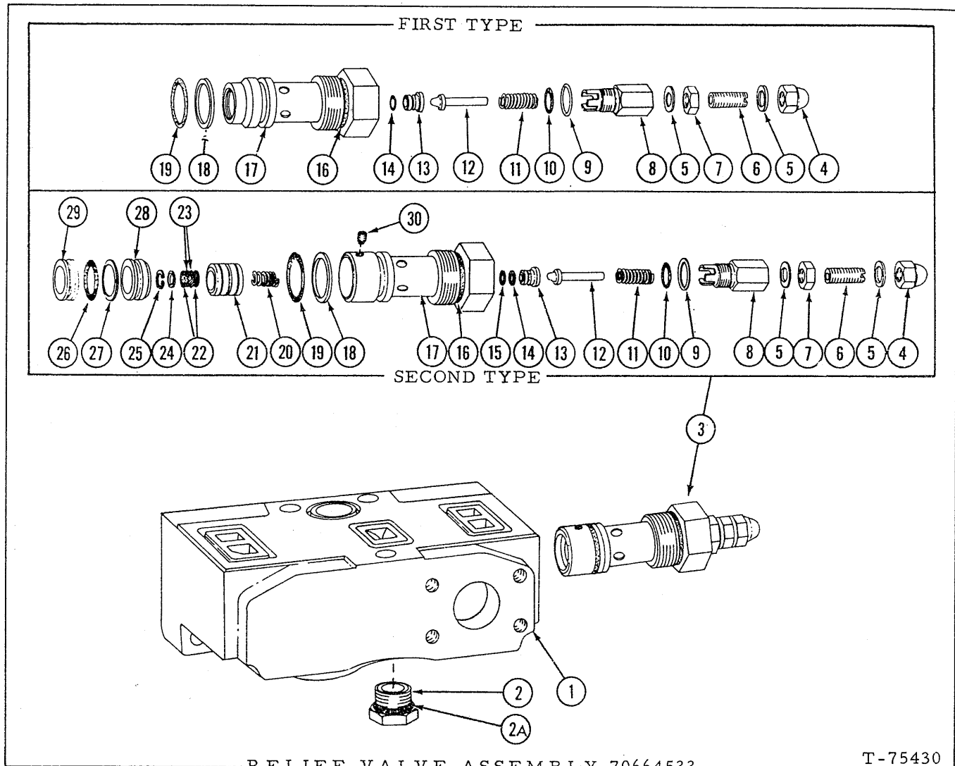
RELIEF VALVE ASSEMBLY 70664533
