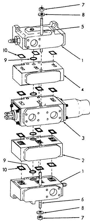
VALVE ASSY 70660647
