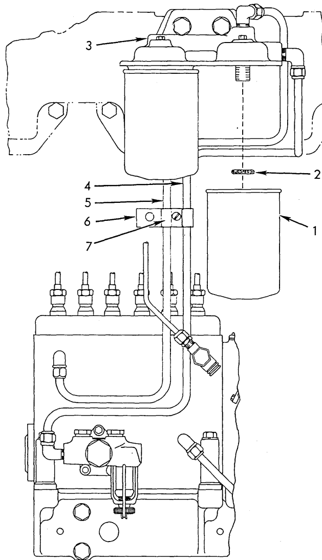
FUEL FILTER
