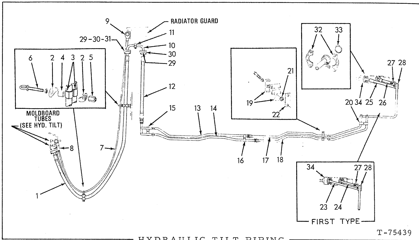
HYDRAULIC TILT PIPING
