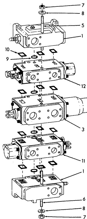
VALVE ASSY 70662085
