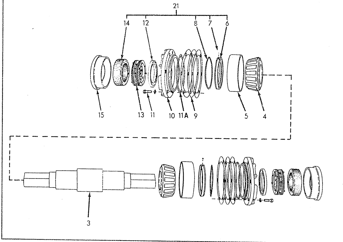
TRACK ROLLERS (First type)
