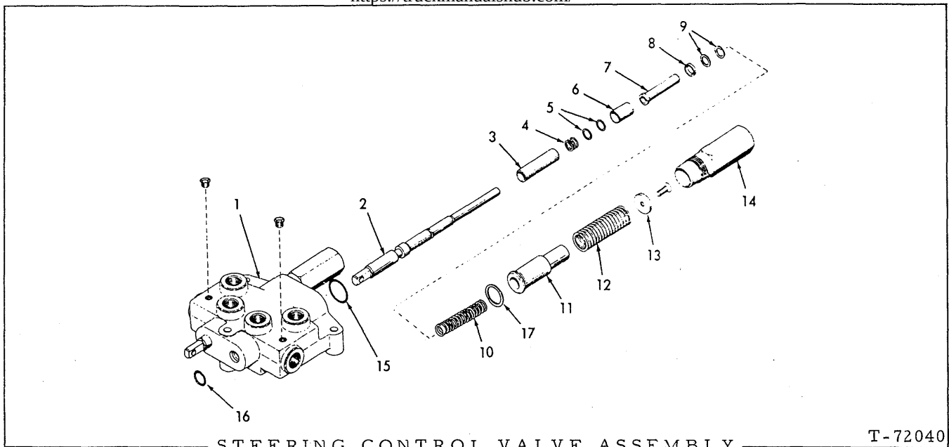
STEERING CONTROL VALVE ASSEMBLY
