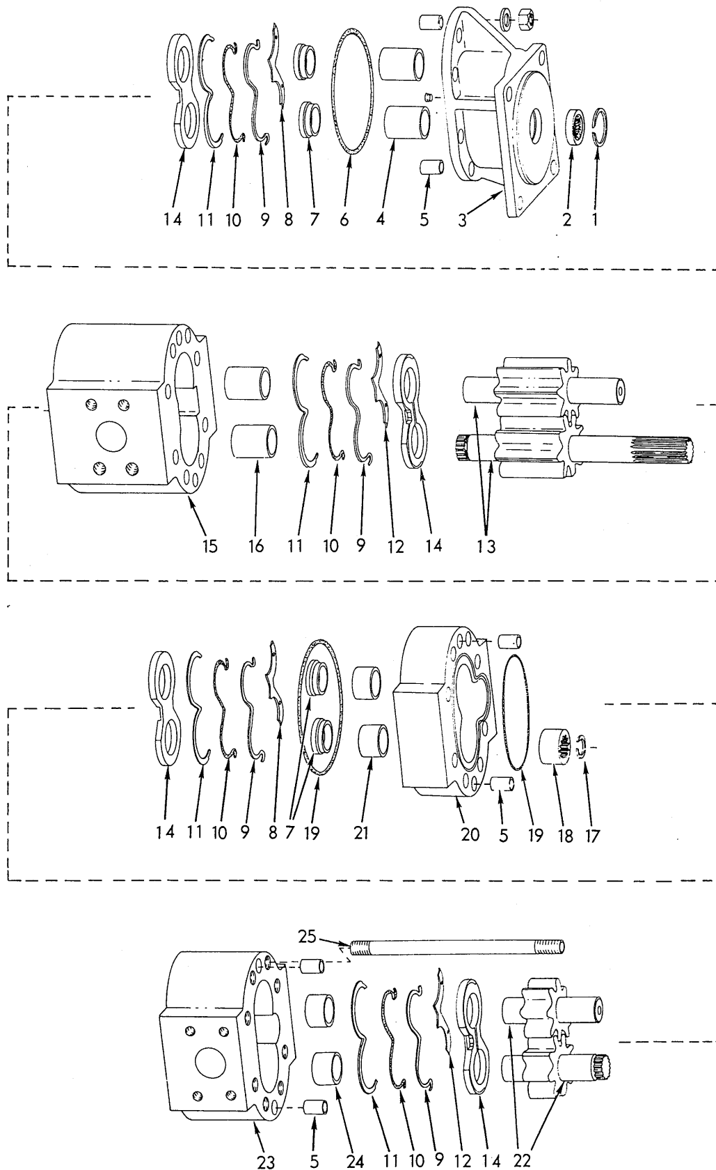
PUMP PARTS
