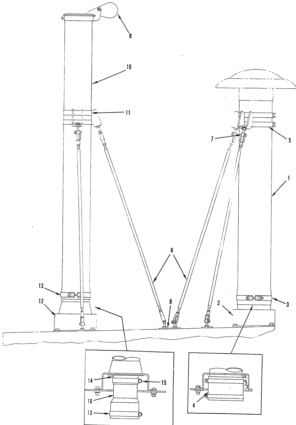
AIR INTAKE AND EXHAUST EXTENSIONS
