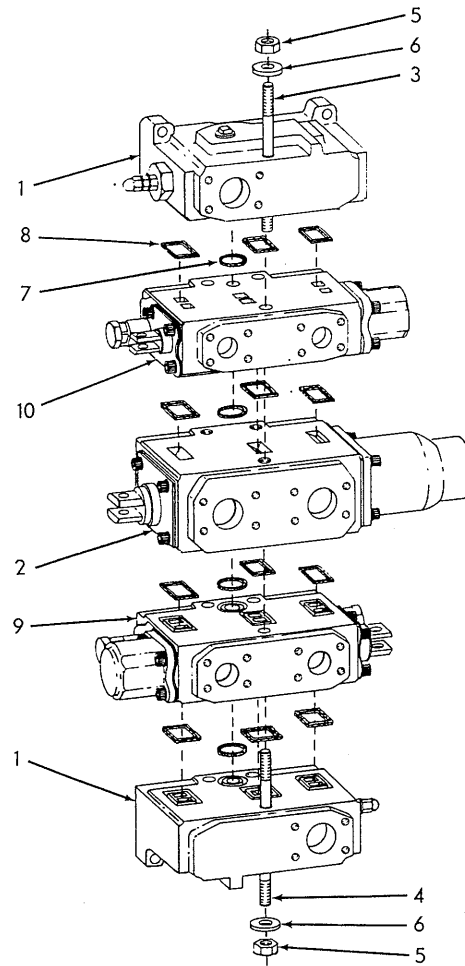
VALVE ASSY. 70686070
