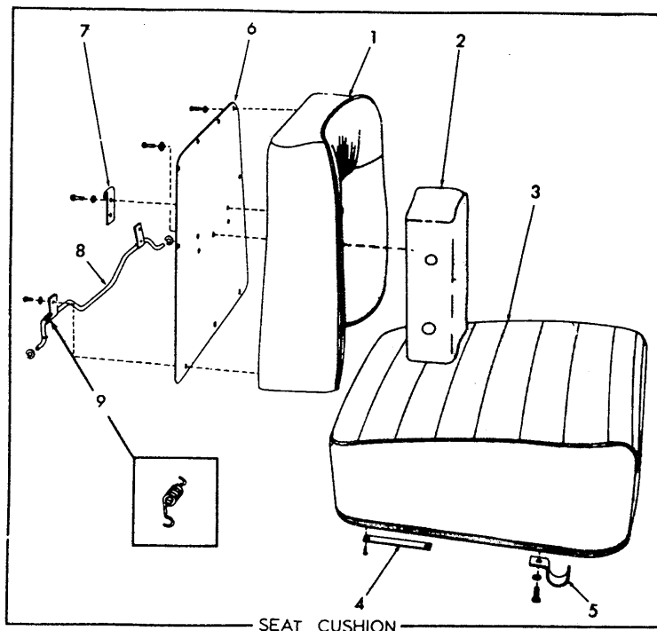
SEAT ASSEMBLY
