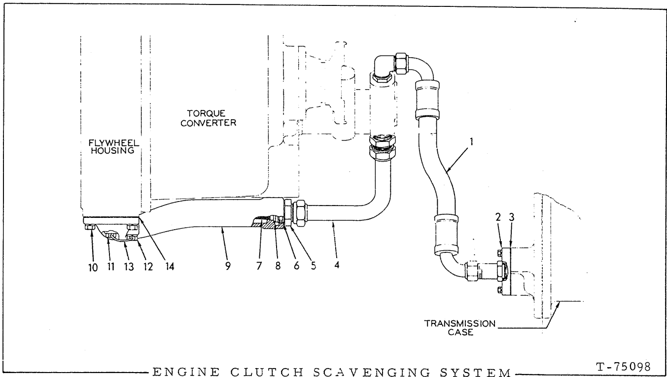
ENGINE CLUTCH SCAVENGING SYSTEM
