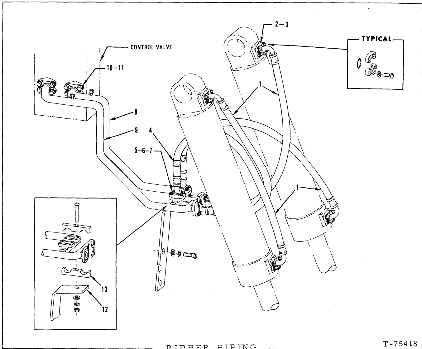
RIPPER PIPING
