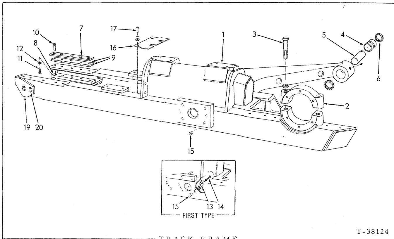
TRACK FRAME
