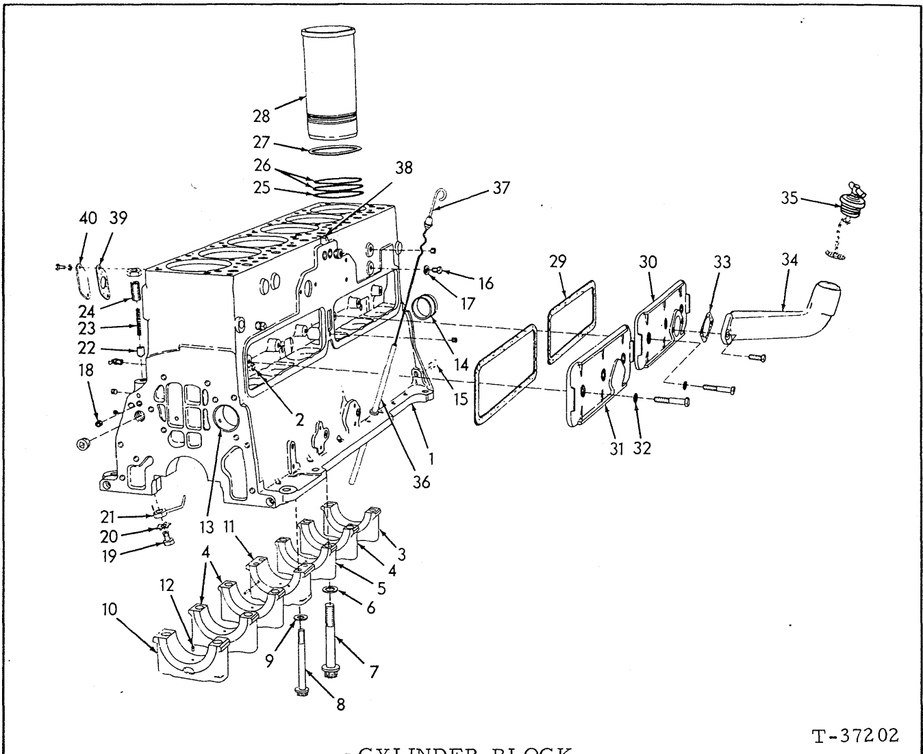
CYLINDER BLOCK
