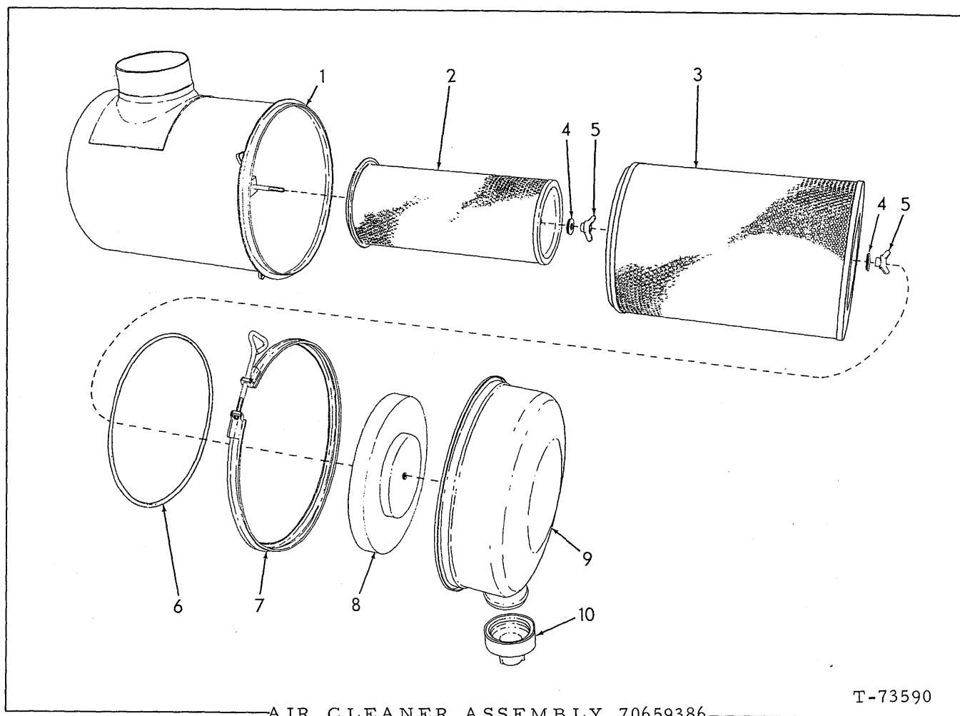
AIR CLEANER ASSEMBLY 70659386
