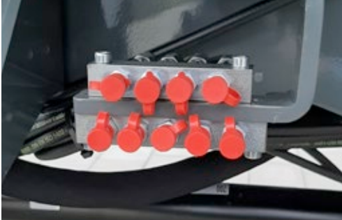
Central lubrication strip (option)
