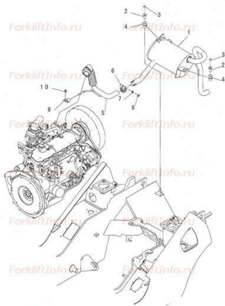
FIG. B4110-01A4 MUFFLER AND EXHAUST CONNECTION
