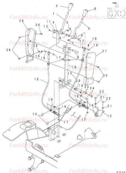
FIG. L4140-01A0 TRANSMISSION SHIFT LEVER (A-TYPE)
