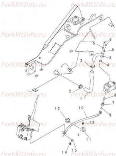
FIG. R4220-01A0 HYDRAULIC PIPING (TANK TO CONTROL VALVE)
