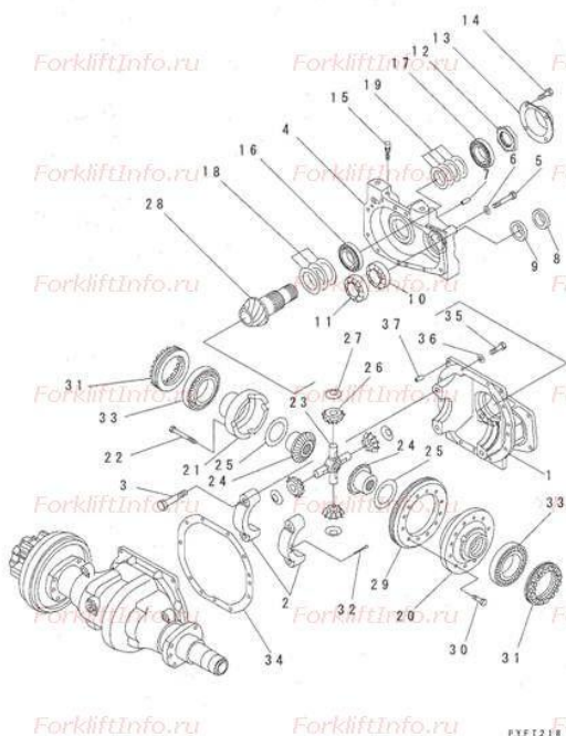
FIG. F4100-02A0 DRIVE AXLE (DIFFERENTIAL GEAR) (2/4)
