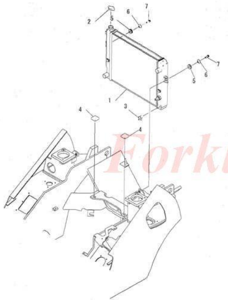
FIG. C4110-01A5 RADIATOR (TORQUE CONVERTER SPEC.)
