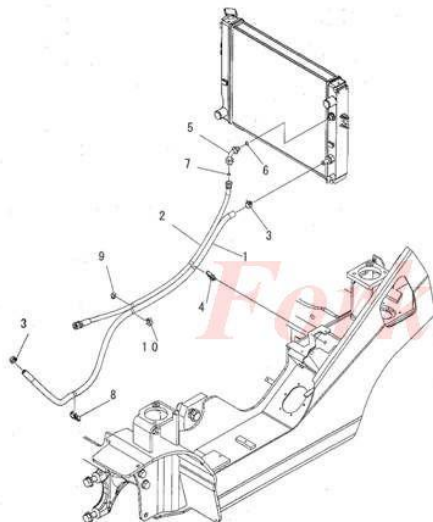
FIG. C4140-01A0 TORQUE CONVERTER COOLER PIPING
