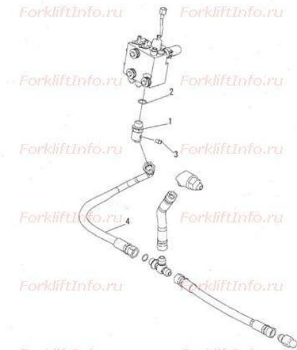
FIG. R4270-01A0 HYDRAULIC PIPING (LIFT CYLINDER LINE) (FOR FV AND FFV MAST)
