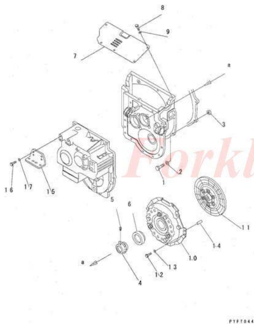
FIG. F4160-33A0 DIRECT DRIVE TRANSMISSION (3/3) (FOR DRY CLUTCH)
