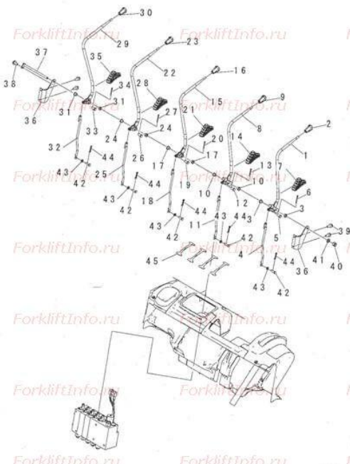
FIG. R4150-01A3 5-SPOOL CONTROL VALVE LEVER
