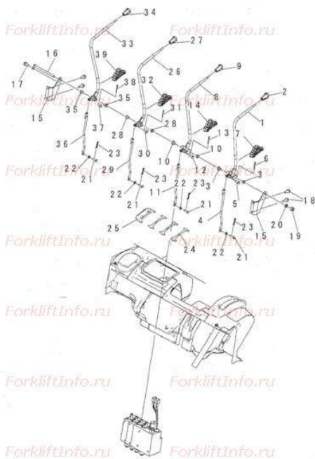
FIG. R4150-01A2 4-SPOOL CONTROL VALVE LEVER
