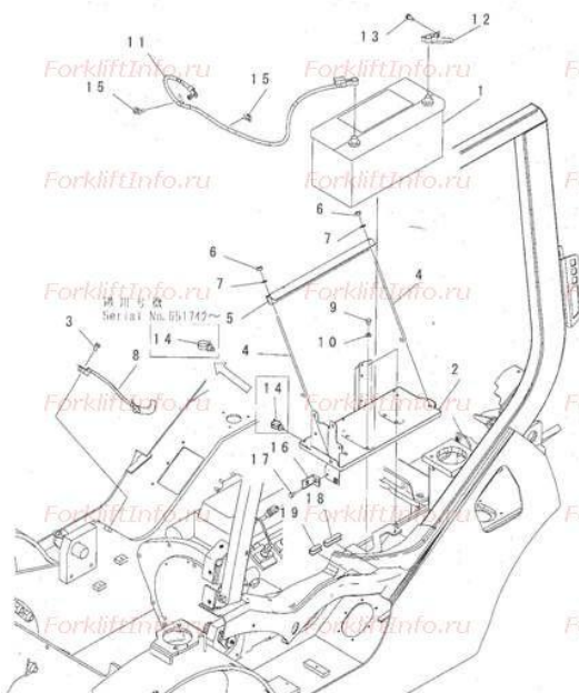
FIG. Q4130-01B0 ELECTRICAL SYSTEM (BATTERY)
