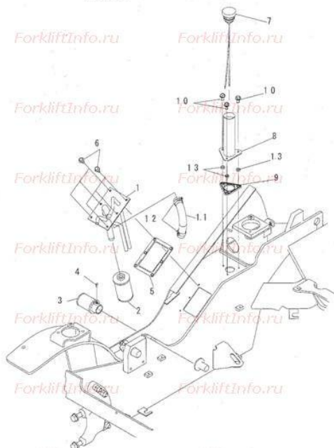
FIG. R4210-01A1 TANK COVER (DRY CLUTCH AND TORQUE CONVERTER SPEC.) (FOR FV MAST 4.0-6.0M)
