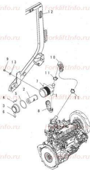
FIG. A4140-01A4 AIR INTAKE CONNECTION
