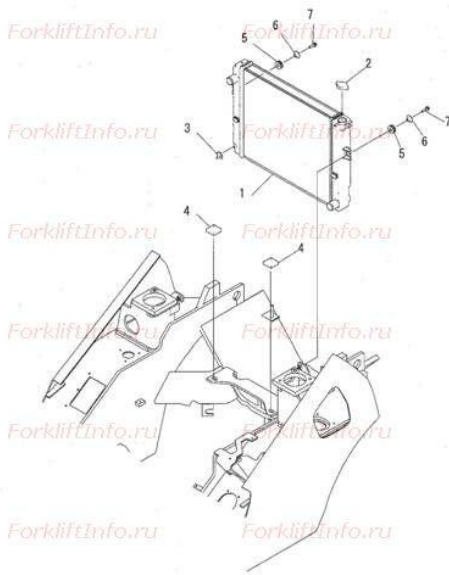
FIG. C4110-01A1 RADIATOR (TORQUE CONVERTER SPEC.)
