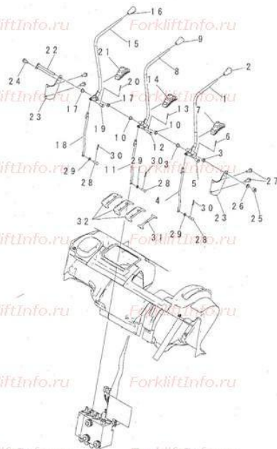
FIG. R4150-01A1 3-SPOOL CONTROL VALVE LEVER
