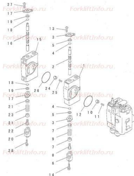
FIG. R4140-53A2 CONTROL VALVE (INNER PARTS) (3/4) (FOR 4-SPOOL CONTROL VALVE)
