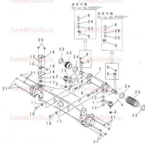
FIG. H4110-02B1 STEERING AXLE (2/2) (INCLUDE POWER STEERING CYLINDER BOOT AND STEERING SYNCHRONIZER FUNCTION)
