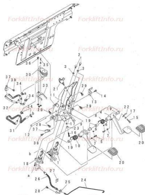
FIG. L4150-01A0 BRAKE AND CLUTCH PEDAL (DRY CLUTCH SPEC.)
