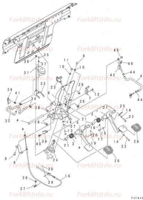
FIG. L4150-01A2B BRAKE AND INCHING PEDAL (TORQUE CONVERTER SPEC.) (#653223-)
