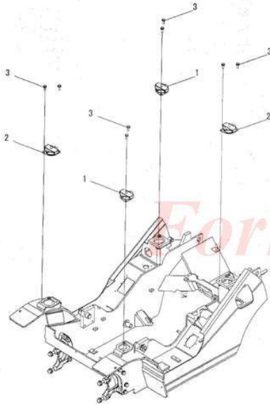
FIG. P4280-01A0 HEAD GUARD MOUNTING PARTS
