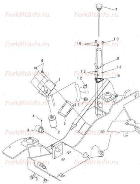
FIG. R4210-01AD TANK COVER (DRY CLUTCH AND TORQUE CONVERTER SPEC.) (FOR FV MAST 3.0-3.7M AND TFV/FFV MAST)
