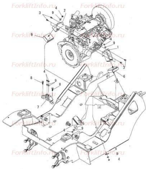
FIG. A4120-01A4 ENGINE MOUNTING PARTS
