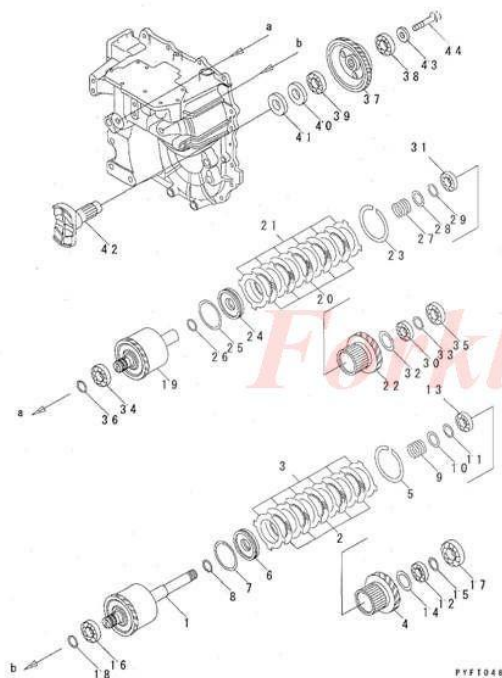
FIG. F4160-42AO TORQUE FLOW DRIVE TRANSMISSION (2/6)
