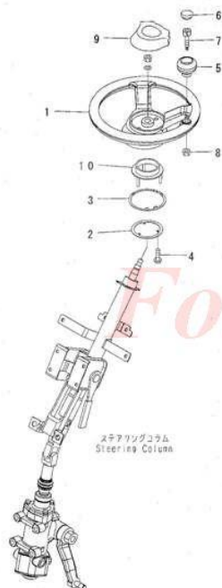
FIG. L4120-01A0 STEERING WHEEL
