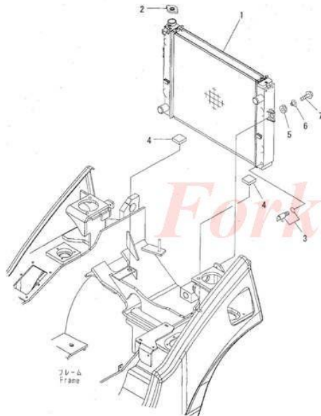
FIG. C4110-01A4 RADIATOR (DRY CLUTCH SPEC.)
