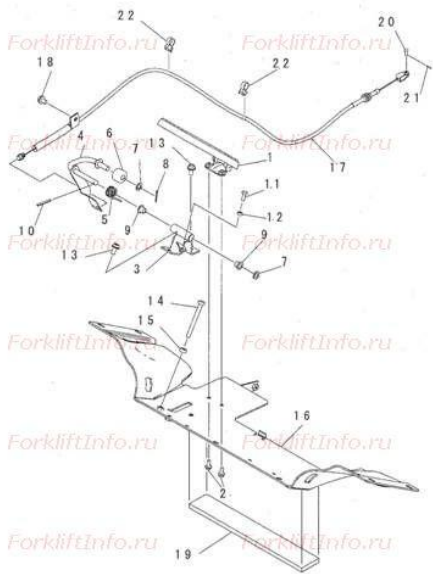
FIG. L4160-01A0 ACCELERATOR PEDAL
