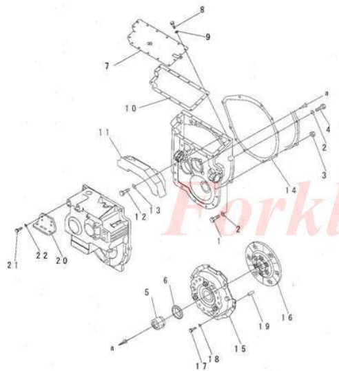
FIG. F4160-33A1 DIRECT DRIVE TRANSMISSION (3/3) (FOR WET CLUTCH)
