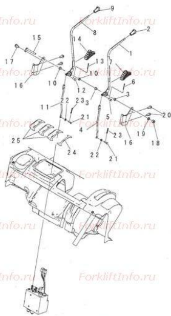
FIG. R4150-01A0 2-SPOOL CONTROL VALVE LEVER
