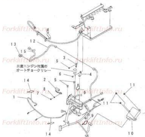
FIG. 04210-01B6A ELECTRICAL SYSTEM (ENGINE WIRING) (STEERING SYNCHRONIZER FUNCTION AND OPS) (#651742-)
