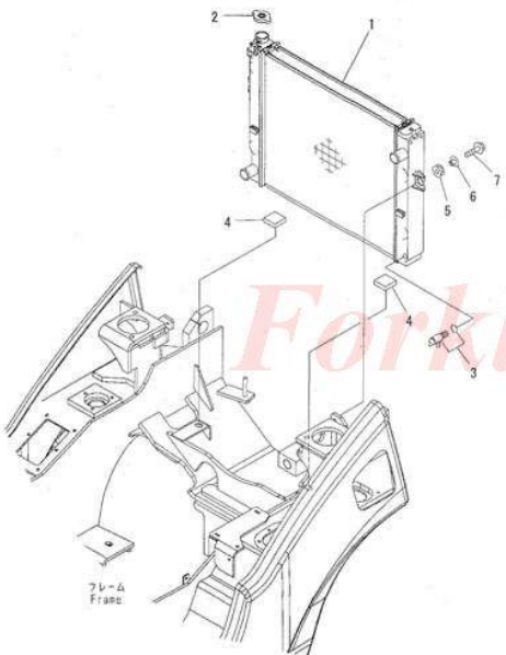
FIG. C4110-01A7 RADIATOR (DRY CLUTCH SPEC.)
