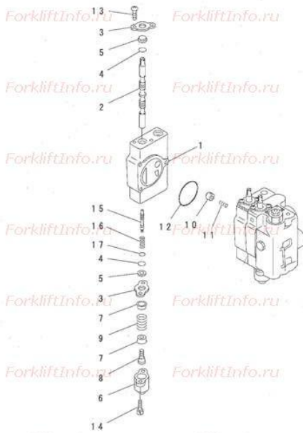
FIG. R4140-52A0 CONTROL VALVE (INNER PARTS) (2/4) (TILT SPOOL BLOCK)
