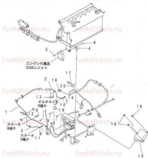
FIG. 04210-01B5A ELECTRICAL SYSTEM (ENGINE WIRING) (STEERING SYNCHRONIZER FUNCTION AND OPS) (#651742-)
