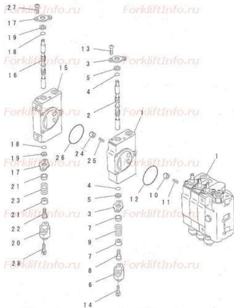
FIG. R4140-53A4 CONTROL VALVE (INNER PARTS) (3/4) (FOR 5-SPOOL CONTROL VALVE)
