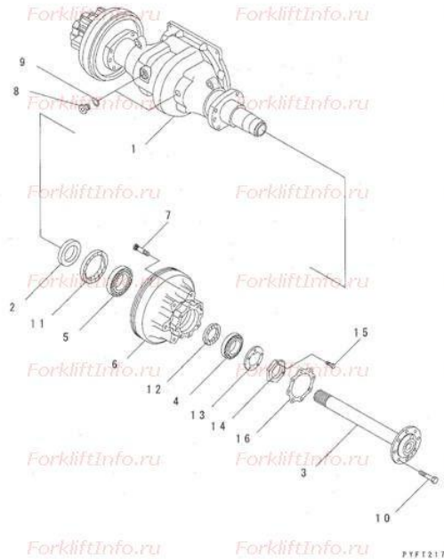
FIG. F4100-01A0 DRIVE AXLE (HOUSING AND HUB) (1/4)
