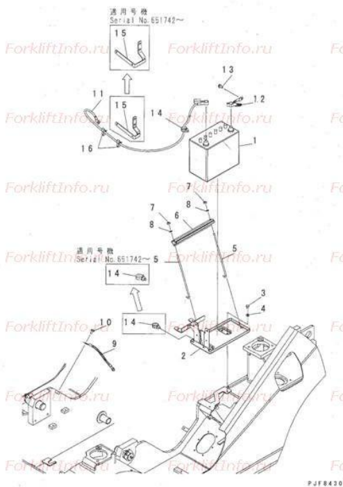
FIG. Q4130-01B1 ELECTRICAL SYSTEM (BATTERY)
