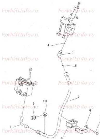
FIG. R4240-01A0 HYDRAULIC PIPING (POWER STEERING LINE) (1/2)
