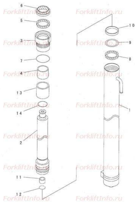
FIG. S4010-03A1 FV MAST LIFT CYLINDER (4.0-5.0M)
