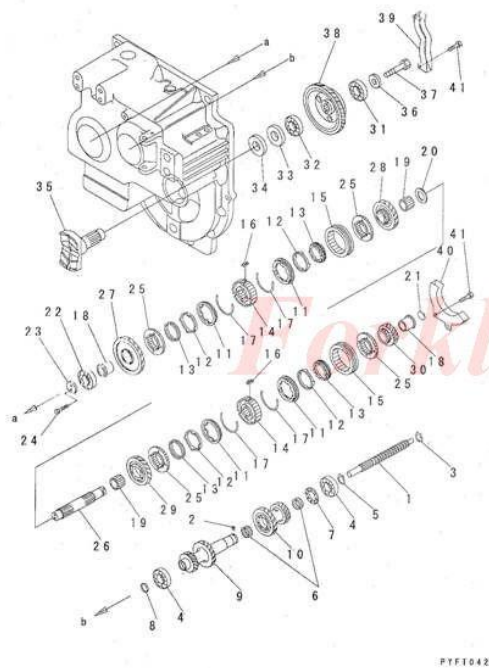
FIG. F4160-32A0 DIRECT DRIVE TRANSMISSION (2/3)
