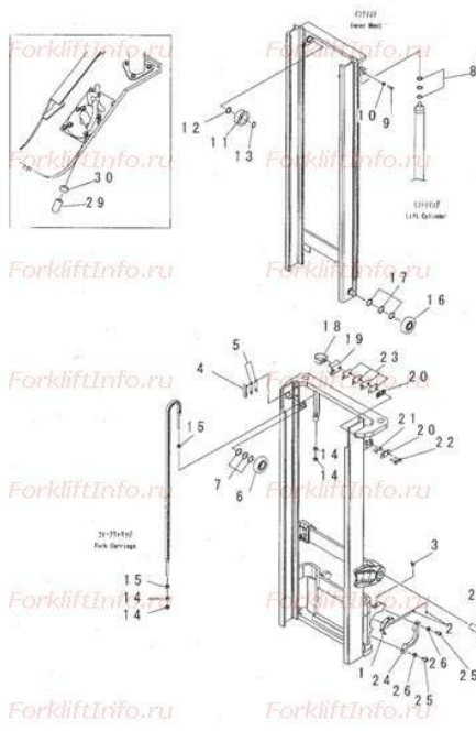
FIG. S4010-02A0 FV MAST (2/2) (MAST ATTACHING PARTS)
