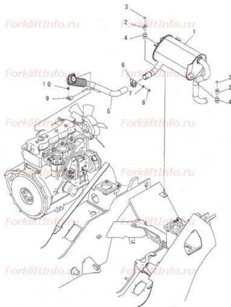
FIG. B4110-01A0 MUFFLER AND EXHAUST CONNECTION
