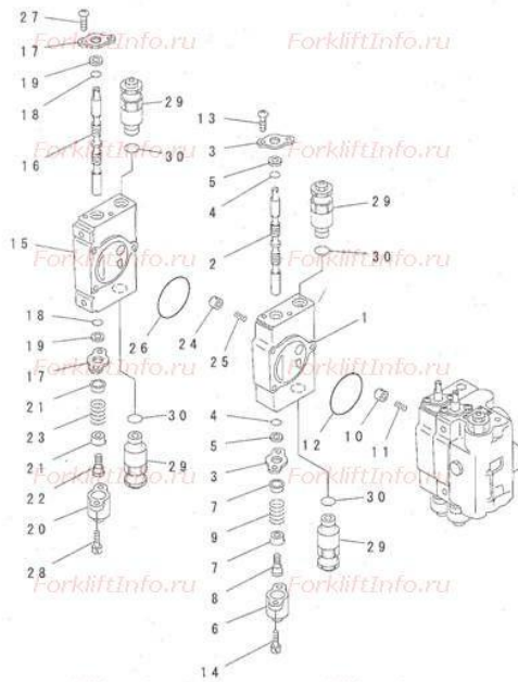
FIG. R4140-53A3 CONTROL VALVE (INNER PARTS) (3/4) (FOR 4-SPOOL CONTROL VALVE) (WITH PORT RELIEF VALVE)
