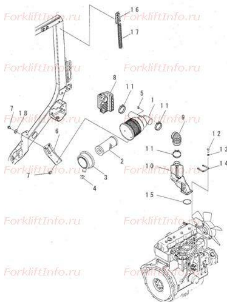
FIG. A4140-01A0 AIR INTAKE CONNECTION
