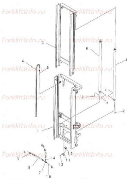
FIG. S4010-01A0 FV MAST (1/2) (MAST AND LIFT CYLINDER)
