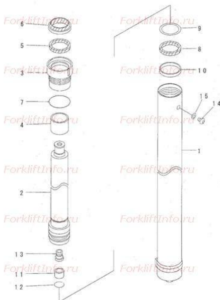
FIG. S4010-03A0 FV MAST LIFT CYLINDER (3.0-3.7M)
