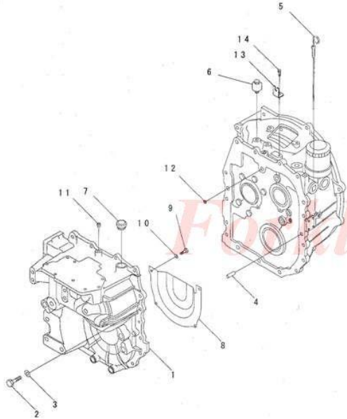
FIG. F4160-41A0 TORQUE FLOW DRIVE TRANSMISSION (1/6)
