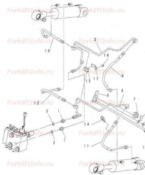
FIG. R4230-01A0 HYDRAULIC PIPING (TILT CYLINDER LINE)
