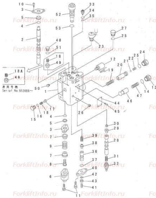
FIG. R4140-51A0 CONTROL VALVE (INNER PARTS) (1/4) (LIFT SPOOL BLOCK)
