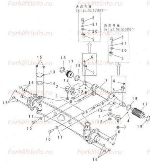
FIG. H4110-02B0 STEERING AXLE (2/2) (INCLUDE POWER STEERING CYLINDER BOOT SPEC.)
