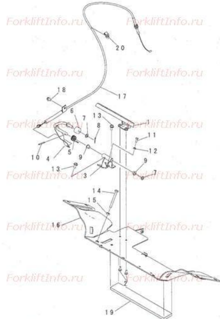
FIG. L4160-01A2 ACCELERATOR PEDAL
