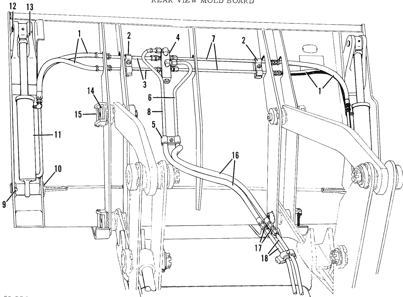
REAR VIEW MOLD BOARD
