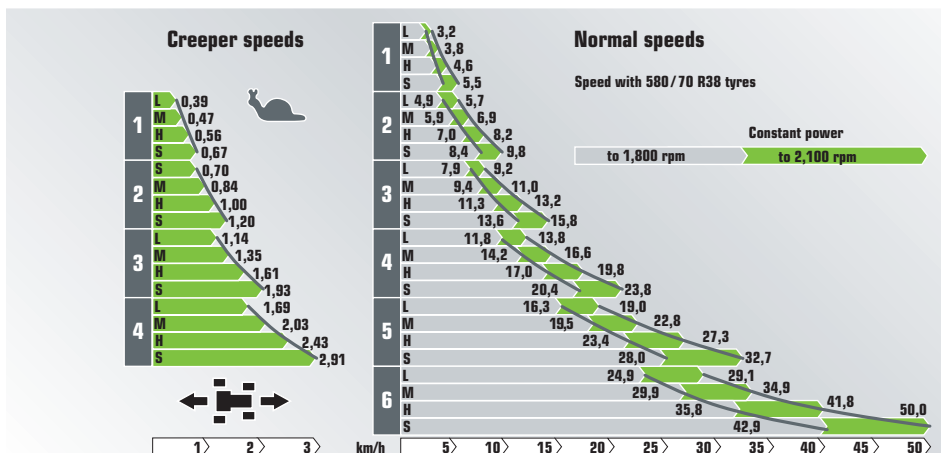
Economical in each speed: Additional Powershift stages are unnecessary due to the perfect coordination of engine and transmission. The driver can drive without constant shifting and still save fuel.
