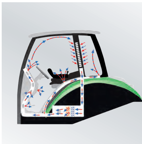
A total of 14 adjustable air nozzles ensure quick demisting and a pleasant atmosphere in the cab.
