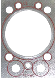
5316 HEAD GASKET ZETOR (1.5/110/9 HOLE)
