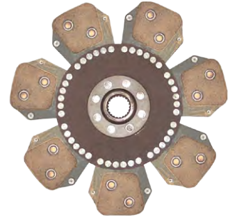
4788 14" 7 PADDLE DISC
