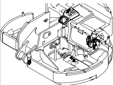
Fig. 16 電装品 (機器) ELECTRIC PART (EQUIPMENT)
