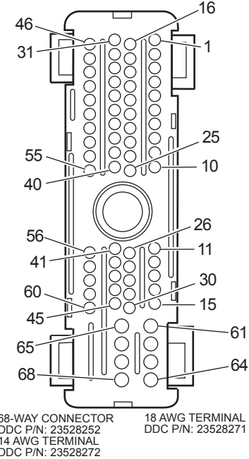
SHROUD SIDE OF CONNECTOR
