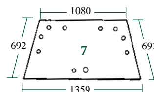
21/4047-46 (D7712, 04314333) Arrière haut, 10 trous Upper rear, 10 holes DX.85, 90, 110, 120, 140, 145, 160
