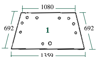
21/4000-65 (D7712, 04307803) Pare-brise ouvrant 10 trous, Ep.: 6 mm Windscreen opening 10 holes, Thick.: 6mm
