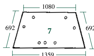
21/4072-47 (D7710, 04346800) Arrière haut, 7 trous Upper rear, 7 holes (DX.80, 86, 92, DX.85 (S/N 7816/0001 & 7817/0001 ☺), DX.90 (S/N 7818/0001 & 7819/0001 ☺), DX.110 (S/N 7820/0001 & 7821/0001 ☺), DX.120 (S/N 7826/0001 & 7827/0001 ☺))
